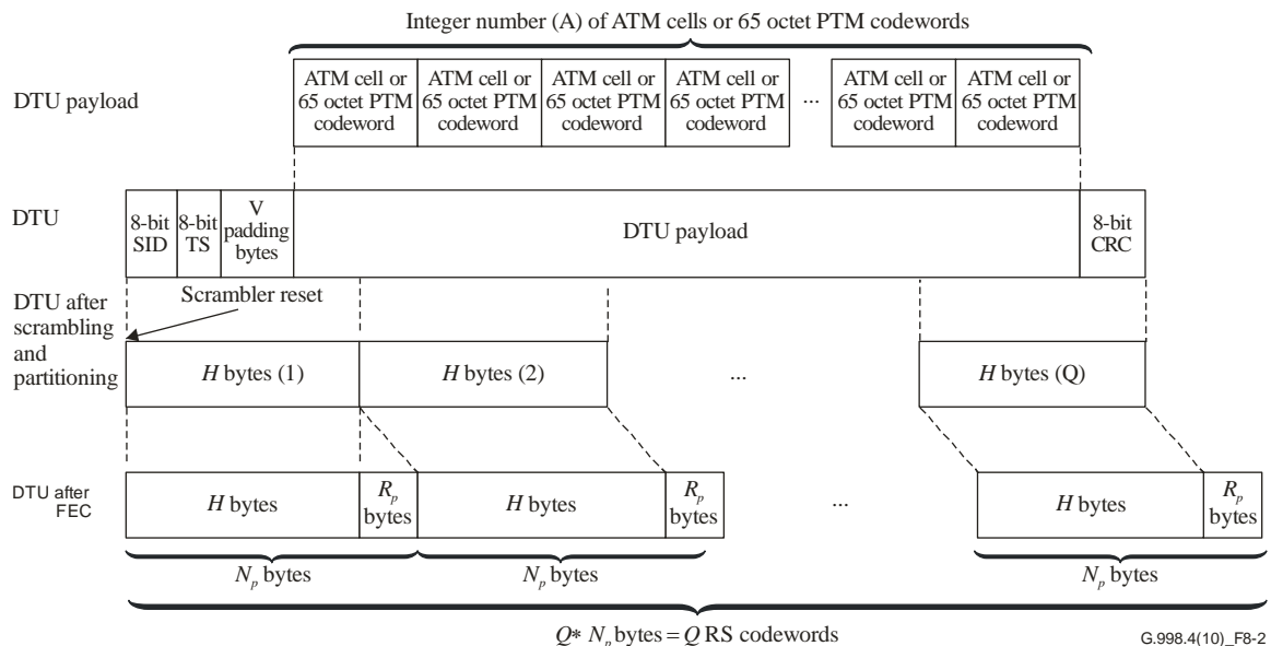
Figure 8-2 – Structure of DTU with CRC at the tail (Framing type 2) and synchronization with RS codewords
