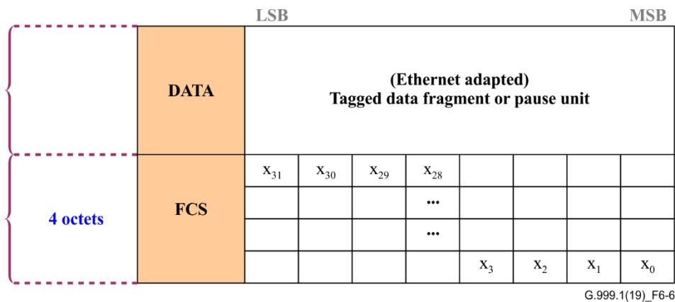
Figure 6-6 – Addition of FCS
