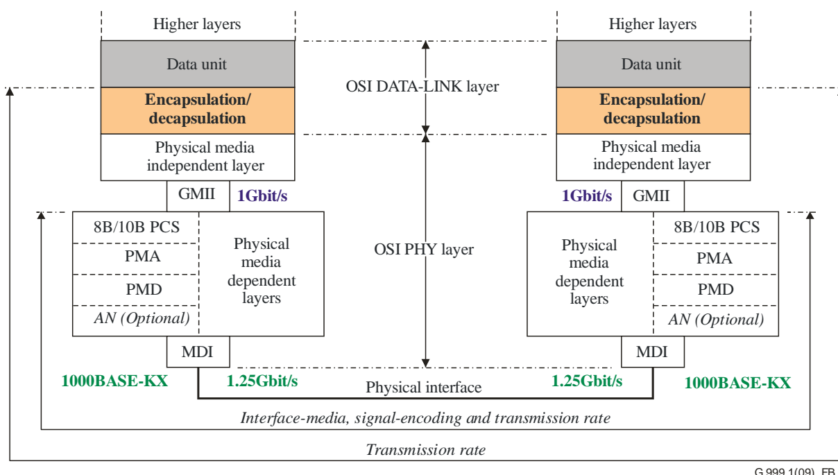
Figure B.1 – LINK/PHY interface based on 1000BASE-KX
