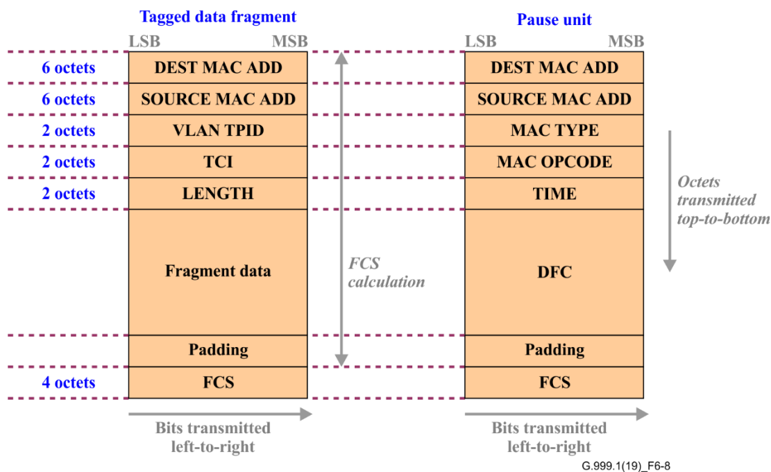
Figure 6-8 – Final encapsulation format with Ethernet encapsulation
