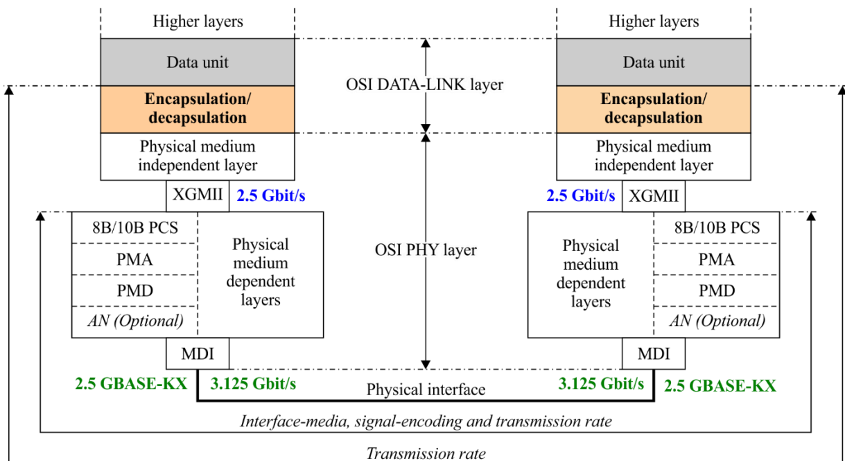
Figure C.1 – LINK/PHY interface based on 2.5GBASE-KX
