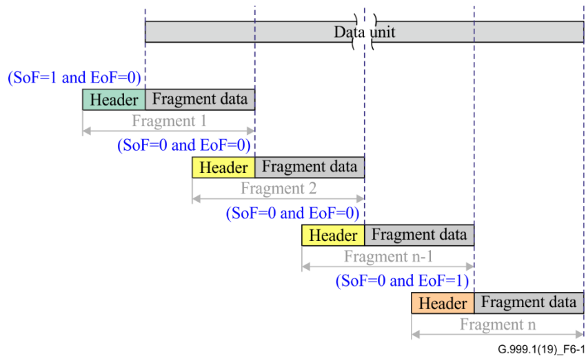
Figure 6-1 – Data unit fragmentation
