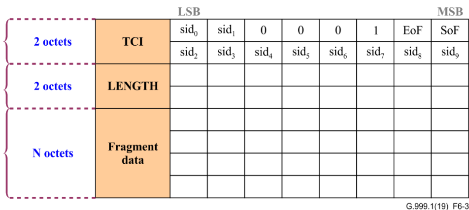
Figure 6-3 – Tagged fragment format
