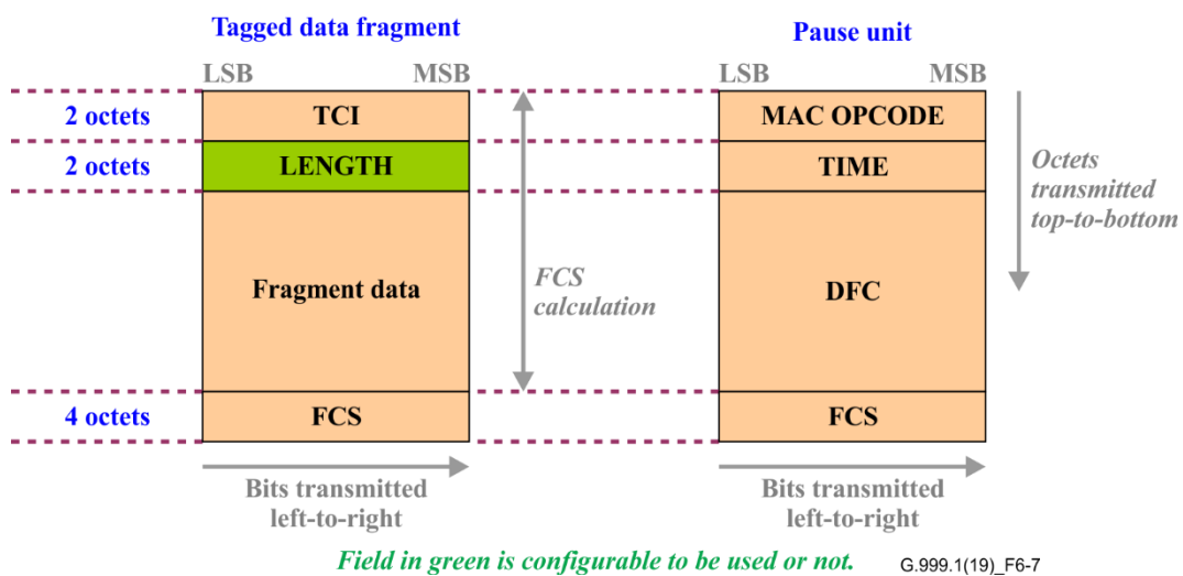
Figure 6-7 – Final encapsulation format without Ethernet encapsulation
