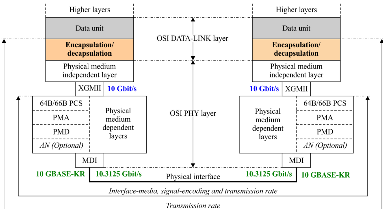
Figure D.1 – LINK/PHY interface based on 10GBASE-KR
