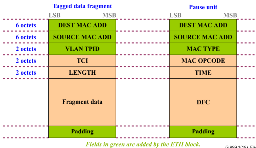
Figure 6-5 – Ethernet adapted format
