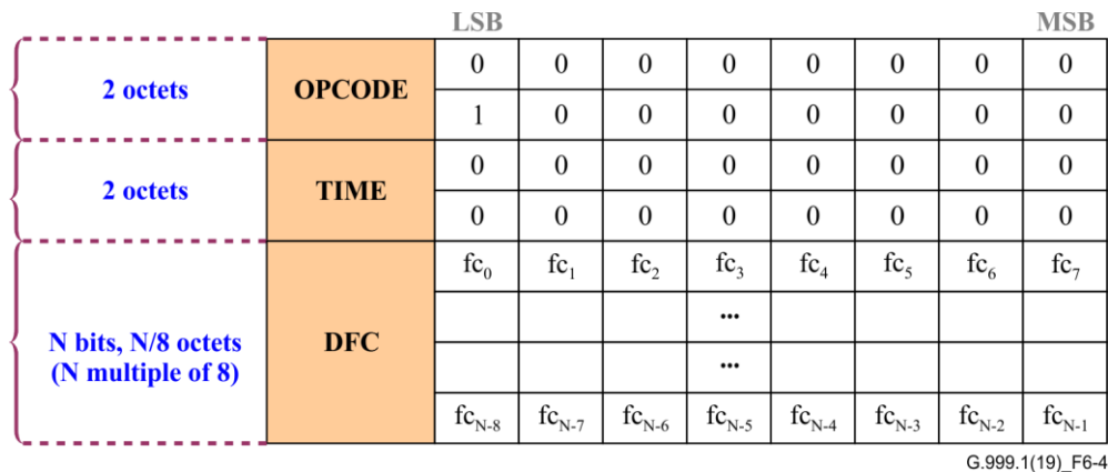
Figure 6-4 – Pause unit format
