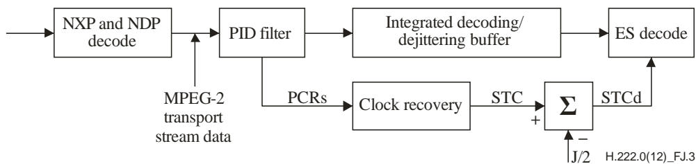
Figure J.3 – Integrated dejittering and MPEG-2 decoding
