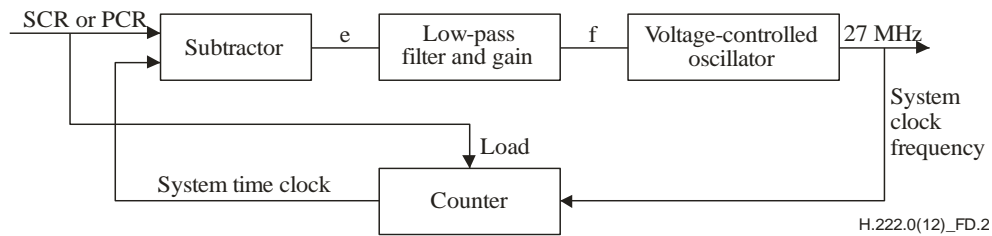
Figure D.2 – STC recovery using PLL
