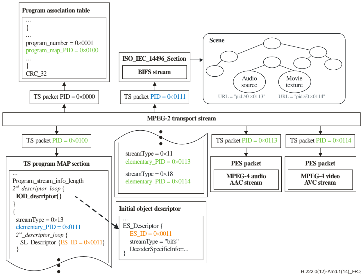
Figure R.3 – Usage of MPEG-4 in a transport stream with BIFS scene referring to native PES
