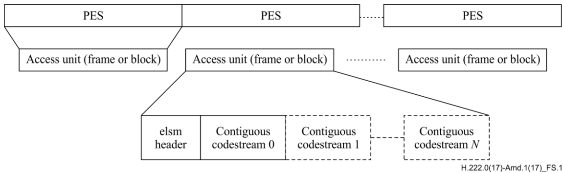
Figure S.1 – Structure and order of JPEG 2000 access units
