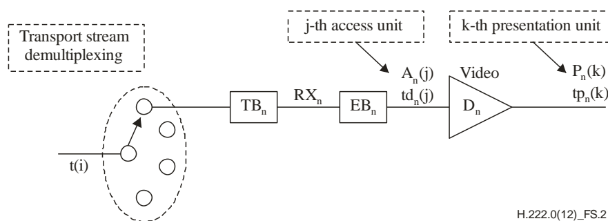
Figure S.2 – T-STD model extensions for J2K Video
