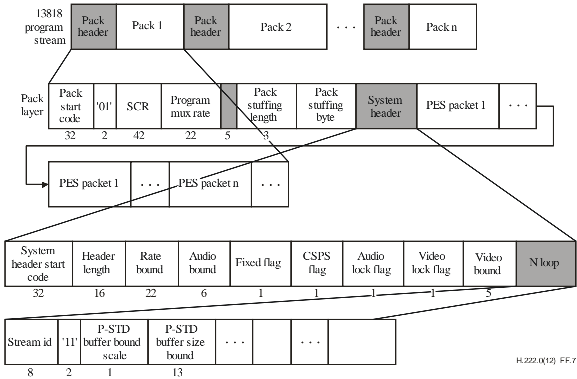
Figure F.7 – Program stream diagram
