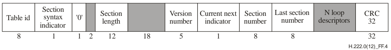
Figure F.4 – Conditional access section diagram
