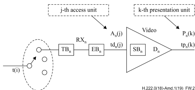
Figure W.2 – T-STD model extensions for JPEG XS Video
