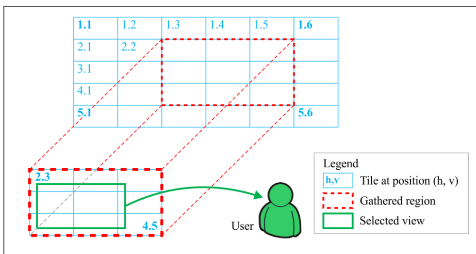
Figure V.1 – Illustration of HEVC tiled encoding of panoramic content beyond UHD
