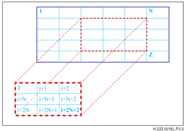
Figure V.3 – Example of subregion layout for a 3 x 3 ROI
