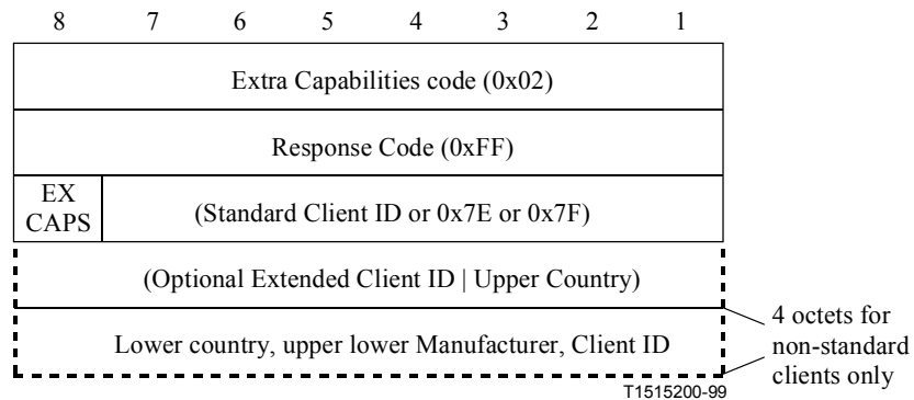
Figure 6/H.224 – CME extra capabilities command
