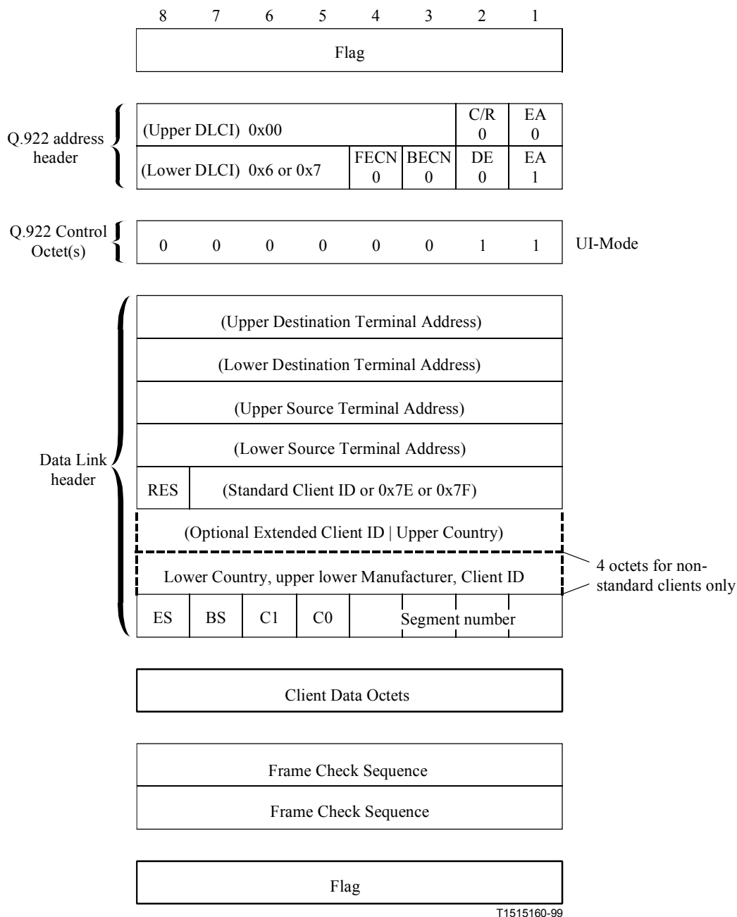
Figure 2/H.224 – H.224 protocol octet structure
