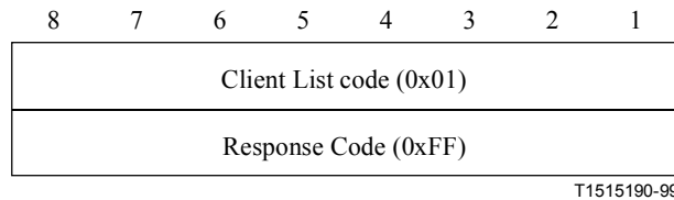
Figure 5/H.224 – CME client list command
