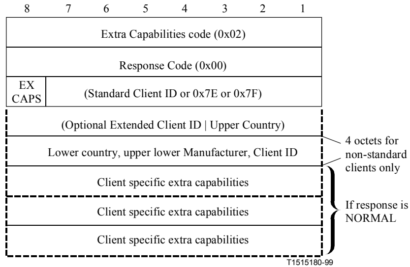
Figure 4/H.224 – CME extra capabilities message
