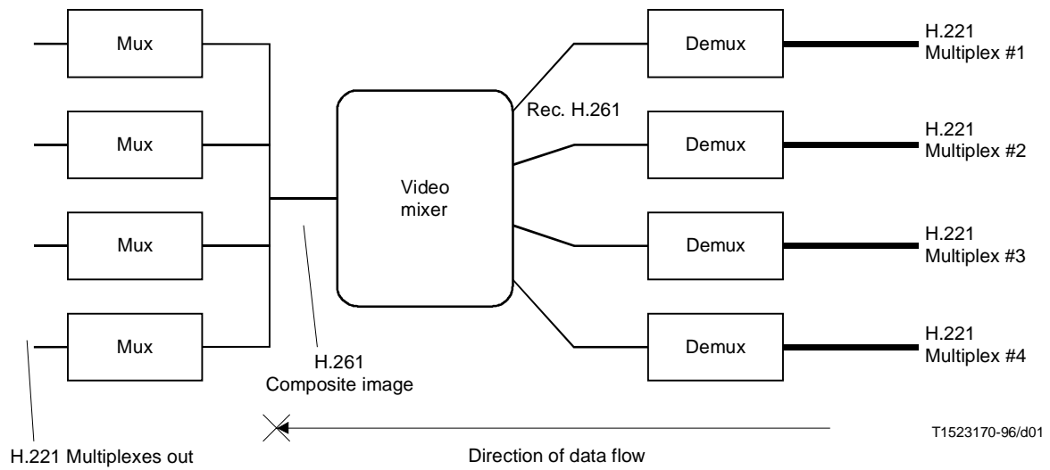
Figure 1/H.243 – Video mixing example: Quadrature
