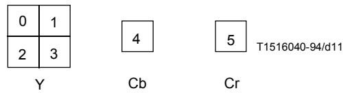
Figure 6-10 – 4:2:0 Macroblock structure
