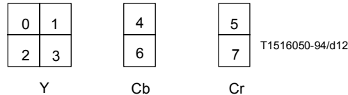
Figure 6-11 – 4:2:2 Macroblock structure
