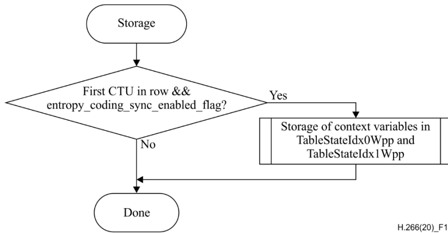
Figure 14 – Flowchart of CABAC storage process (informative)
