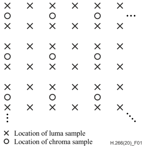
Figure 1 – Nominal vertical and horizontal locations of 4:2:0 luma and chroma samples in a picture
