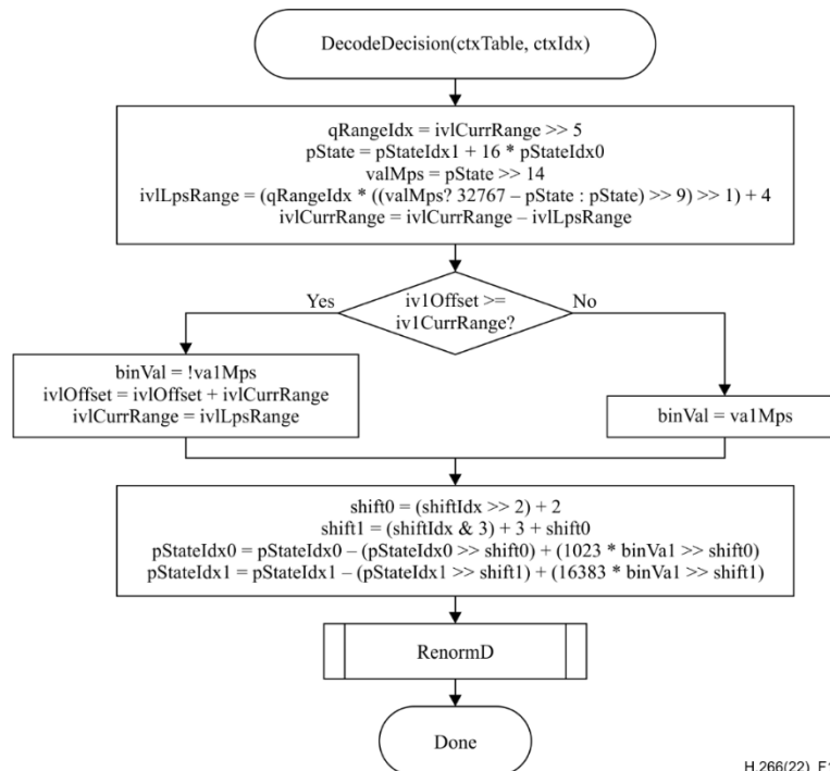
Figure 16 – Flowchart for decoding a decision
