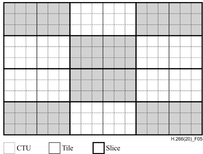
Figure 5 – A picture with 18 by 12 luma CTUs that is partitioned into 24 tiles and 9 rectangular slices (informative)
