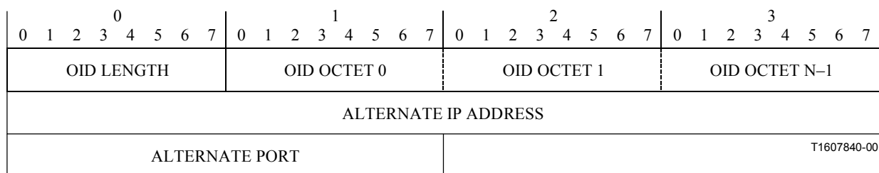
Figure E.11/H.323 – Nack reason 2 structure
