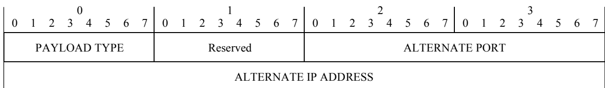
Figure E.10/H.323 – Nack reason 1 structure
