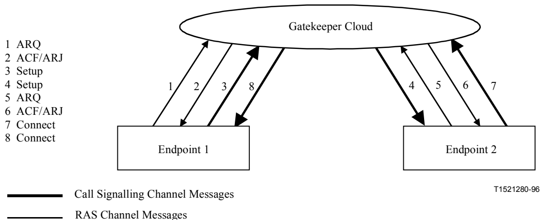
Figure 25/H.323 – Gatekeeper routed call signalling
