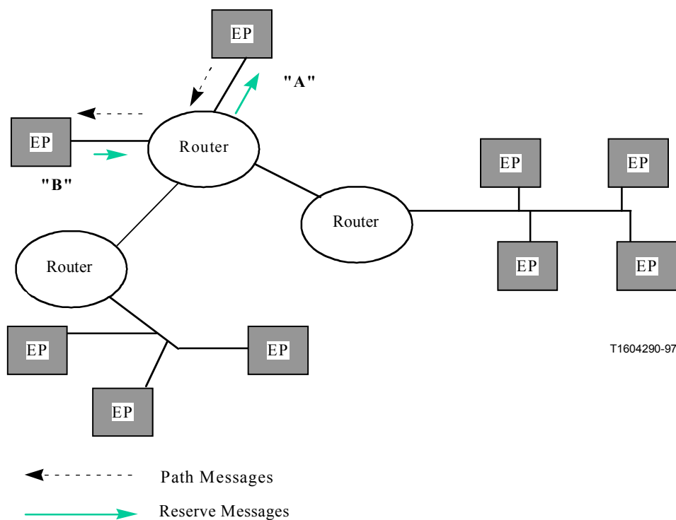
Figure II.1/H.323 – Resource reservation for a point-to-point connection
