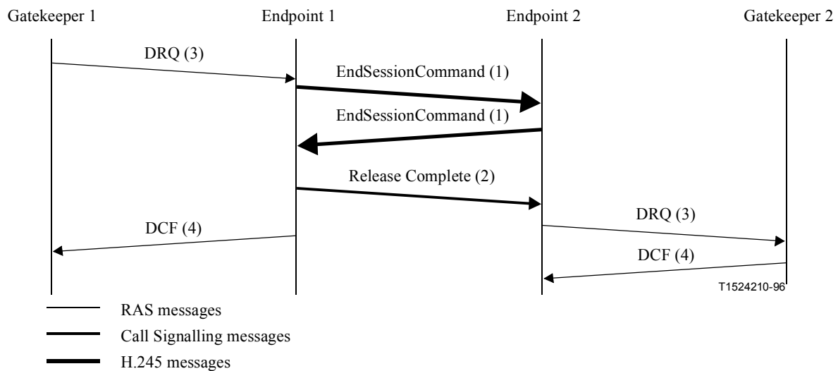
Figure 52/H.323 – Gatekeeper initiated call clearing
