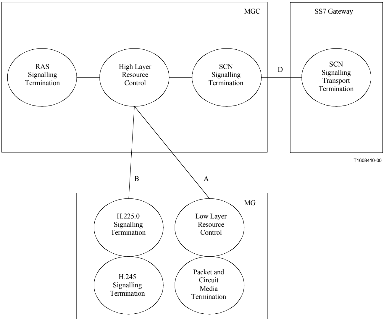
Figure 9/H.323 – SS7 terminated in the media gateway
