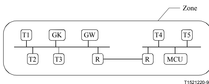
Figure 3/H.323 – Zone
