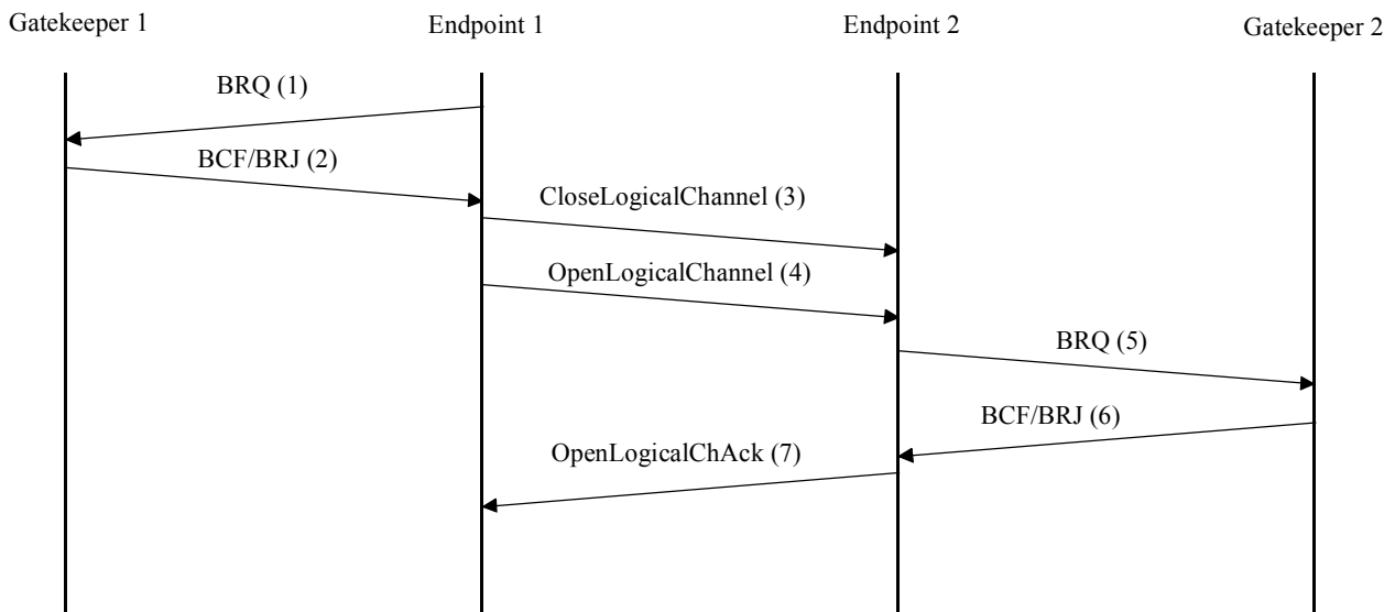
Figure 43/H.323 – Bandwidth change request – Transmitter change
