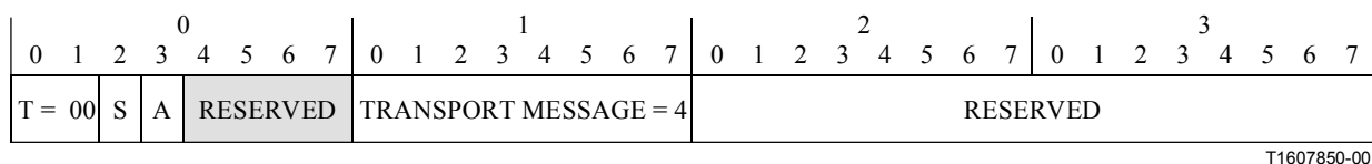
Figure E.12/H.323 – Restart message structure
