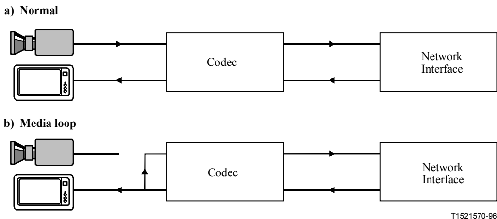
Figure 55/H.323 – Loopback
