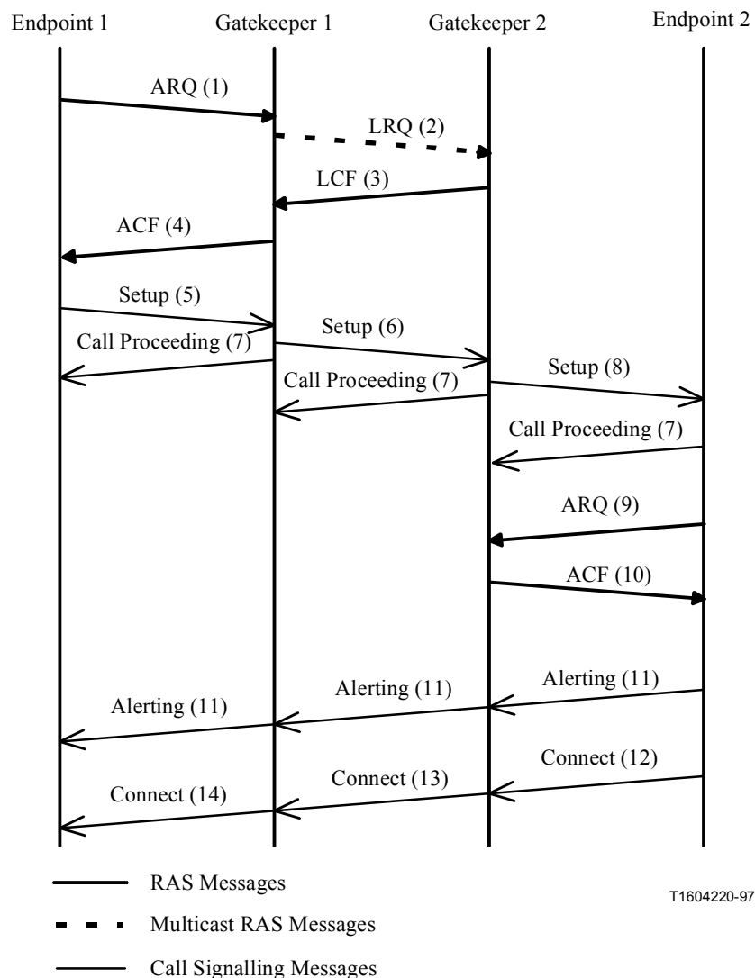
Figure 40/H.323 – Optional called endpoint signalling
