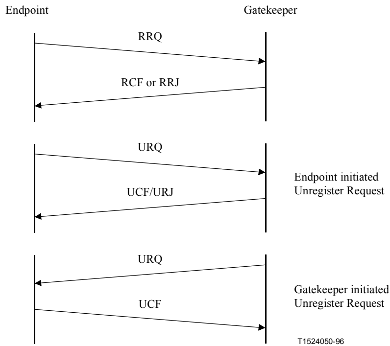
Figure 24/H.323 – Registration
