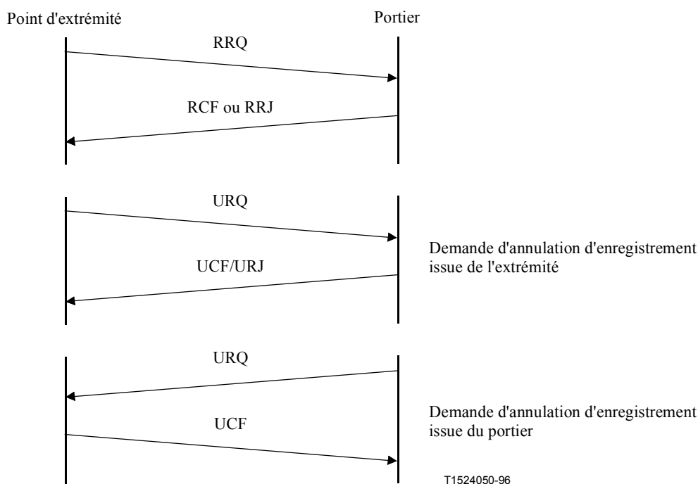
Figure 24/H.323 – Enregistrement
