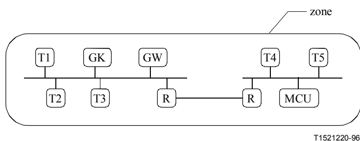
Figure 3/H.323 – Zone
