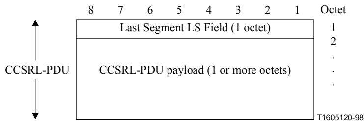
Figure C.3/H.324 – CCSRL-PDU Format
