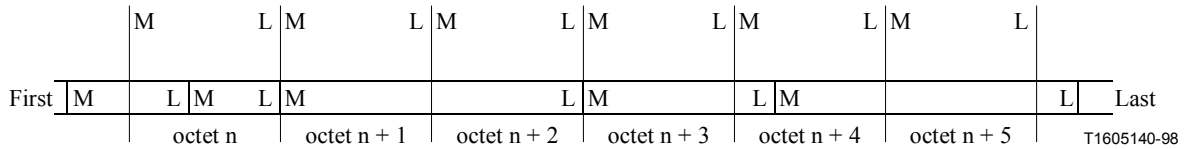
Figure I.2/H.324 – Output split into octets
