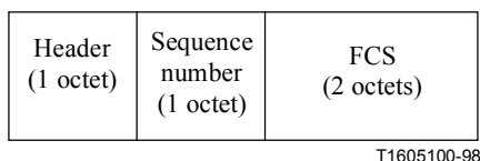
Figure A.3 /H.324 – Format of NSRP response frame
