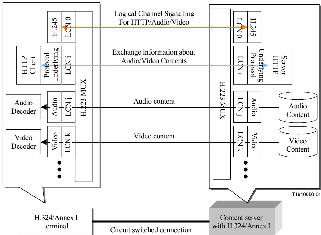
Figure I.1/H324 – An application using H.324 Annex I
