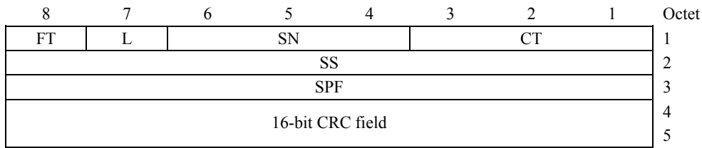
Figure H.4/H.324 – Full header format
