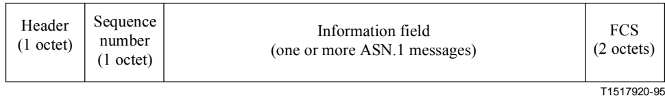
Figure A.2/H.324 – Format of SRP command frames for MultimediaSystemControlPDU messages
