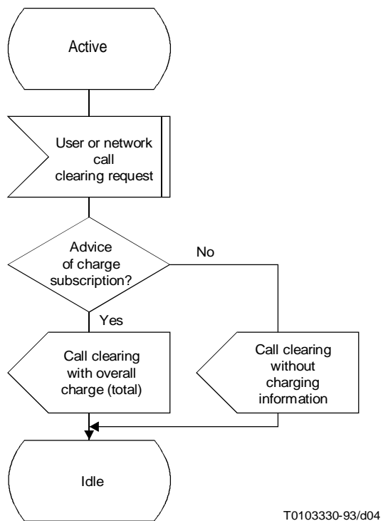
FIGURE 2/I.256.2b Charging information – Cumulative information at call clearing
