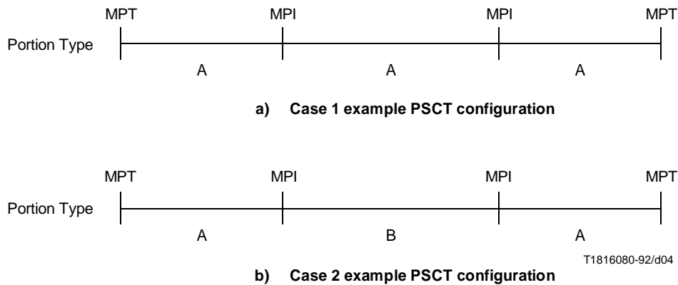
FIGURE B.1/I.355 Definition of Case 1 and Case 2 example PSCT configurations
