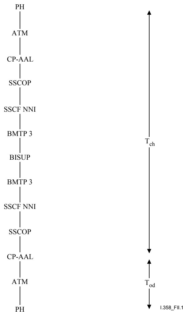
Figure II.1/I.358 – Reference model for the cross-office handling time T_{ch}
