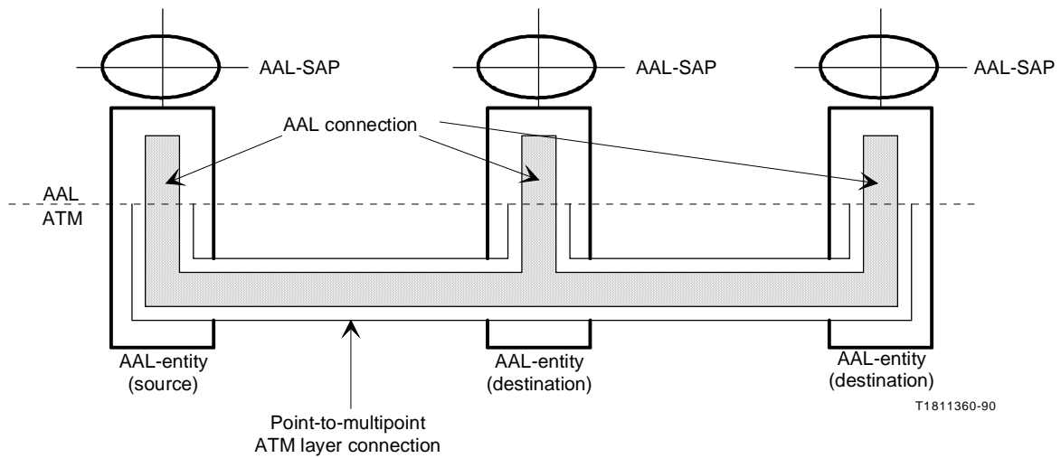
FIGURE 4b/I.363 Point-to-multipoint AAL connection
