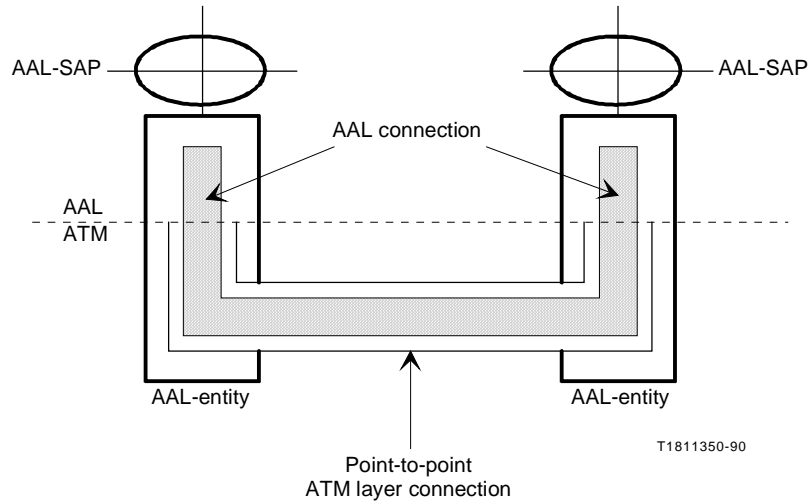
FIGURE 4a/I.363 Point-to-point AAL connection
