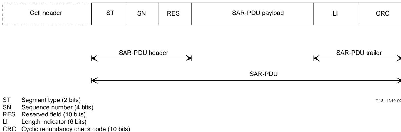
FIGURE 3/I.363 SAR-PDU format for AAL type 3
