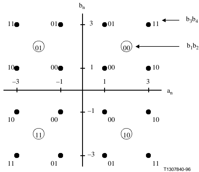
Figure 3/I.432.4 – Constellation de signaux en modulation 16-QAM
