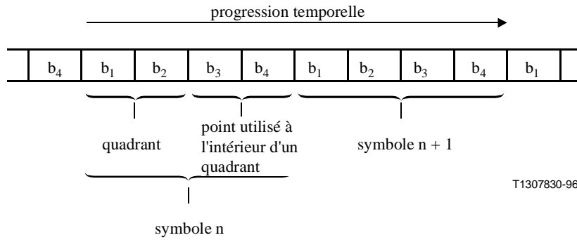
Figure 2/I.432.4 – Mappage bits-symbole en modulation 16-QAM
