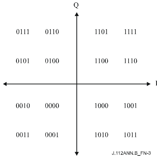
Figure B.N-3/J.112 – 16QAM differential-coded symbol mapping
