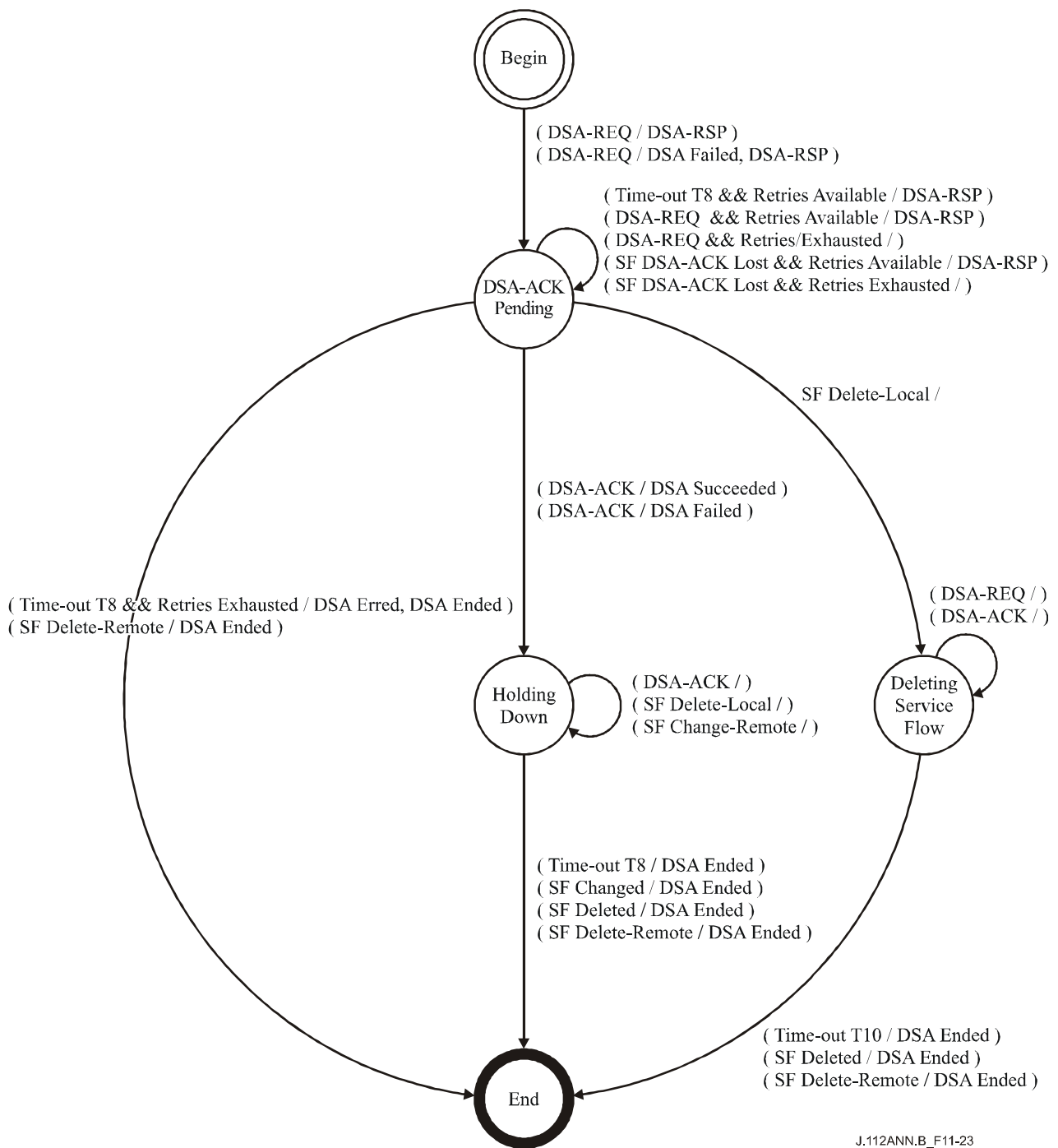
Figure B.11-23/J.112 – DSA – Remotely initiated Transaction State Transition Diagram
