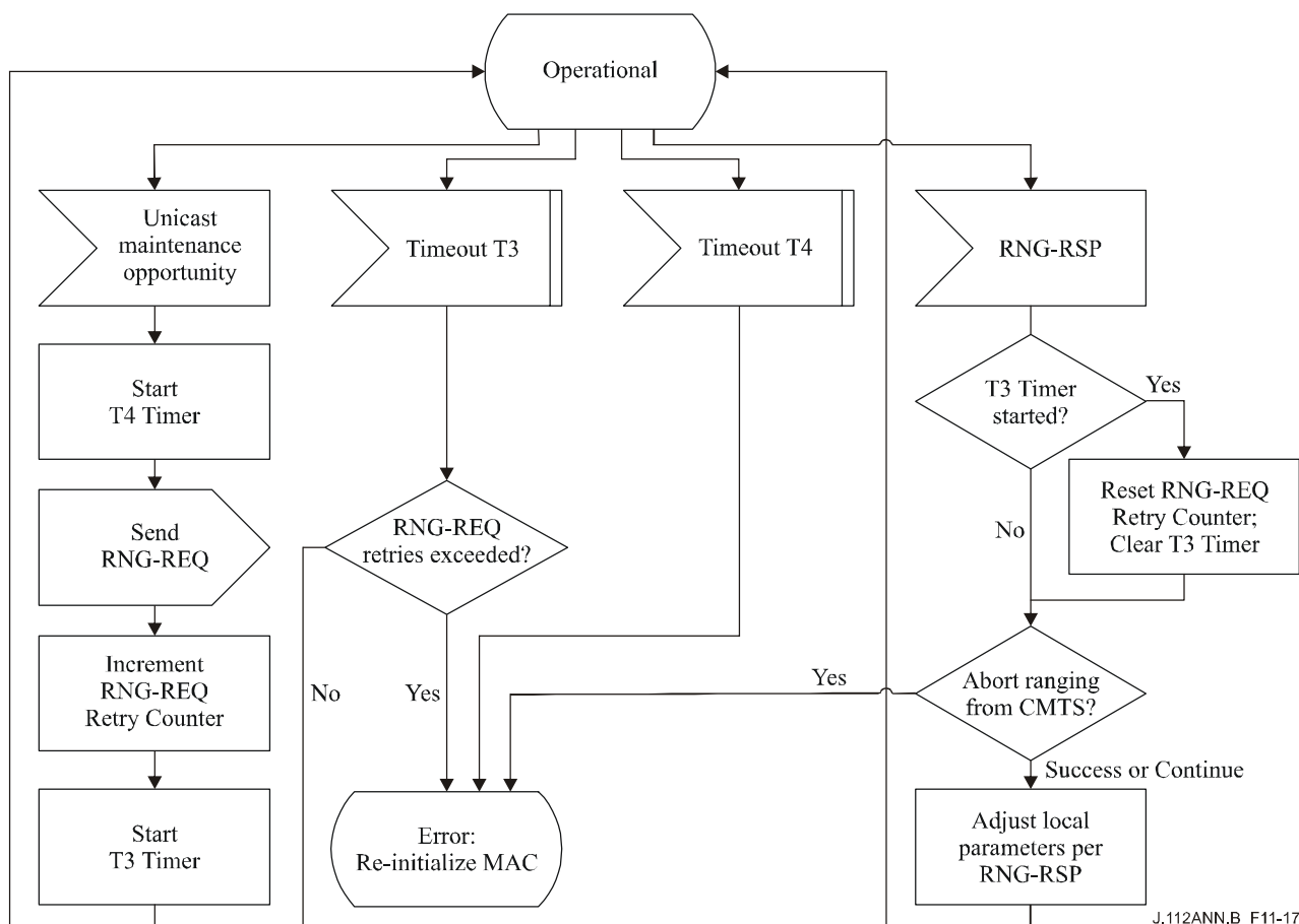
Figure B.11-17/J.112 – Periodic Ranging – CM view
