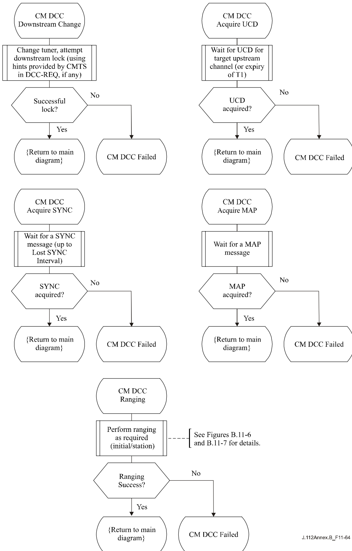
Figure B.11-64/J.112 – Dynamically Changing Channels: CM view, Part 3
