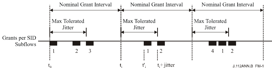
Figure B.M-1/J.112 – Example jitter with multiple grants per SID
