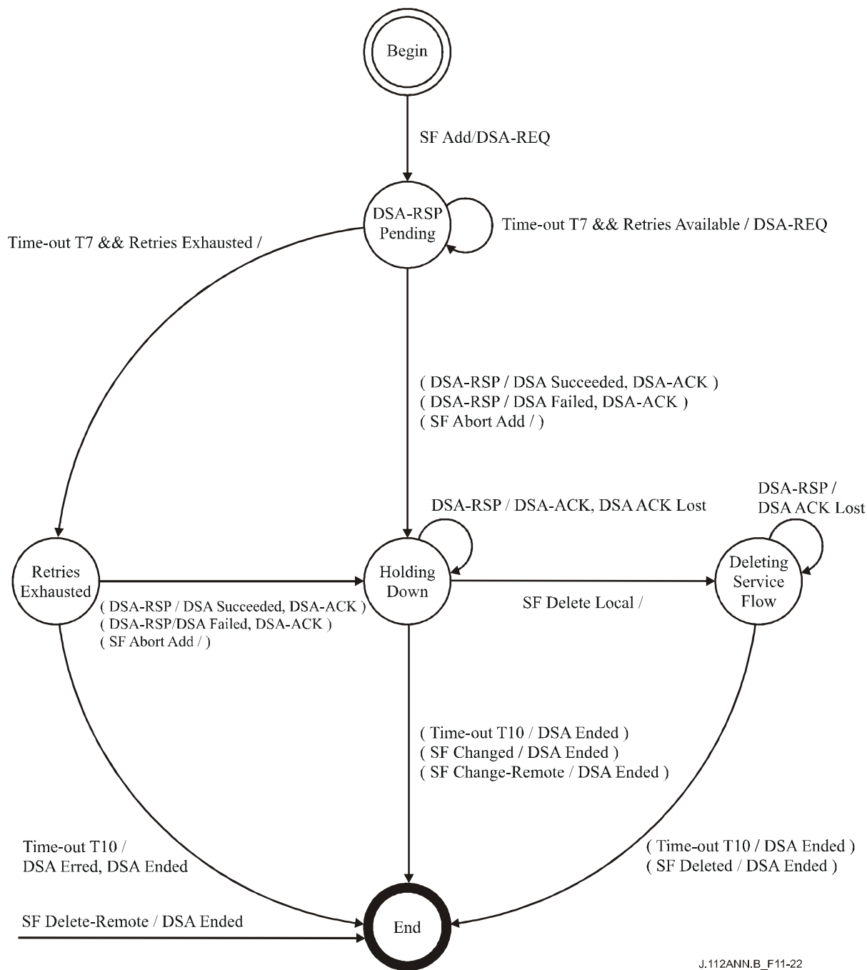
Figure B.11-22/J.112 – DSA – Locally initiated Transaction State Transition Diagram
