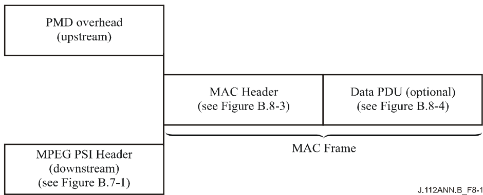
Figure B.8-1/J.112 – Generic MAC frame format
