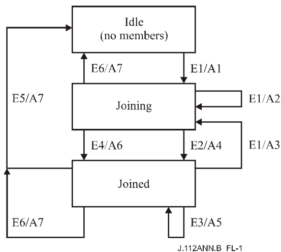
Figure B.L-1/J.112 – IGMP support – CM passive mode
