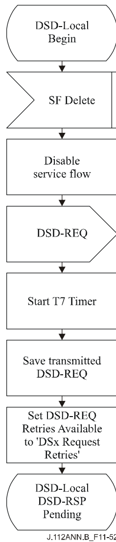
Figure B.11-52/J.112 – DSD – Locally initiated Transaction Begin State Flow Diagram
