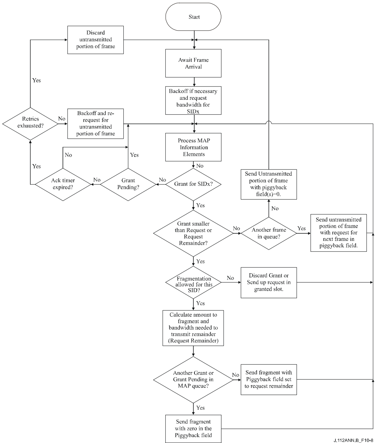
Figure B.10-8/J.112 – CM fragmentation flowchart
