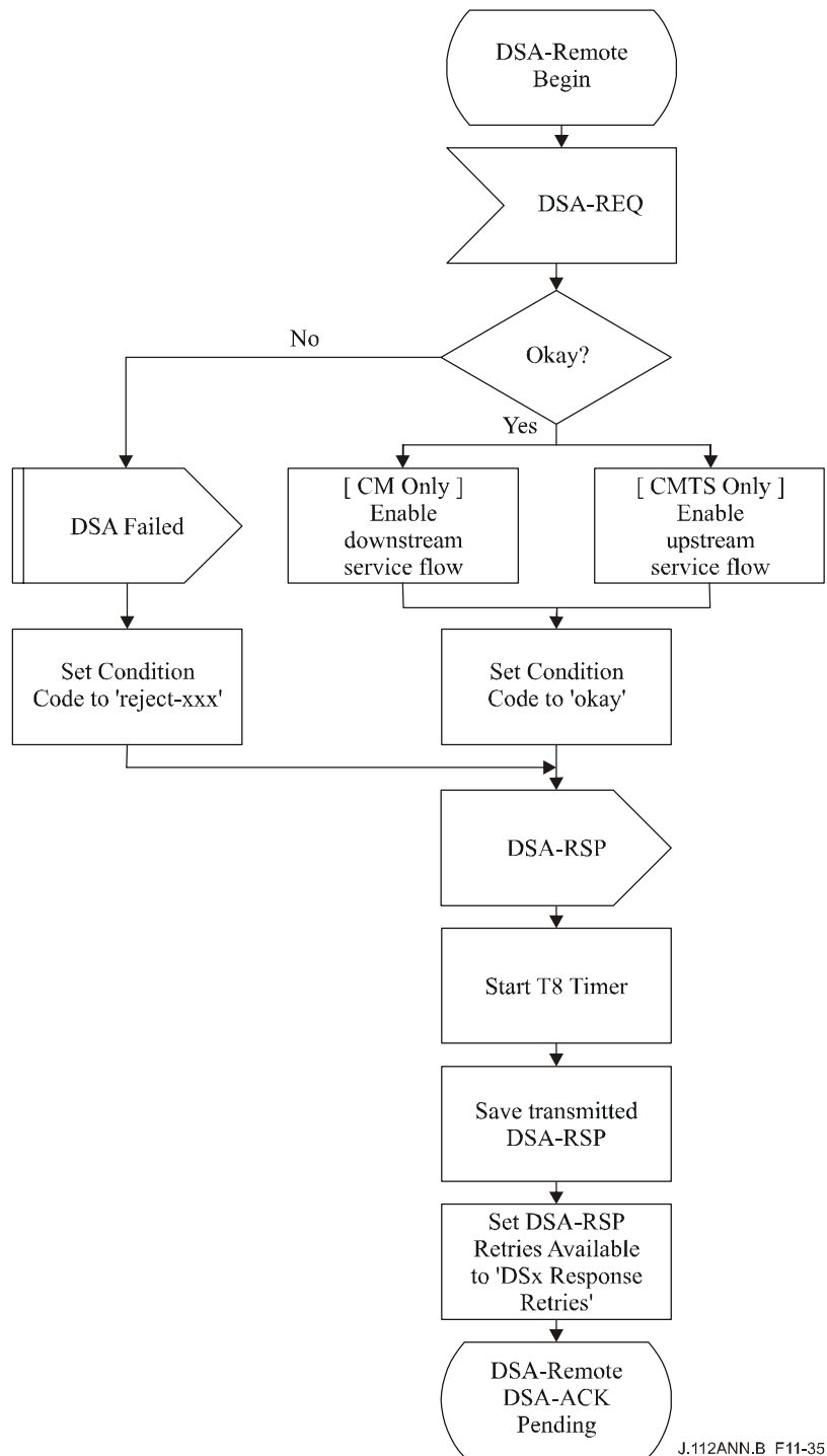
Figure B.11-35/J.112 – DSA – Remotely initiated Transaction Begin State Flow Diagram
