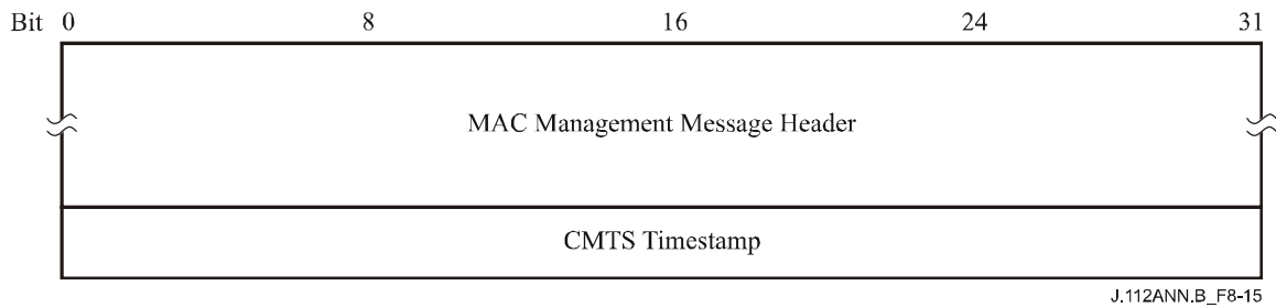
Figure B.8-15/J.112 – Format of Packet PDU following the Timing Header
