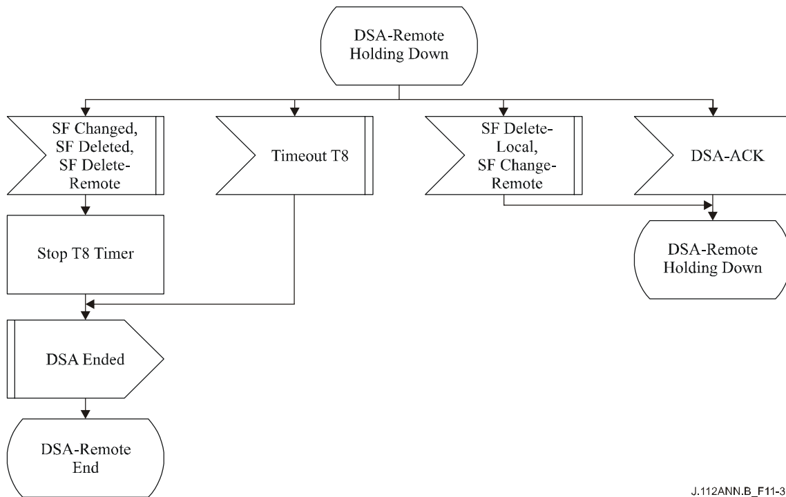
Figure B.11-37/J.112 – DSA – Remotely initiated Transaction Holding Down State Flow Diagram
