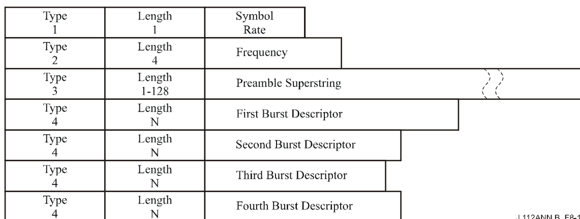
Figure B.8-18/J.112 – Example of UCD encoded TLV data
