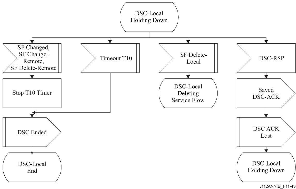
Figure B.11-43/J.112 – DSC – Locally initiated Transaction Holding Down State Flow Diagram
