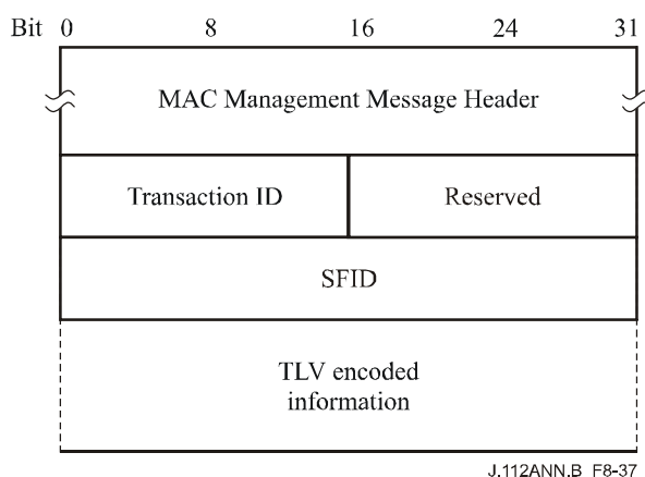
Figure B.8-37/J.112 – Dynamic Service Deletion-Request
