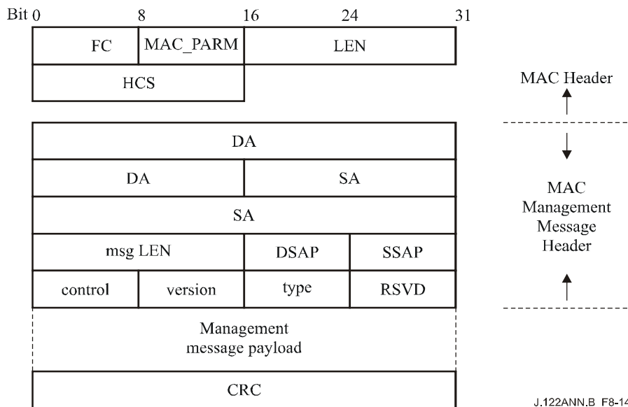
Figure B.8-14/J.112 – MAC Header and MAC Management Message Header fields
