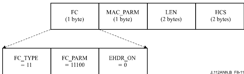
Figure B.8-11/J.112 – Concatenation MAC Header format
