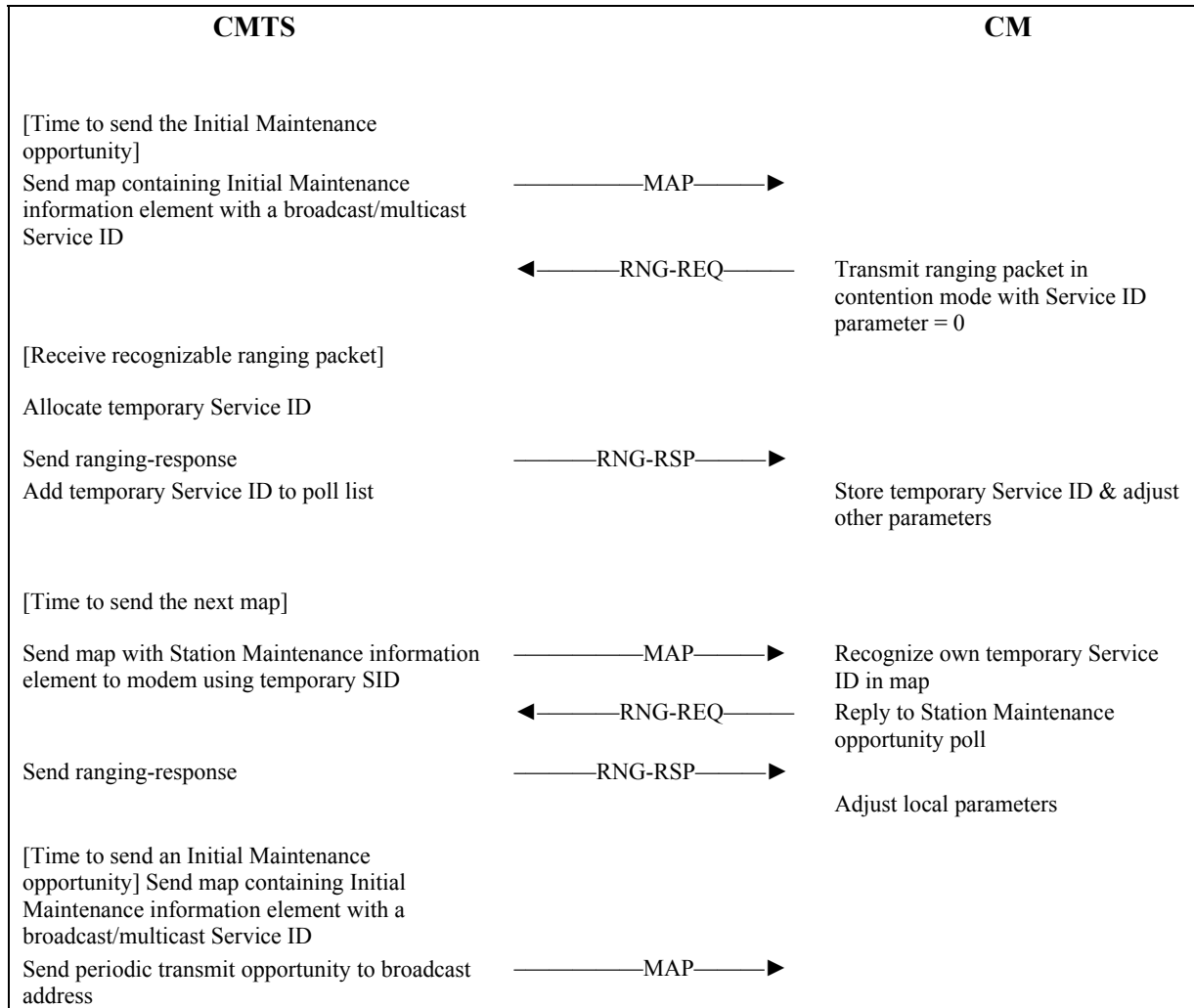
Figure B.11-5/J.112 – Ranging and automatic adjustments procedure
