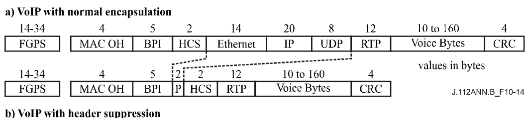
Figure B.10-14/J.112 – Upstream payload header suppression example
