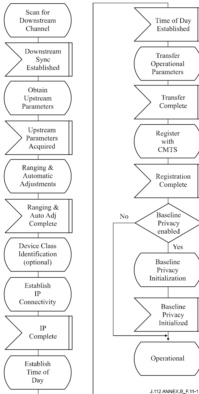
Figure B.11-1/J.112 – CM initialization overview
