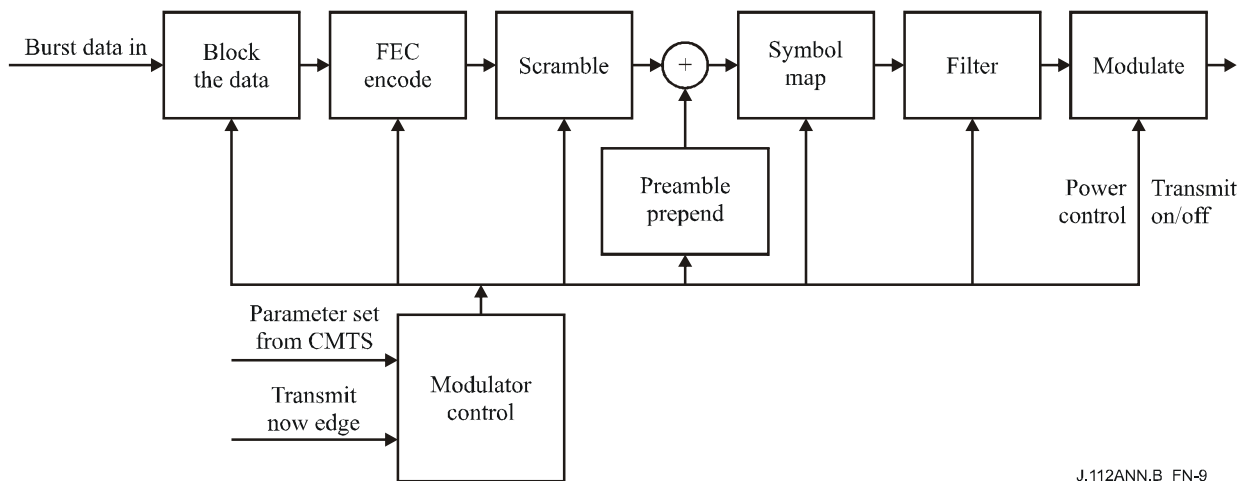
Figure B.N-9/J.112 – Signal-processing sequence
