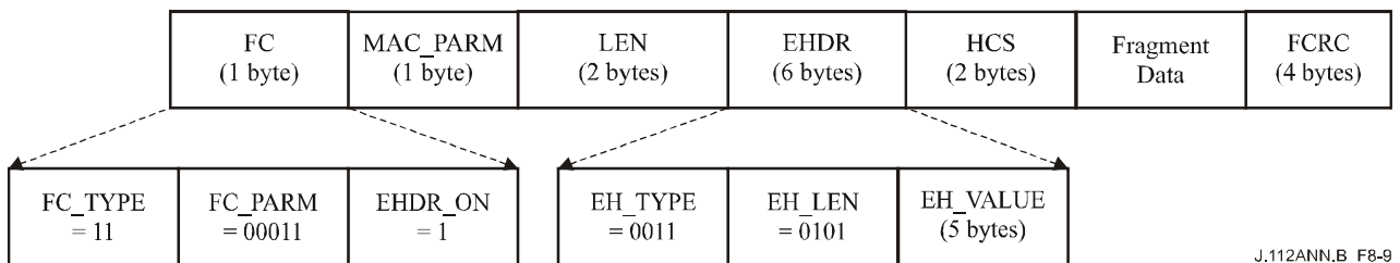
Figure B.8-9/J.112 – Fragmentation MAC Header format
