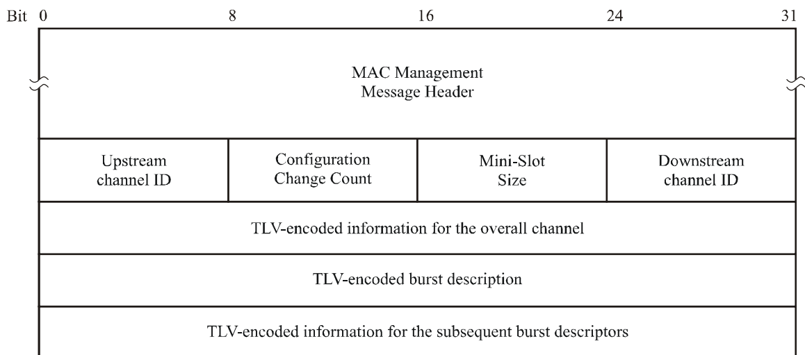
Figure B.8-16/J.112 – Upstream Channel Descriptor
