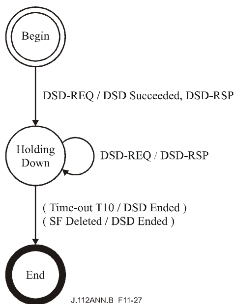
Figure B.11-27/J.112 – Dynamic Deletion (DSD) – Remotely initiated Transaction State Transition Diagram
