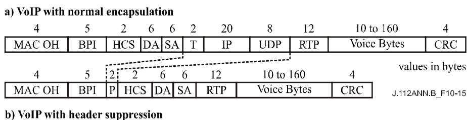
Figure B.10-15/J.112 – Downstream Payload Header Suppression example
