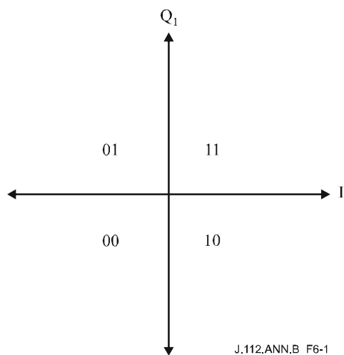
Figure B.6-1/J.112 – QPSK symbol mapping
