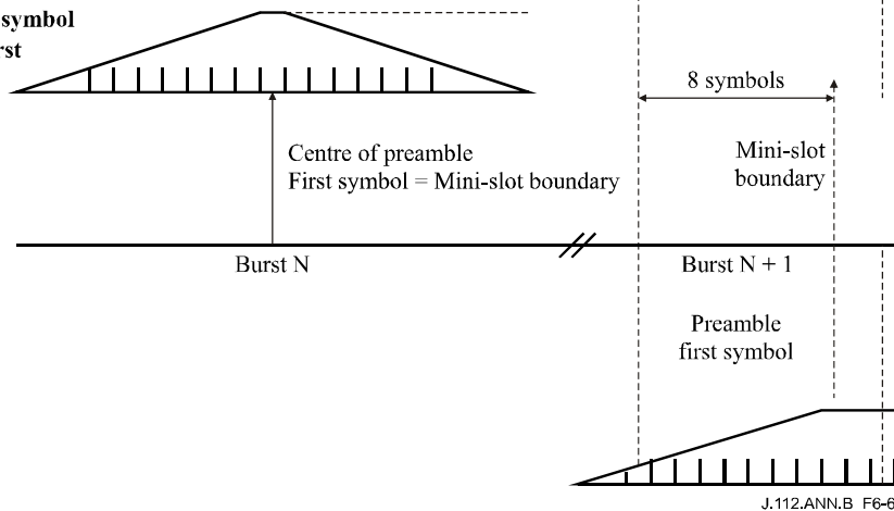
Figure B.6-6/J.112 – Nominal burst timing
