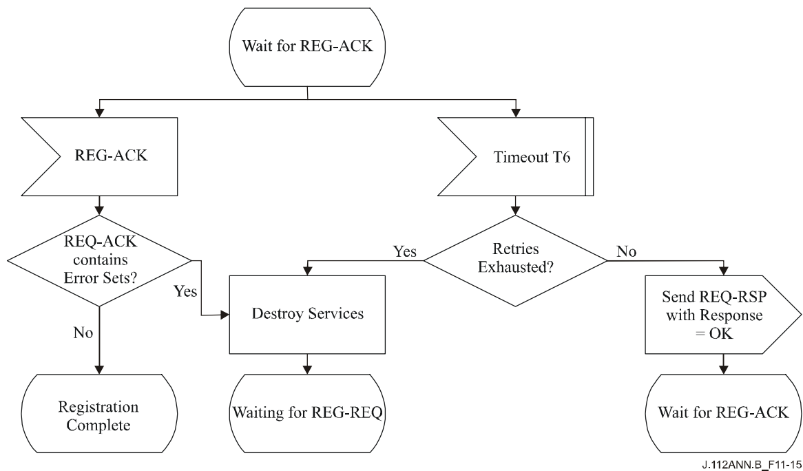
Figure B.11-15/J.112 – Registration Acknowledgment – CMTS
