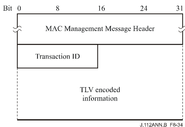
Figure B.8-34/J.112 – Dynamic Service Change-Request
