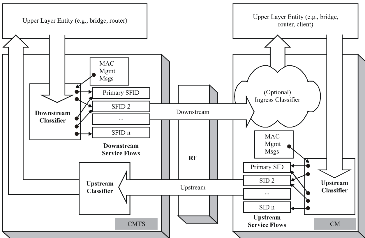
Figure B.10-3/J.112 – Classification within the MAC layer
