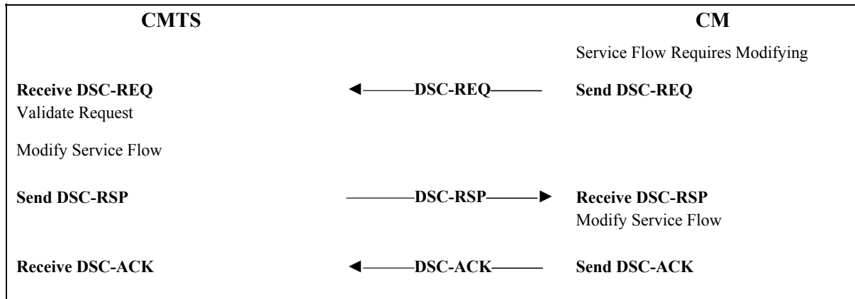
Figure B.11-39/J.112 – CM-initiated DSC
