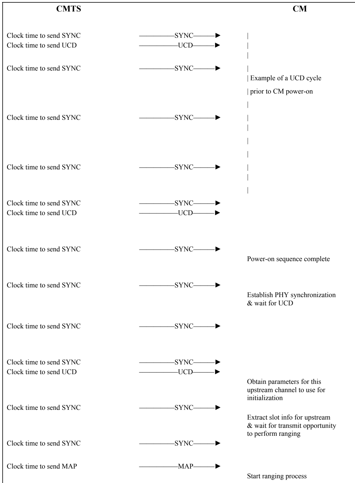
Figure B.11-4/J.112 – Message flows during scanning and upstream parameter acquisition
