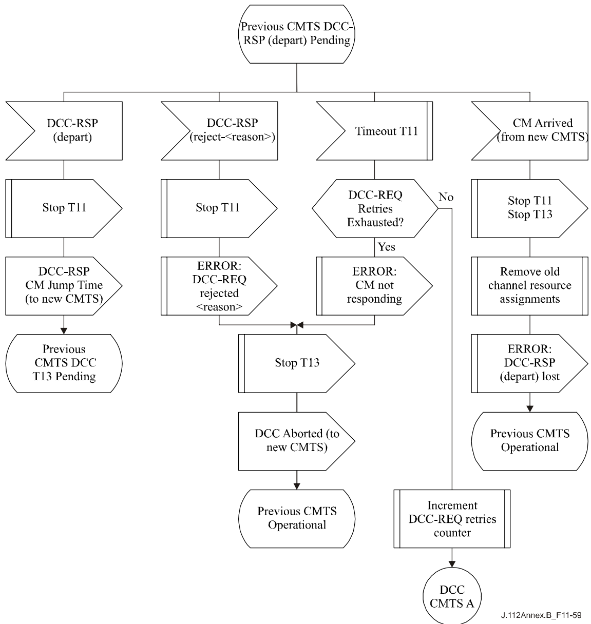
Figure B.11-59/J.112 – Dynamically Changing Channels: CMTS view, Part 2
