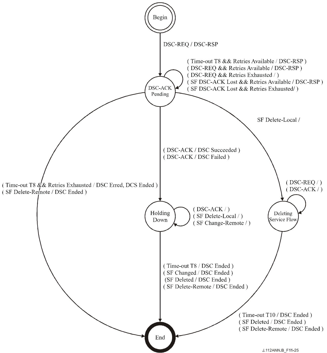
Figure B.11-25/J.112 – DSC – Remotely initiated Transaction State Transition Diagram
