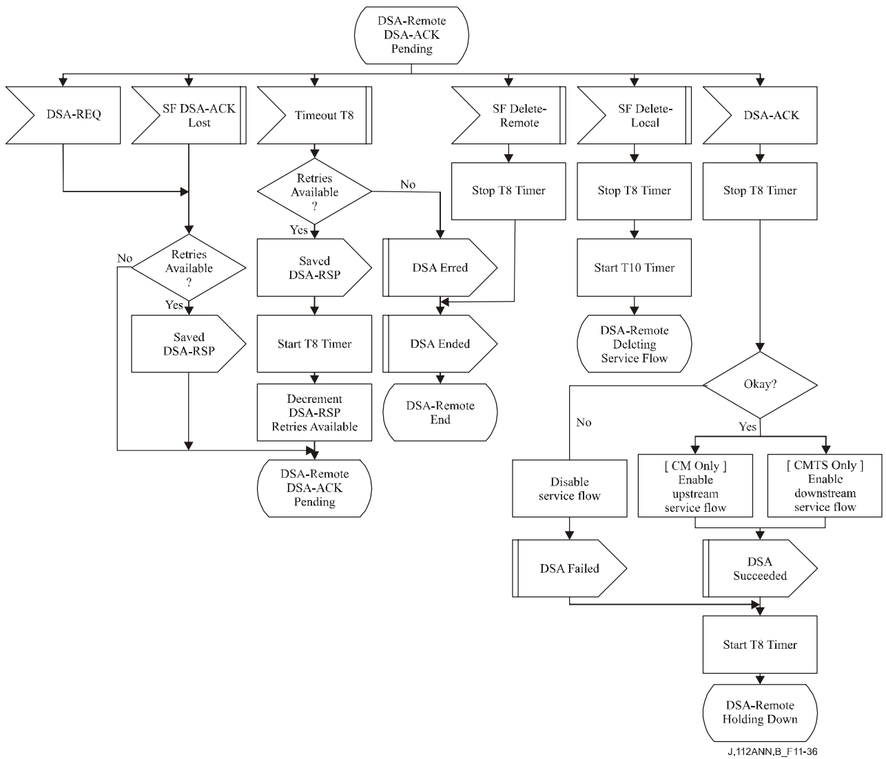
Figure B.11-36/J.112 – DSA – Remotely initiated Transaction DSA-ACK Pending State Flow Diagram
