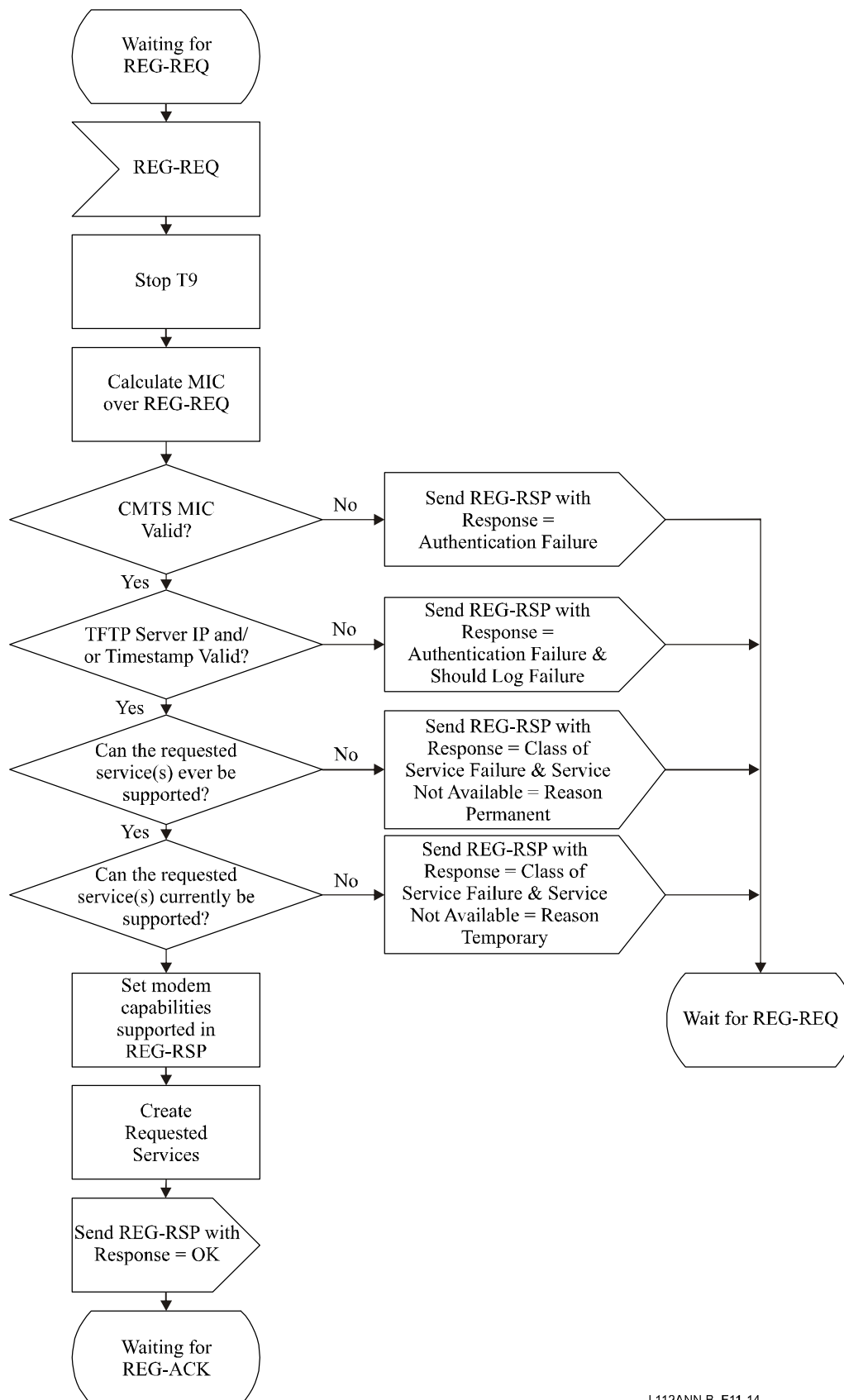
Figure B.11-14/J.112 – Registration – CMTS
