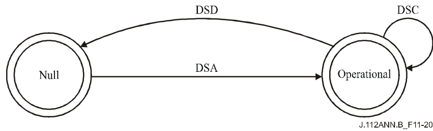
Figure B.11-20/J.112 – Dynamic Service Flow overview
