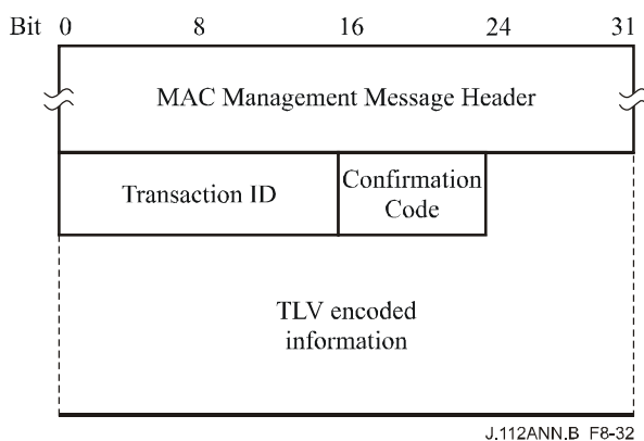
Figure B.8-32/J.112 – Dynamic Service Addition-Response
