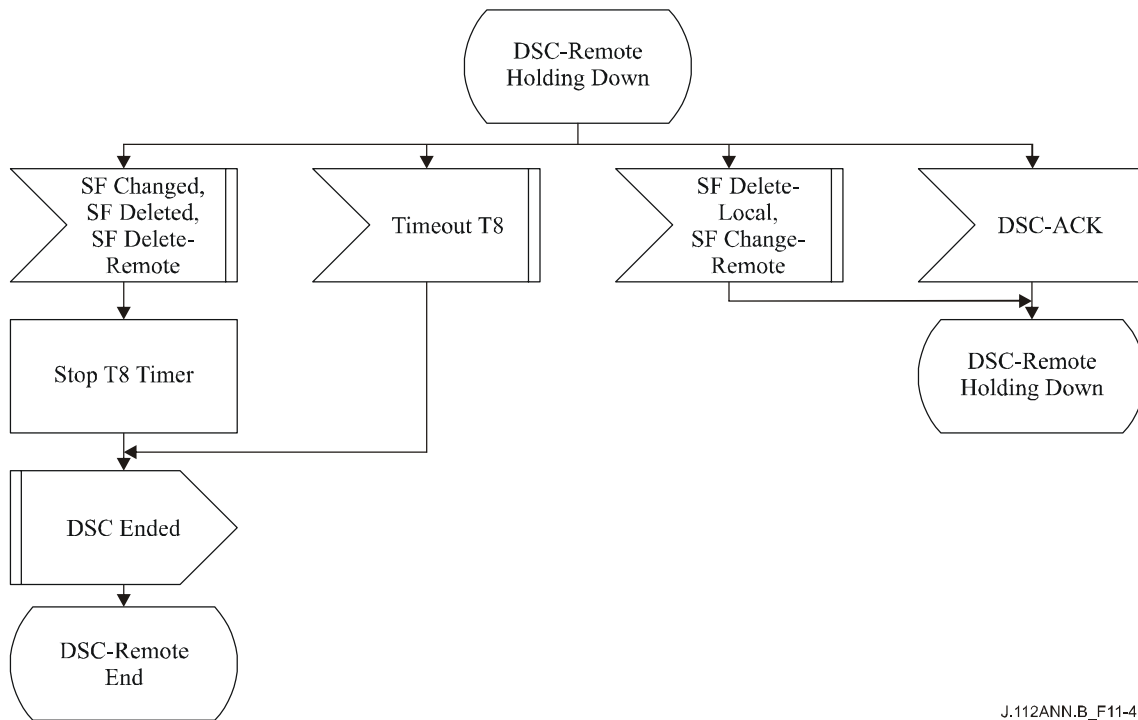
Figure B.11-48/J.112 – DSC – Remotely initiated Transaction Holding Down State Flow Diagram
