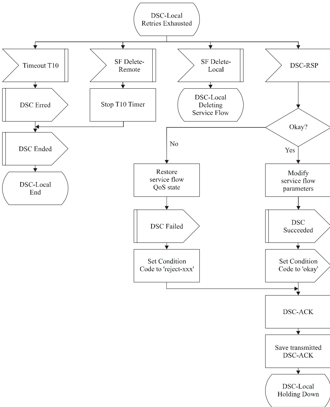
Figure B.11-44/J.112 – DSC – Locally initiated Transaction Retries Exhausted State Flow Diagram
