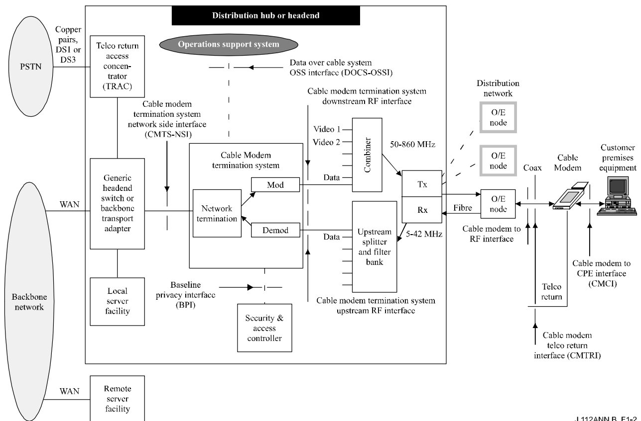
Figure B.1-2/J.112 – Data-over-cable reference architecture
