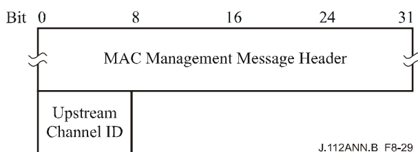
Figure B.8-29/J.112 – Upstream Channel Change-Request
