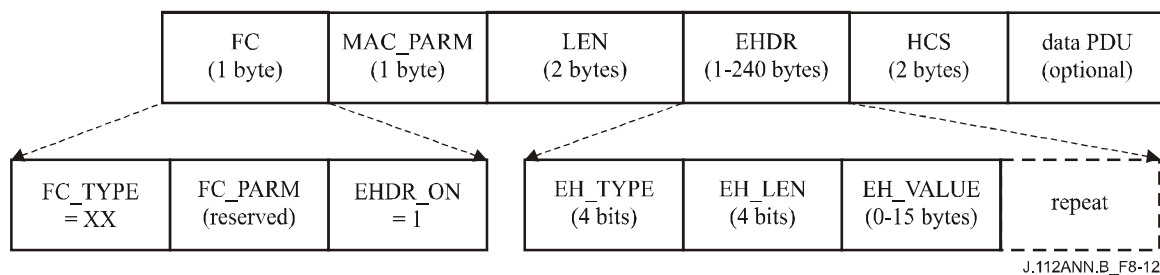
Figure B.8-12/J.112 – Extended MAC format
