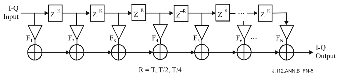
Figure B.N-5/J.112 – Transmit pre-equalizer structure
