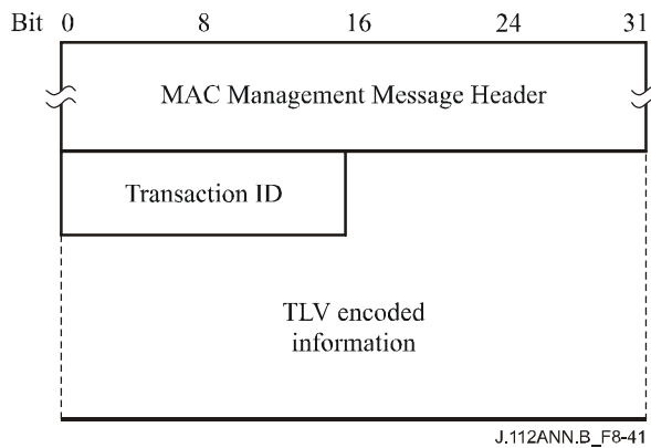
Figure B.8-41/J.112 – Dynamic Channel Change-Acknowledge
