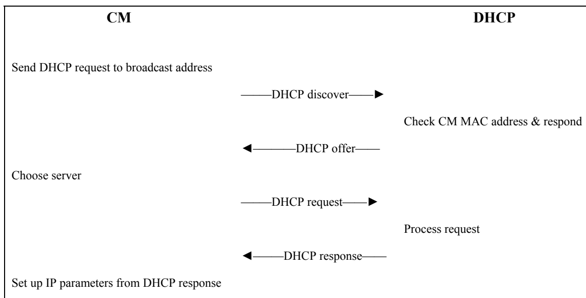
Figure B.11-10/J.112 – Establishing IP connectivity
