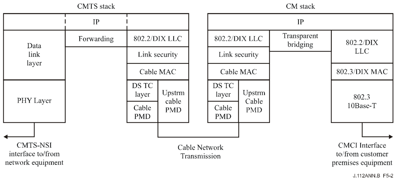
Figure B.5-2/J.112 – Data forwarding through the CM and CMTS
