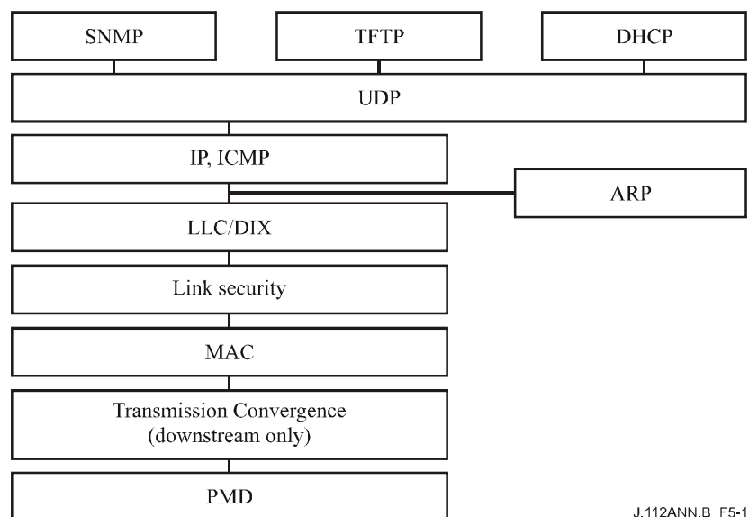
Figure B.5-1/J.112 – Protocol stack on the RF interface
