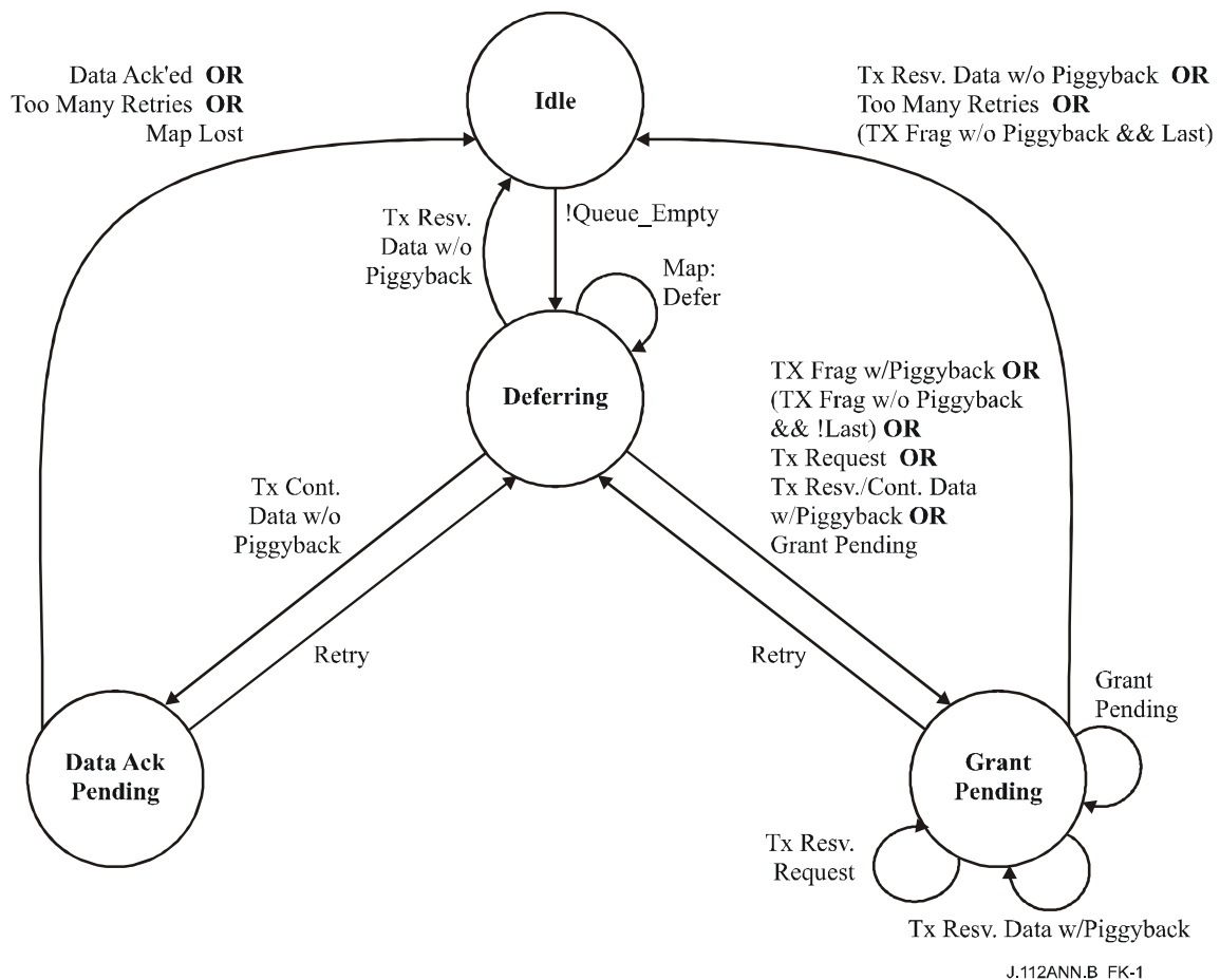
Figure B.K-1/J.112 – Transmission and deference state transition diagram
