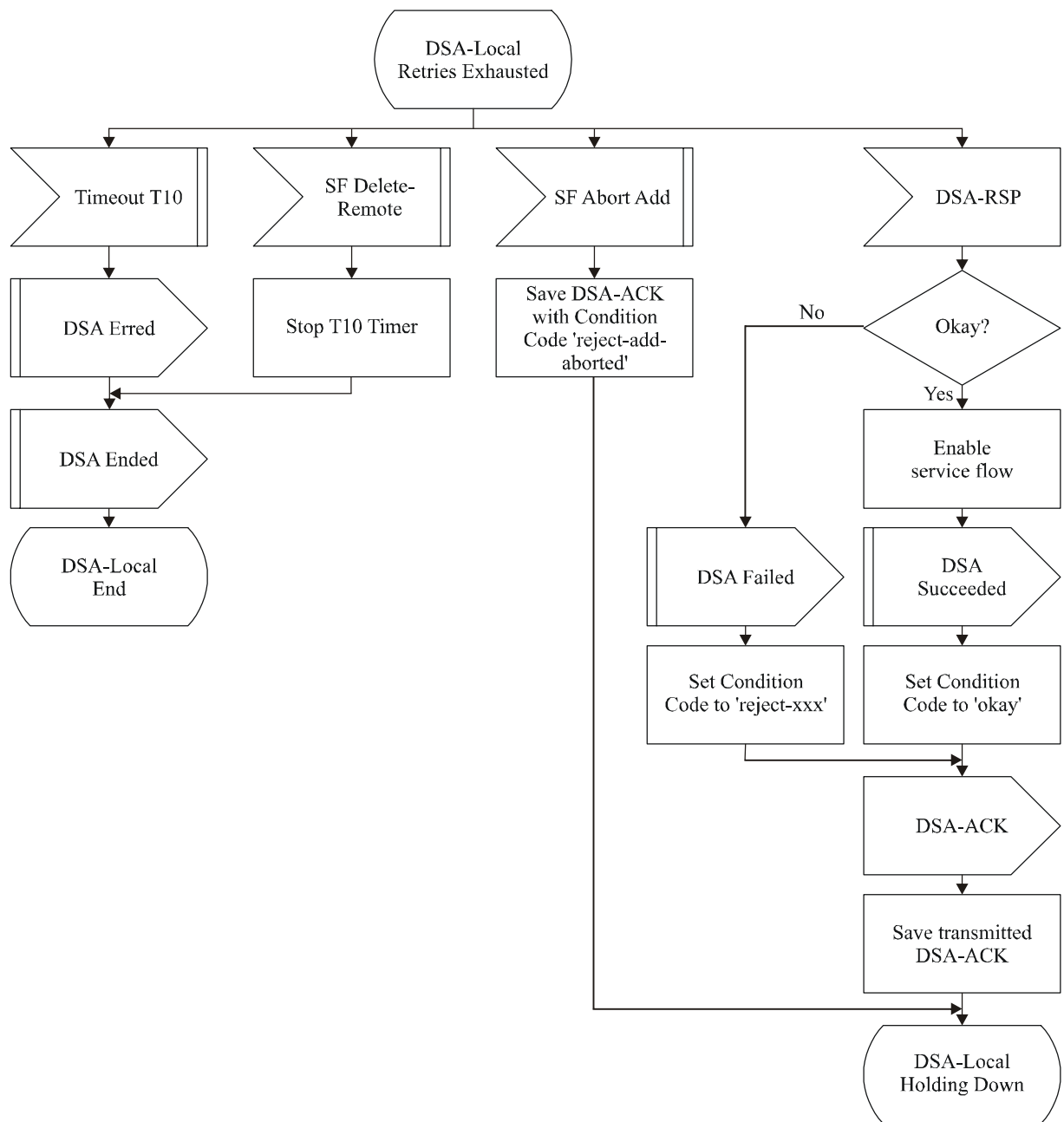
Figure B.11-33/J.112 – DSA – Locally initiated Transaction Retries Exhausted State Flow Diagram
