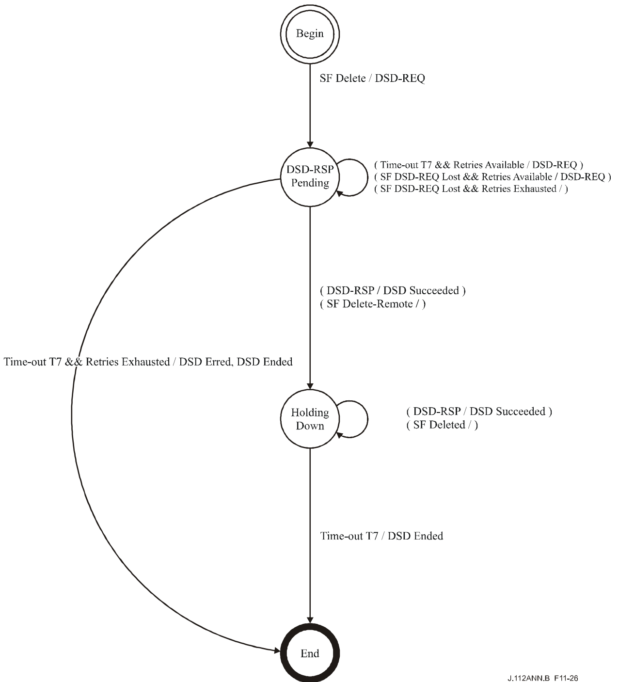
Figure B.11-26/J.112 – DSD – Locally initiated Transaction State Transition Diagram
