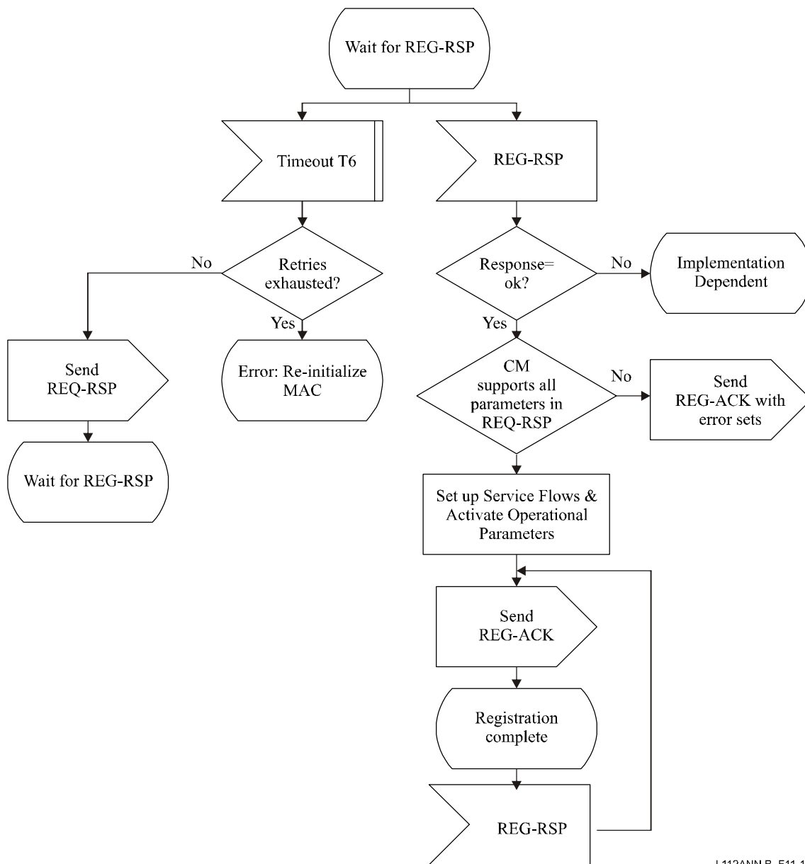
Figure B.11-13/J.112 – Wait for Registration-Response – CM
