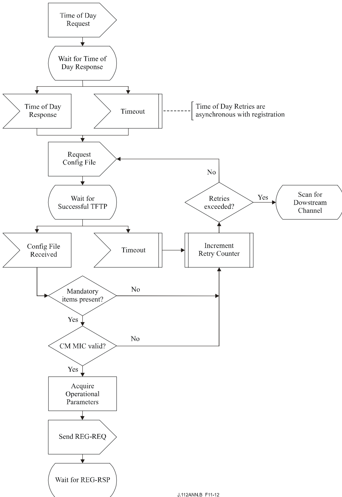
Figure B.11-12/J.112 – Registration – CM
