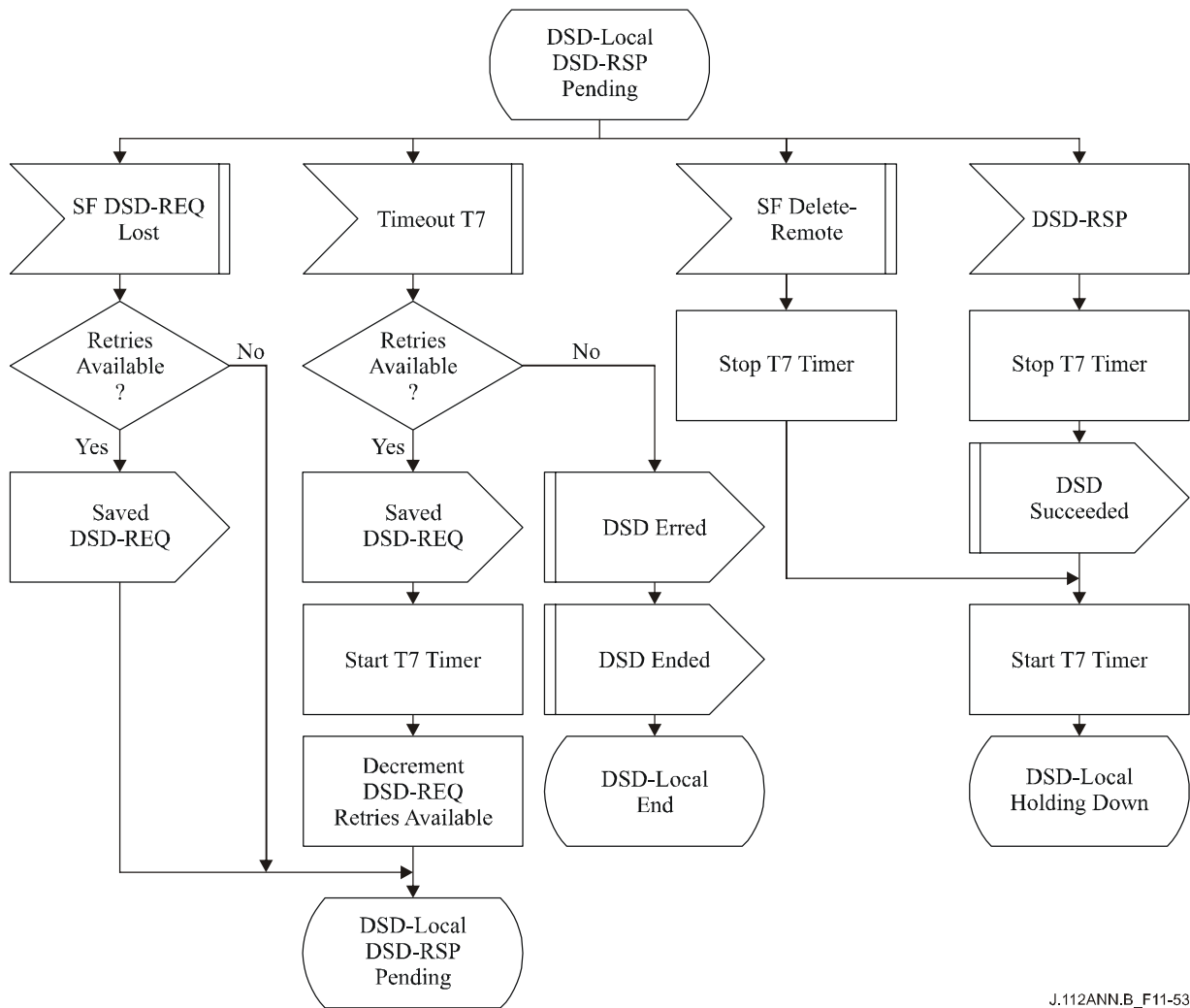
Figure B.11-53/J.112 – DSD – Locally initiated Transaction Pending State Flow Diagram
