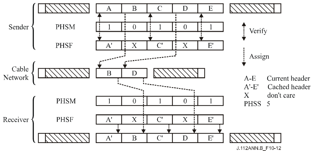
Figure B.10-12/J.112 – Payload header suppression with masking
