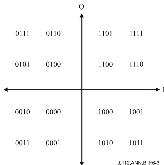
Figure B.6-3/J.112 – 16QAM differential-coded symbol mapping
