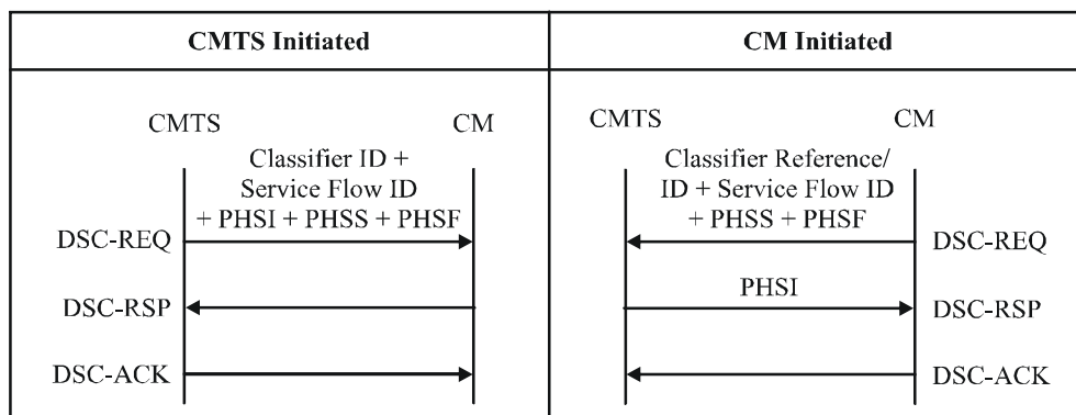
Figure B.10-13/J.112 – Payload header suppression signalling example
