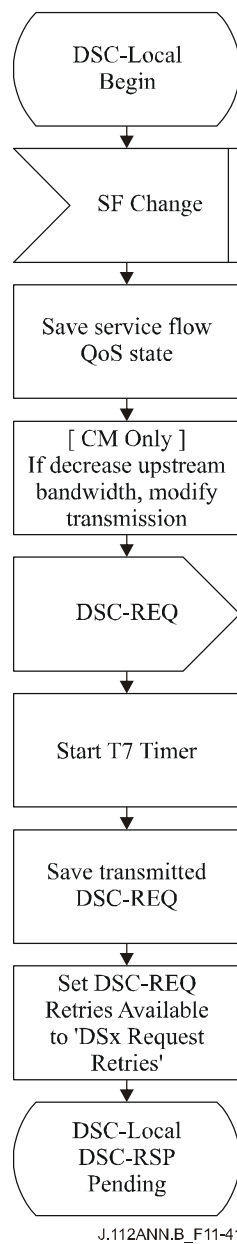
Figure B.11-41/J.112 – DSC – Locally initiated Transaction Begin State Flow Diagram
