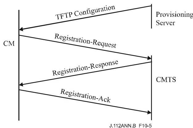
Figure B.10-5/J.112 – Registration Message Flow
