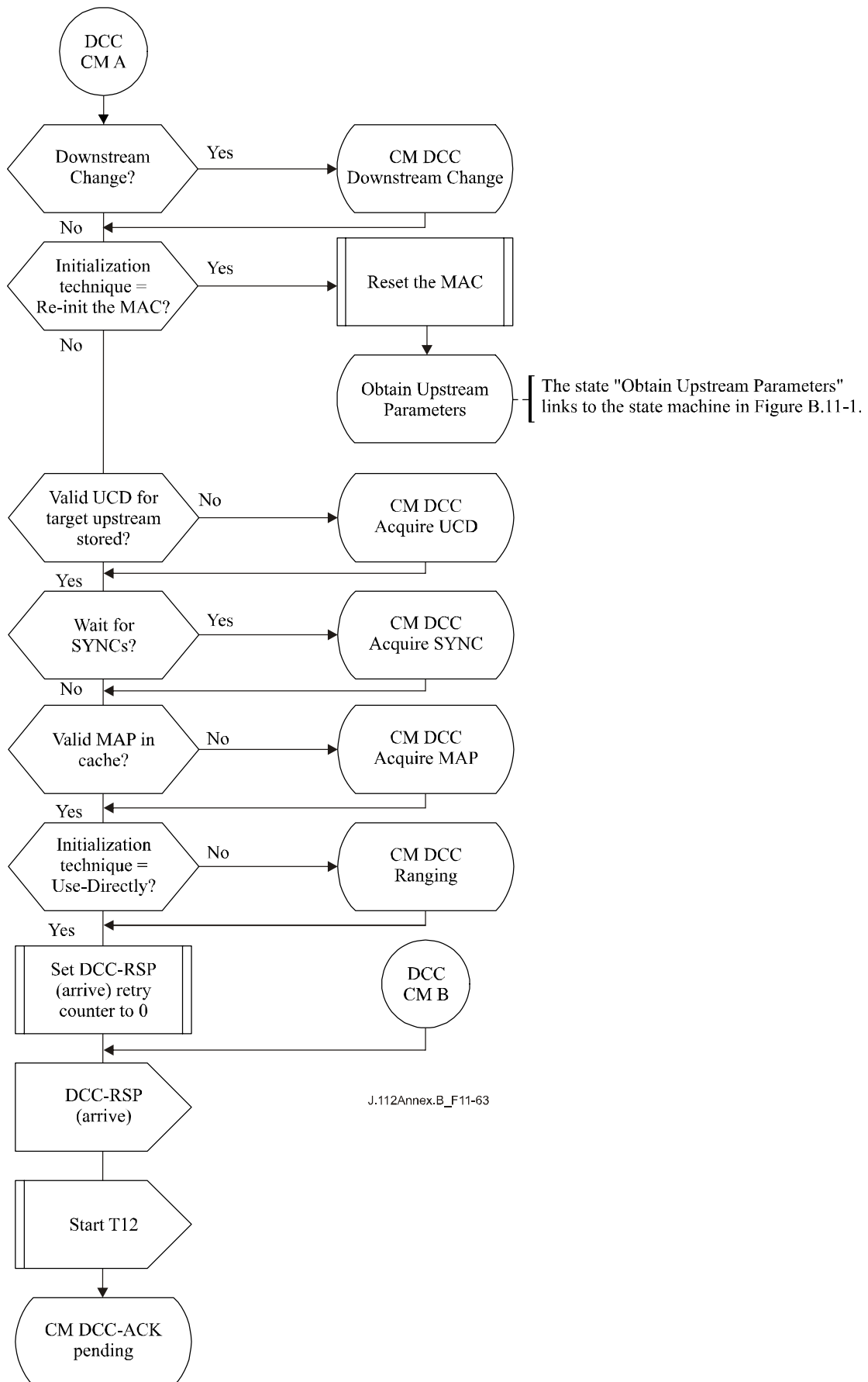
Figure B.11-63/J.112 – Dynamically Changing Channels: CM view, Part 2
