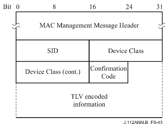
Figure B.8-43/J.112 – Device Class Identification-Response
