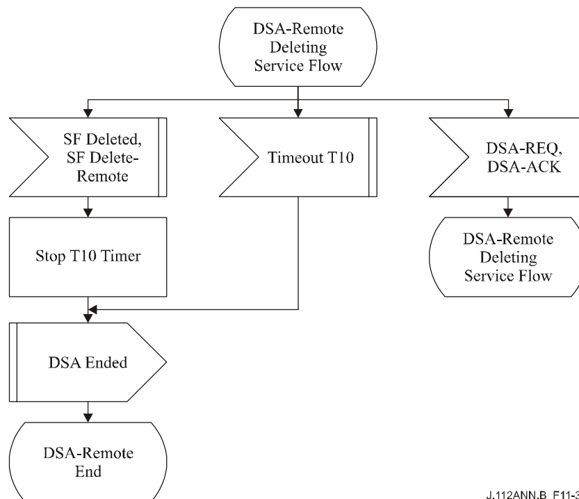
Figure B.11-38/J.112 – DSA – Remotely initiated Transaction Deleting Service State Flow Diagram
