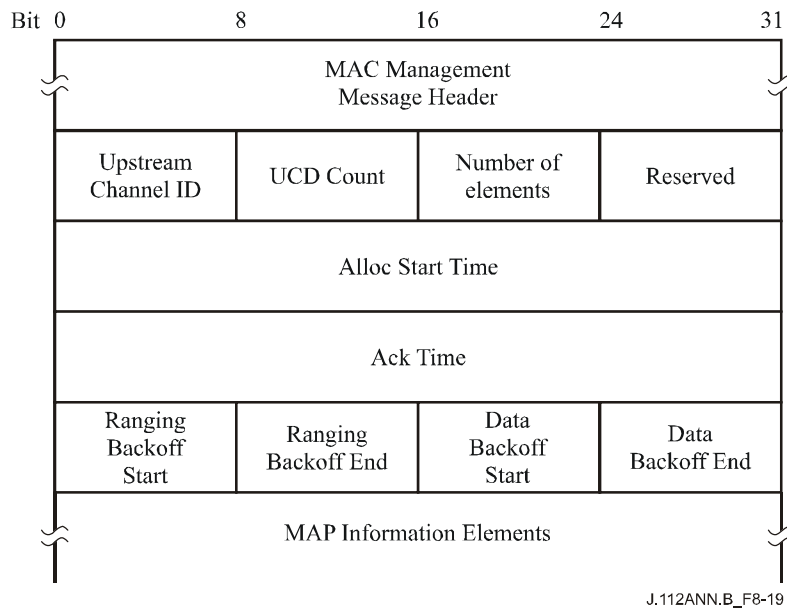
Figure B.8-19/J.112 – MAP format
