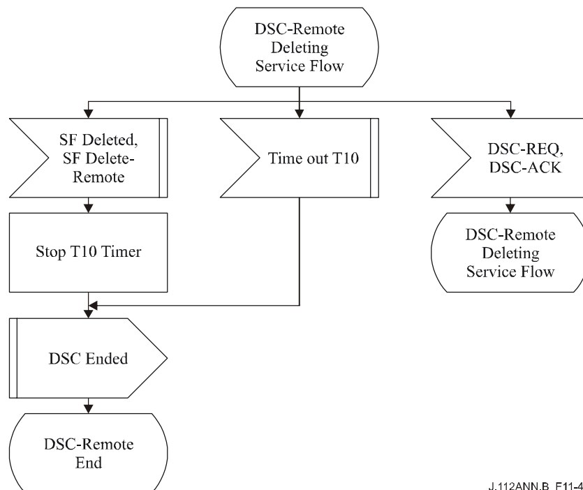
Figure B.11-49/J.112 – DSC – Remotely initiated Transaction Deleting Service Flow State Flow Diagram
