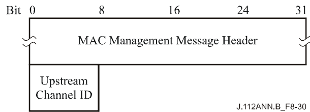
Figure B.8-30/J.112 – Upstream Channel Change-Response
