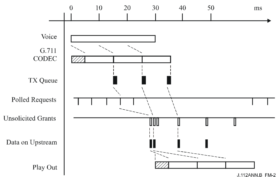
Figure B.M-2/J.112 – VAD start-up and stop
