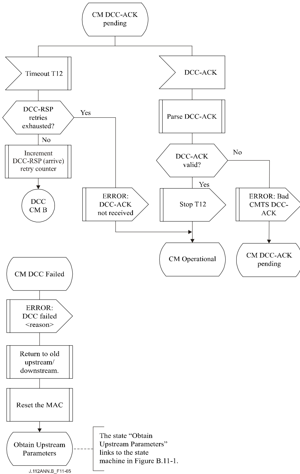
Figure B.11-65/J.112 – Dynamically Changing Channels: CM view, Part 4
