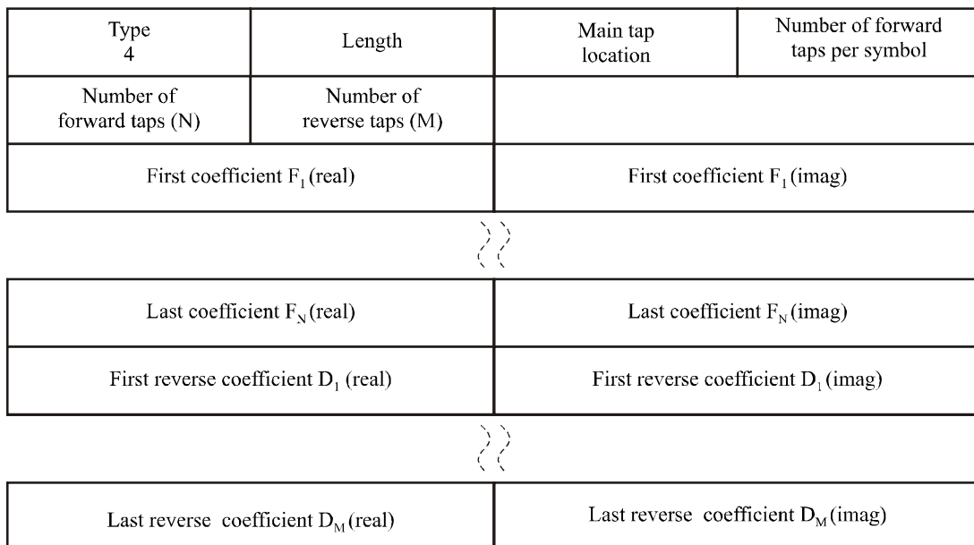
Figure B.8-23/J.112 – Generalized decision feedback equalization coefficients
