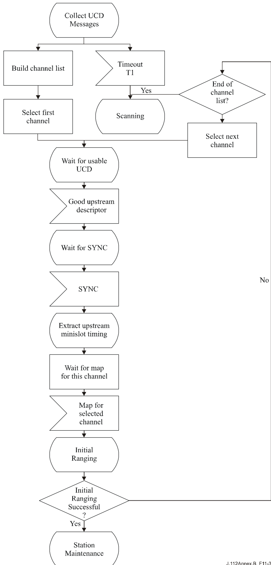
Figure B.11-3/J.112 – Obtaining upstream parameters
