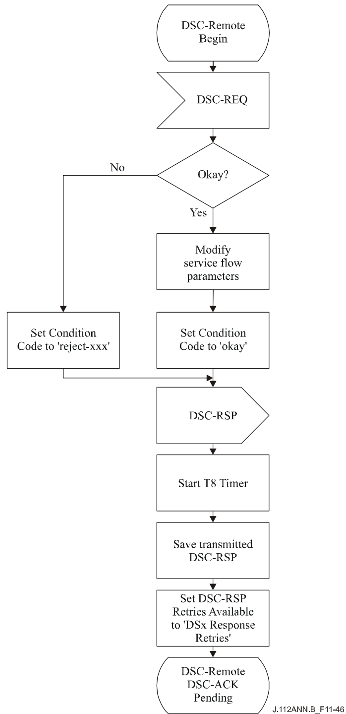
Figure B.11-46/J.112 – DSC – Remotely initiated Transaction Begin State Flow Diagram
