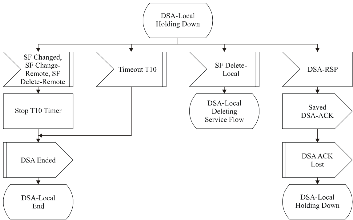
Figure B.11-32/J.112 – DSA – Locally initiated Transaction Holding State Flow Diagram
