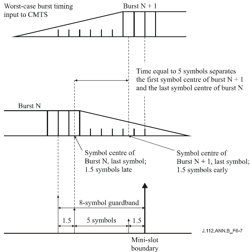
Figure B.6-7/J.112 – Worst-case burst timing
