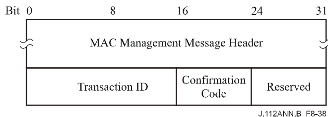
Figure B.8-38/J.112 – Dynamic Service Deletion-Response
