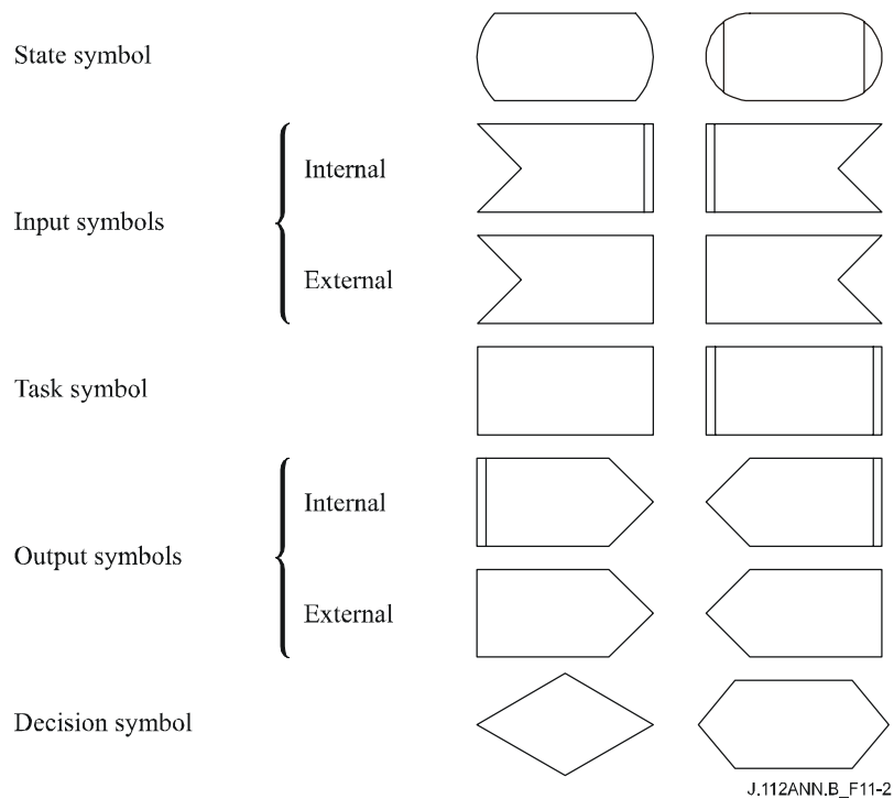
Figure B.11-2/J.112 – SDL notation
