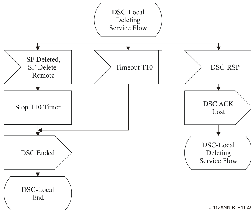
Figure B.11-45/J.112 – DSC – Locally initiated Transaction Deleting Service Flow State Flow Diagram
