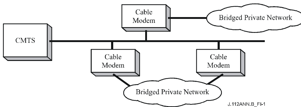
Figure B.I-1/J.112 – Spanning tree topology
