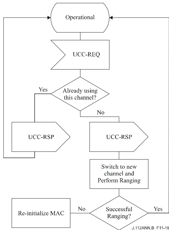
Figure B.11-19/J.112 – Changing upstream channels: CM view
