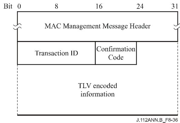
Figure B.8-36/J.112 – Dynamic Service Change-Acknowledge
