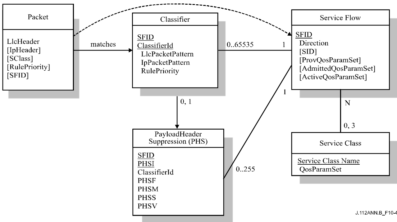
Figure B.10-4/J.112 – Theory of Operation Object Model
