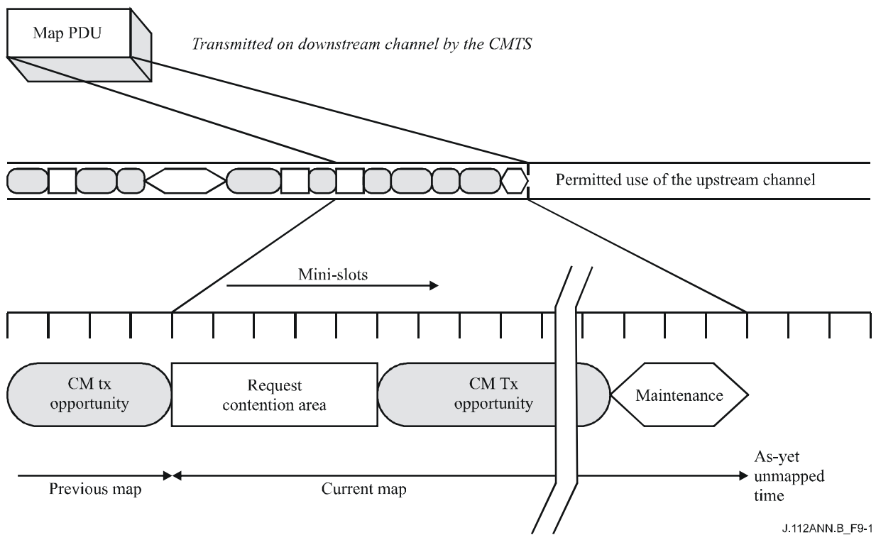
Figure B.9-1/J.112 – Allocation MAP
