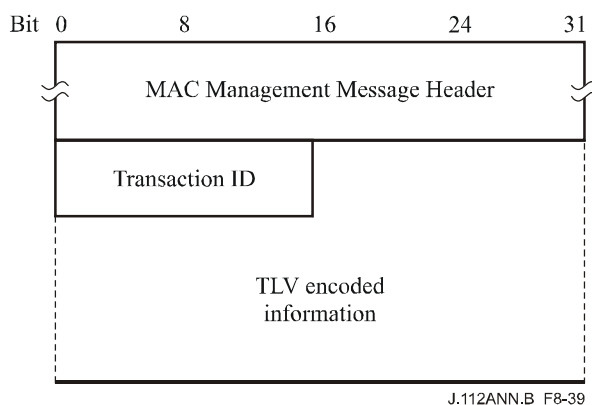
Figure B.8-39/J.112 – Dynamic Channel Change-Request
