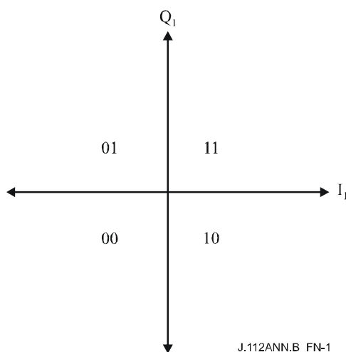
Figure B.N-1/J.112 – QPSK symbol mapping
