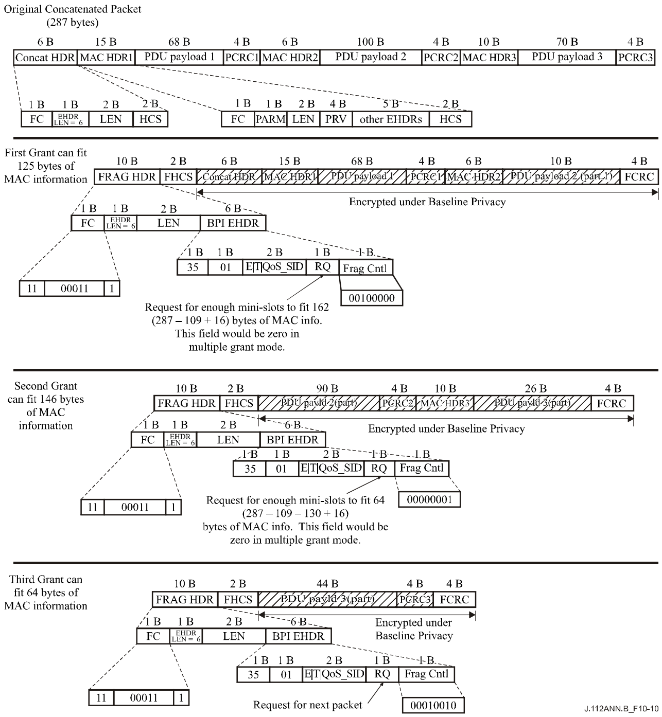
Figure B.10-10/J.112 – Example of a fragmented concatenated packet
