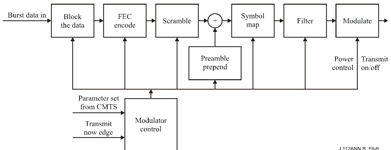
Figure B.6-9/J.112 – Signal-processing sequence
