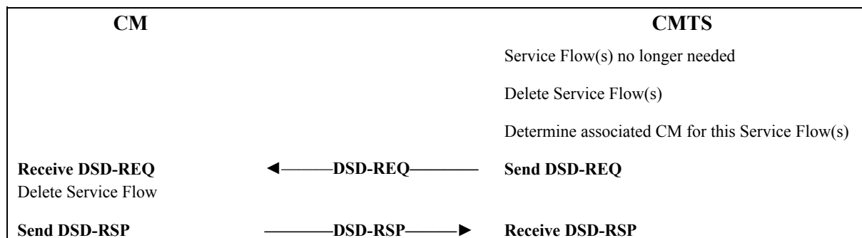
Figure B.11-51/J.112 – Dynamic Service Deletion initiated from CMTS
