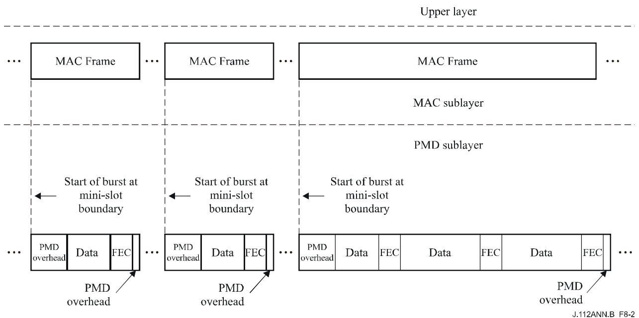
Figure B.8-2/J.112 – Upstream MAC/PMD convergence
