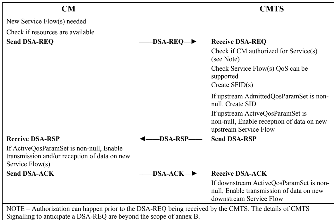
Figure B.11-28/J.112 – Dynamic Service Addition initiated from CM
