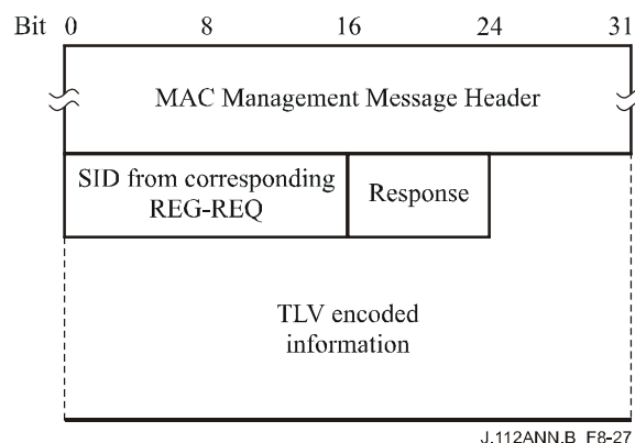
Figure B.8-27/J.112 – Registration-Response format
