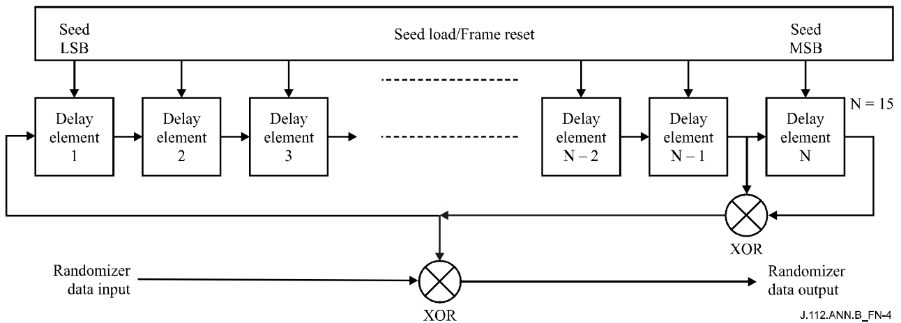
Figure B.N-4/J.112 – Scrambler structure
