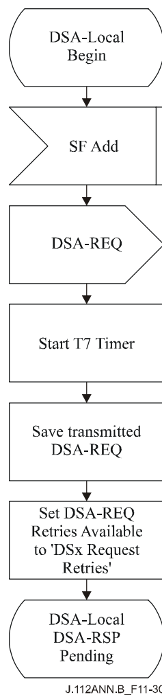
Figure B.11-30/J.112 – DSA – Locally initiated Transaction Begin State Flow Diagram
