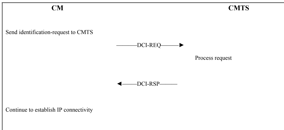
Figure B.11-9/J.112 – Device class identification
