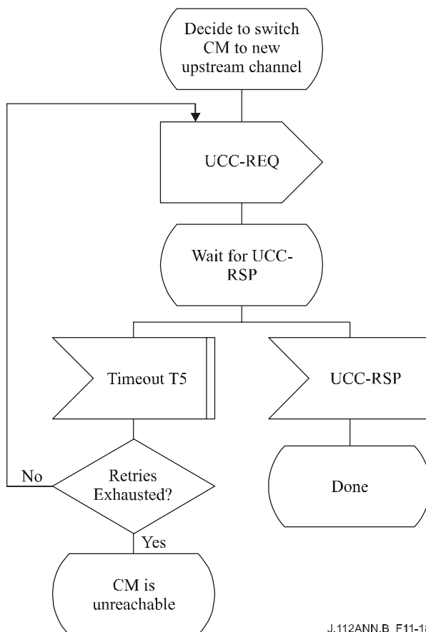
Figure B.11-18/J.112 – Changing upstream channels: CMTS view
