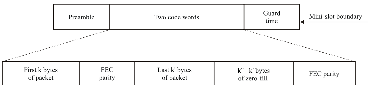
Figure B.N-8/J.112 – Example frame structures with flexible burst length mode
