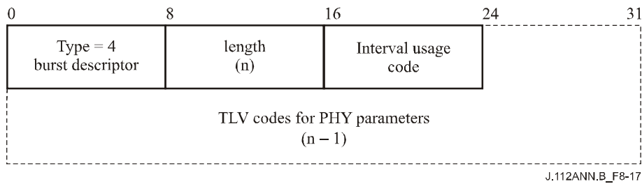
Figure B.8-17/J.112 – Top-Level Encoding for a Burst Descriptor
