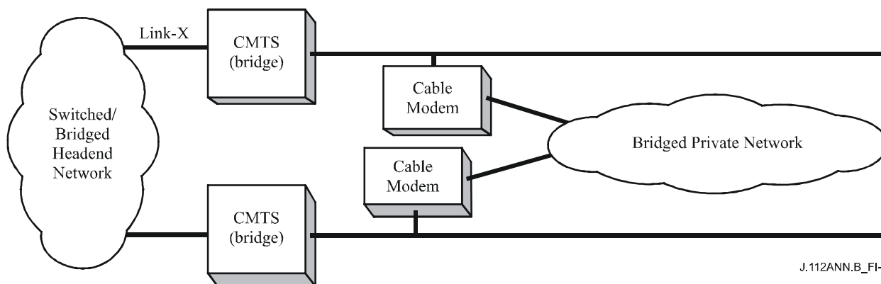
Figure B.I-2/J.112 – Spanning tree across CMTSs
