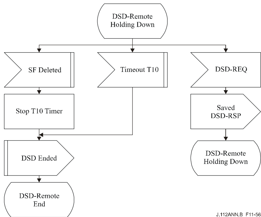
Figure B.11-56/J.112 – DSD – Remotely initiated Transaction Holding Down State Flow Diagram
