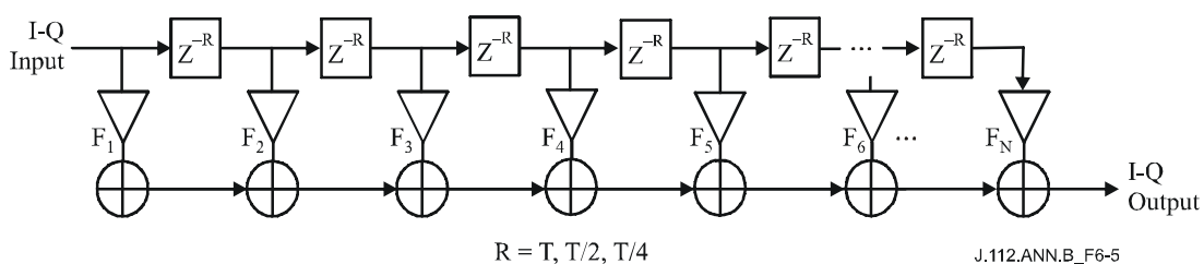
Figure B.6-5/J.112 – Transmit pre-equalizer structure
