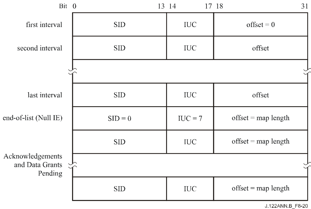
Figure B.8-20/J.112 – MAP Information Element structure
