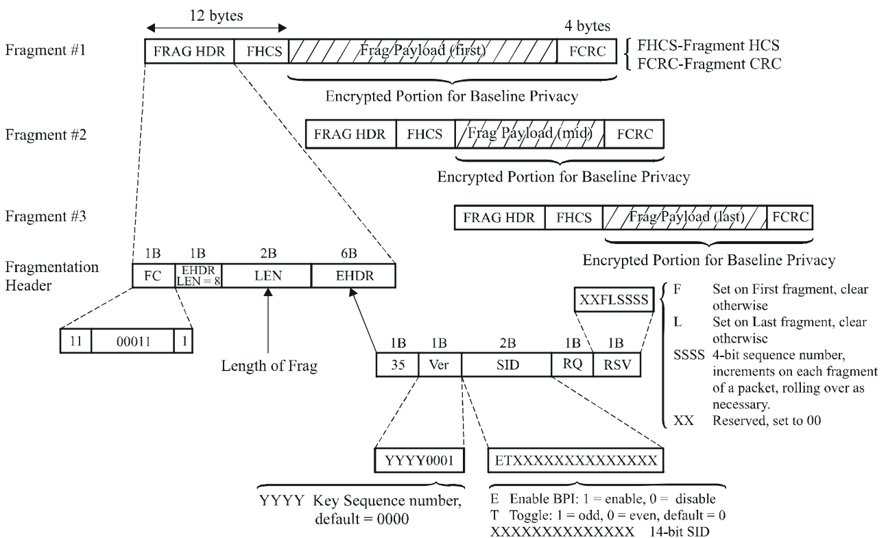
Figure B.8-13/J.112 – Fragmentation details
