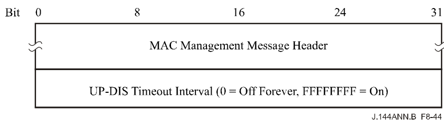
Figure B.8-44/J.112 – UP-DIS message format
