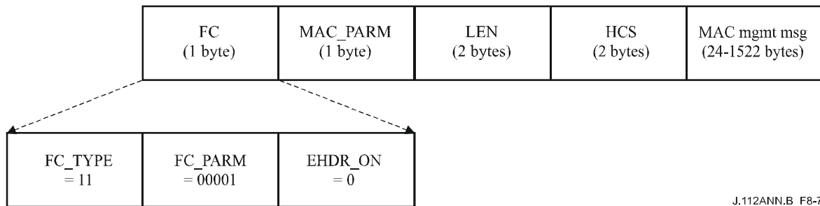
Figure B.8-7/J.112 – Management MAC Header
