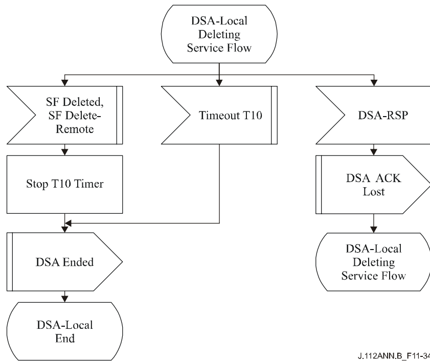
Figure B.11-34/J.112 – DSA – Locally initiated Transaction Deleting Service Flow State Flow Diagram
