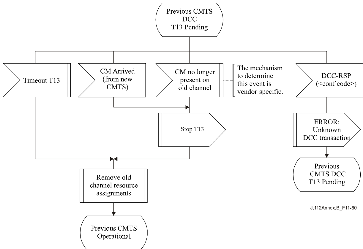
Figure B.11-60/J.112 – Dynamically Changing Channels: CMTS view, Part 3
