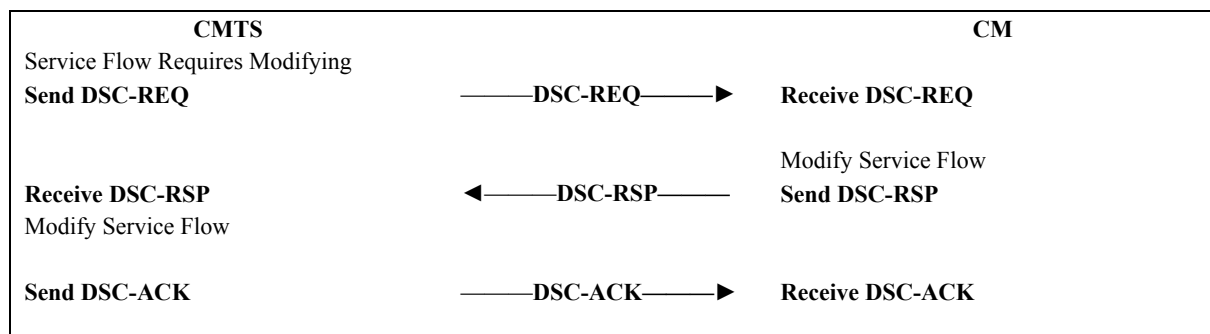
Figure B.11-40/J.112 – CMTS-initiated DSC
