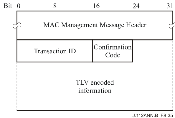
Figure B.8-35/J.112 – Dynamic Service Change-Response
