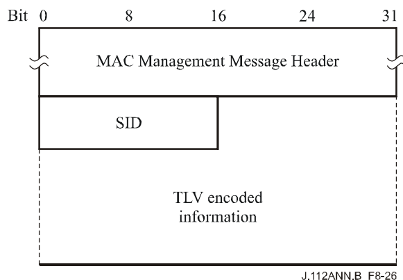
Figure B.8-26/J.112 – Registration-Request
