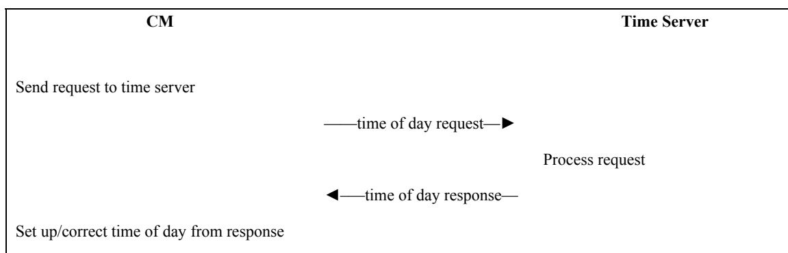
Figure B.11-11/J.112 – Establishing Time of Day
