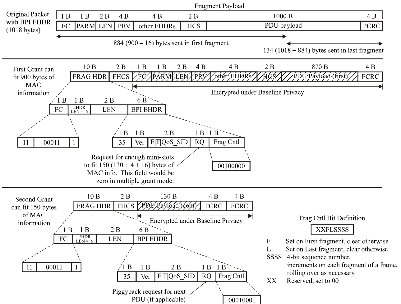
Figure B.10-9/J.112 – Example of fragmenting a single packet
