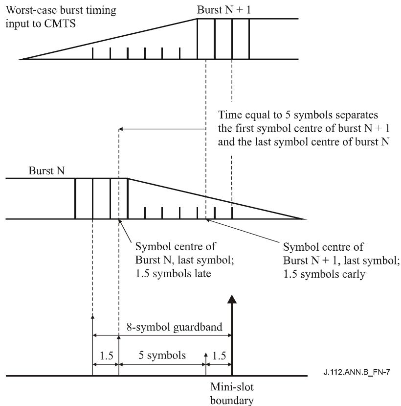
Figure B.N-7/J.112 – Worst-case burst timing
