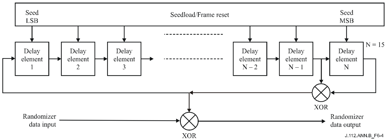
Figure B.6-4/J.112 – Scrambler structure
