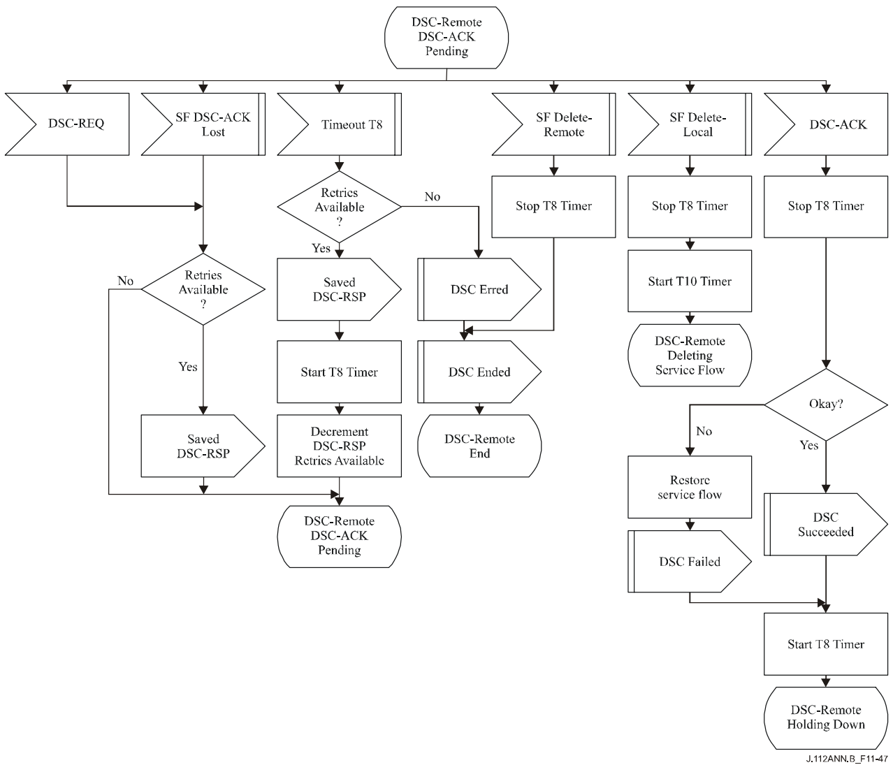
Figure B.11-47/J.112 – DSC – Remotely initiated Transaction DSC-ACK Pending State Flow Diagram
