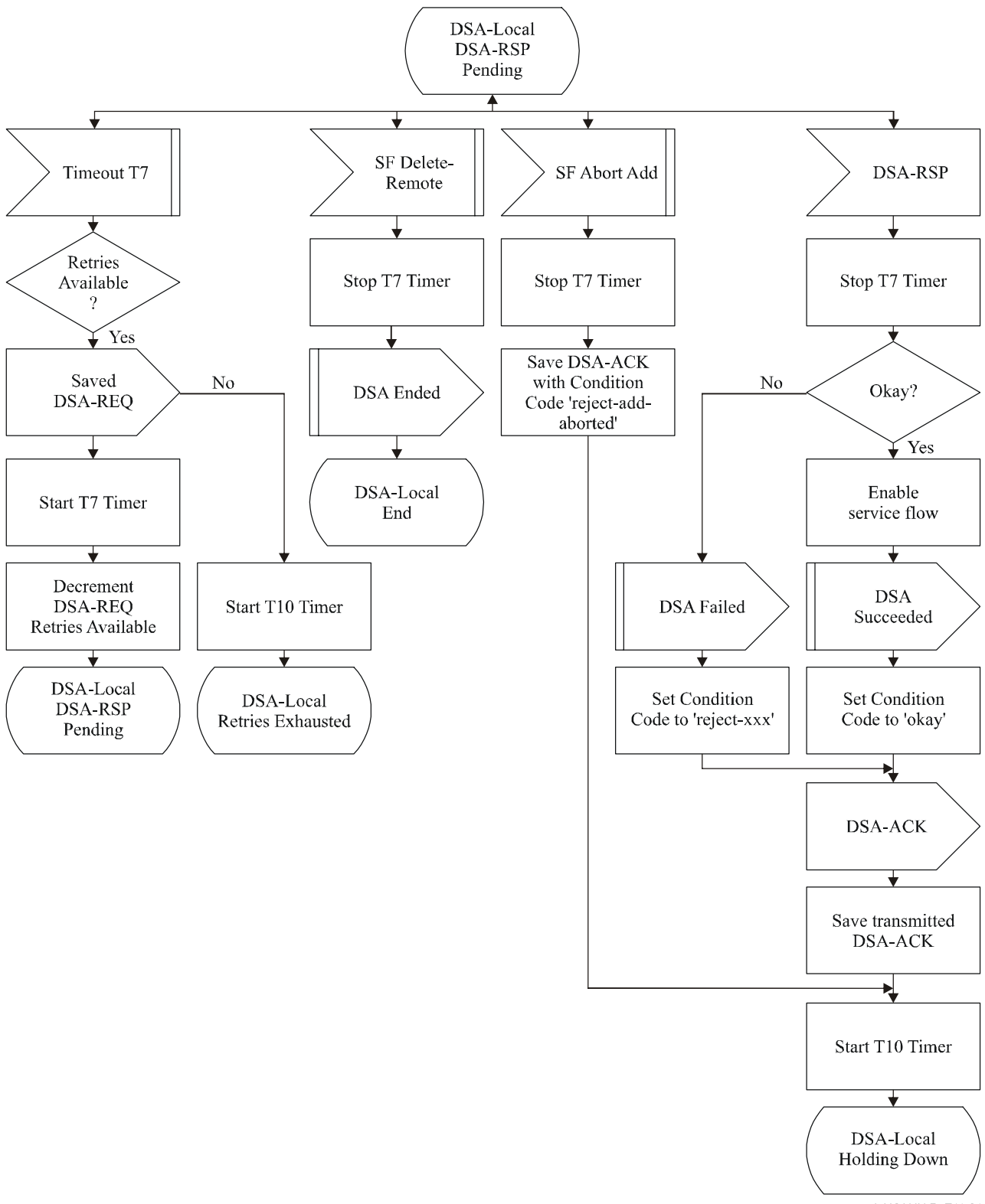
Figure B.11-31/J.112 – DSA – Locally initiated Transaction DSA-RSP Pending State Flow Diagram
