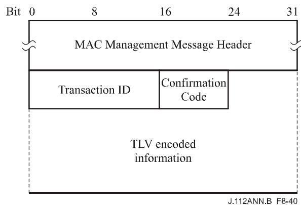
Figure B.8-40/J.112 – Dynamic Channel Change-Response
