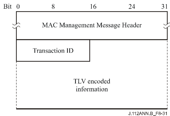
Figure B.8-31/J.112 – Dynamic Service Addition-Request
