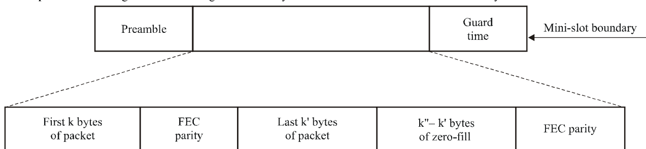
Figure B.6-8/J.112 – Example frame structures with flexible burst length mode
