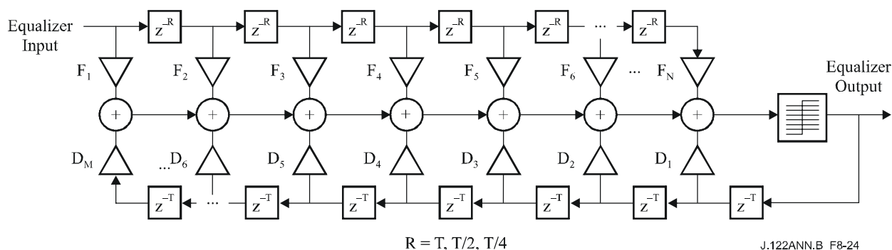
Figure B.8-24/J.112 – Generalized equalizer tap location definition
