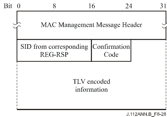
Figure B.8-28/J.112 – Registration-Acknowledgment
