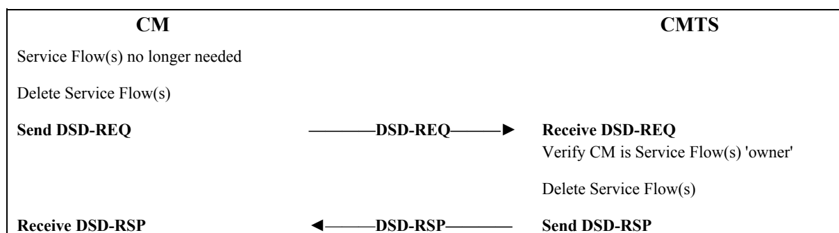
Figure B.11-50/J.112 – Dynamic Service Deletion initiated from CM
