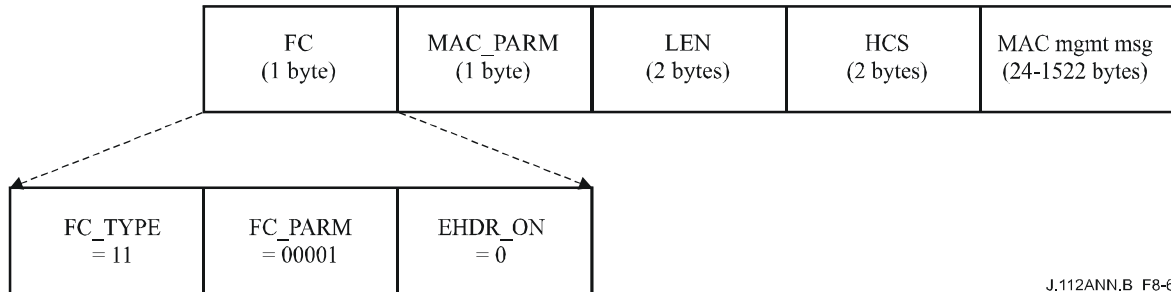
Figure B.8-6/J.112 – Timing MAC Header
