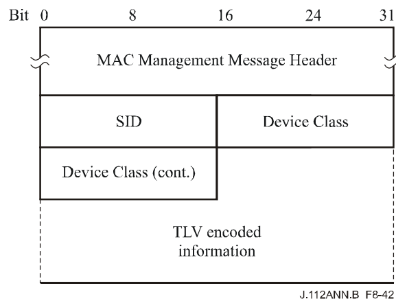
Figure B.8-42/J.112 – Device Class Identification-Request
