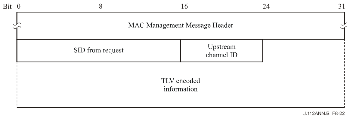
Figure B.8-22/J.112 – Ranging-Response
