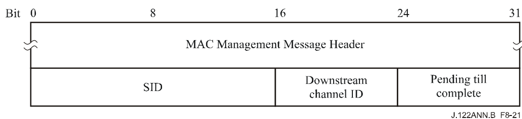
Figure B.8-21/J.112 – Packet PDU following the Timing Header
