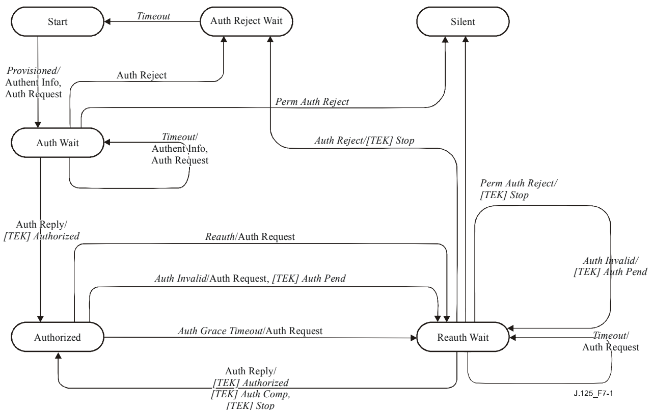
Figure 7-1/J.125 – Authorization state machine flow diagram
