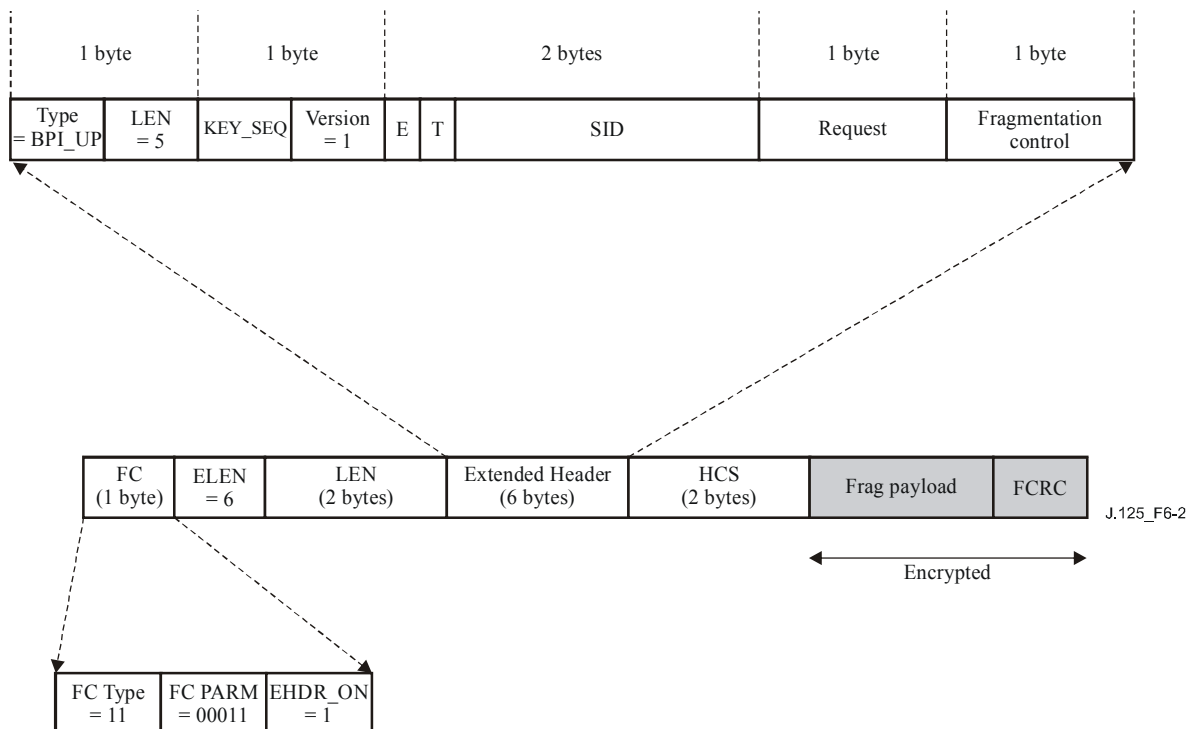
Figure 6-2/J.125 – Format of a DOCSIS MAC fragmentation frame with an encrypted payload
