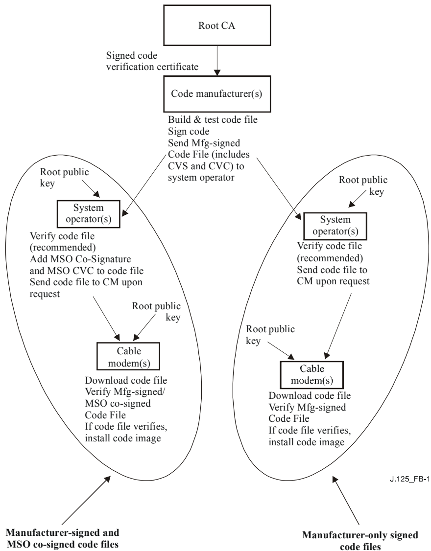
Figure B.1/J.125 – Typical code validation hierarchy
