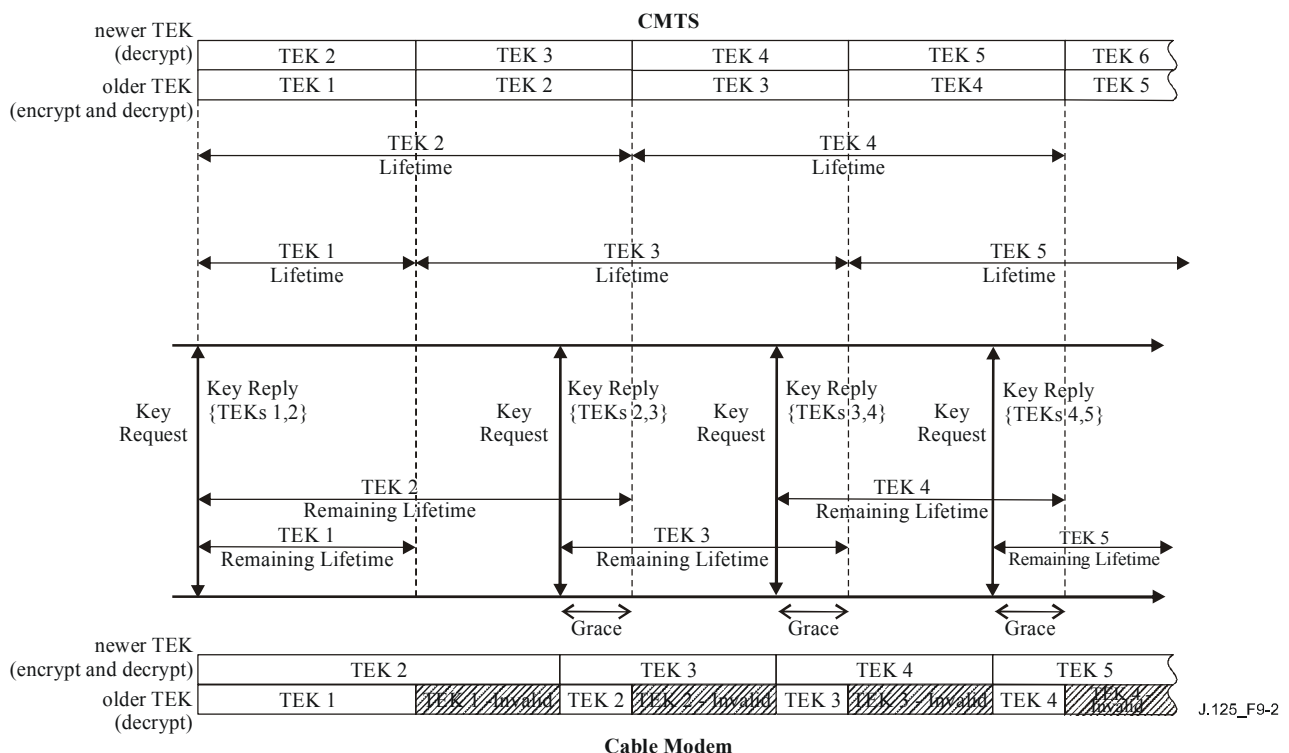
Figure 9-2/J.125 – TEK management in CMTS and CM
