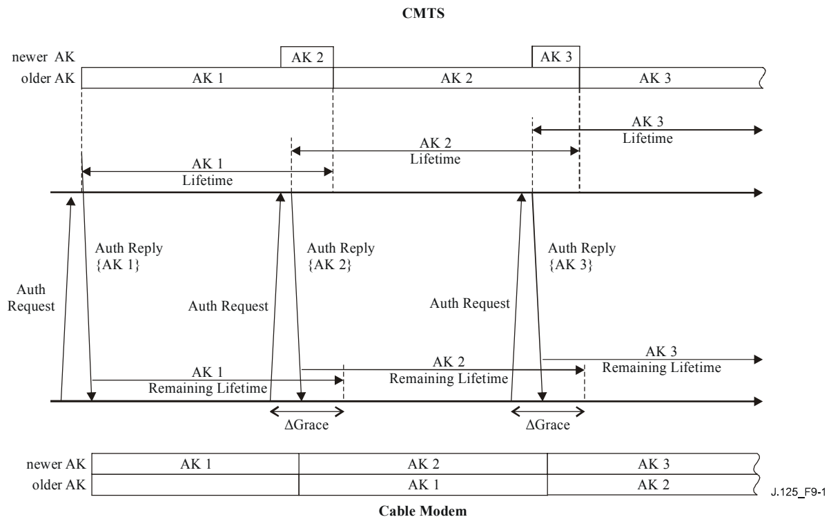
Figure 9-1/J.125 – Authorization key management in CMTS and CM
