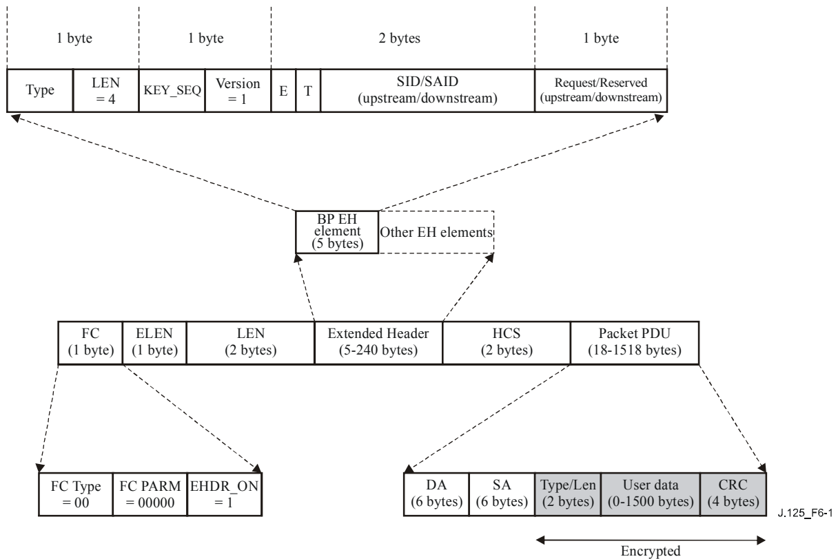
Figure 6-1/J.125 – Format of DOCSIS variable-length packet data PDU with privacy EH element
