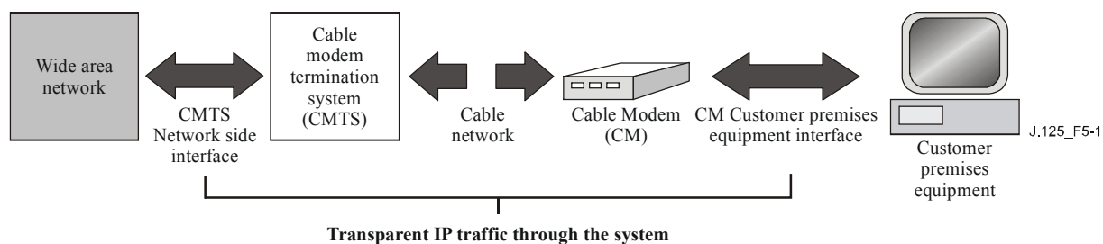
Figure 5-1/J.125 – Transparent IP traffic through the data-over-cable system
