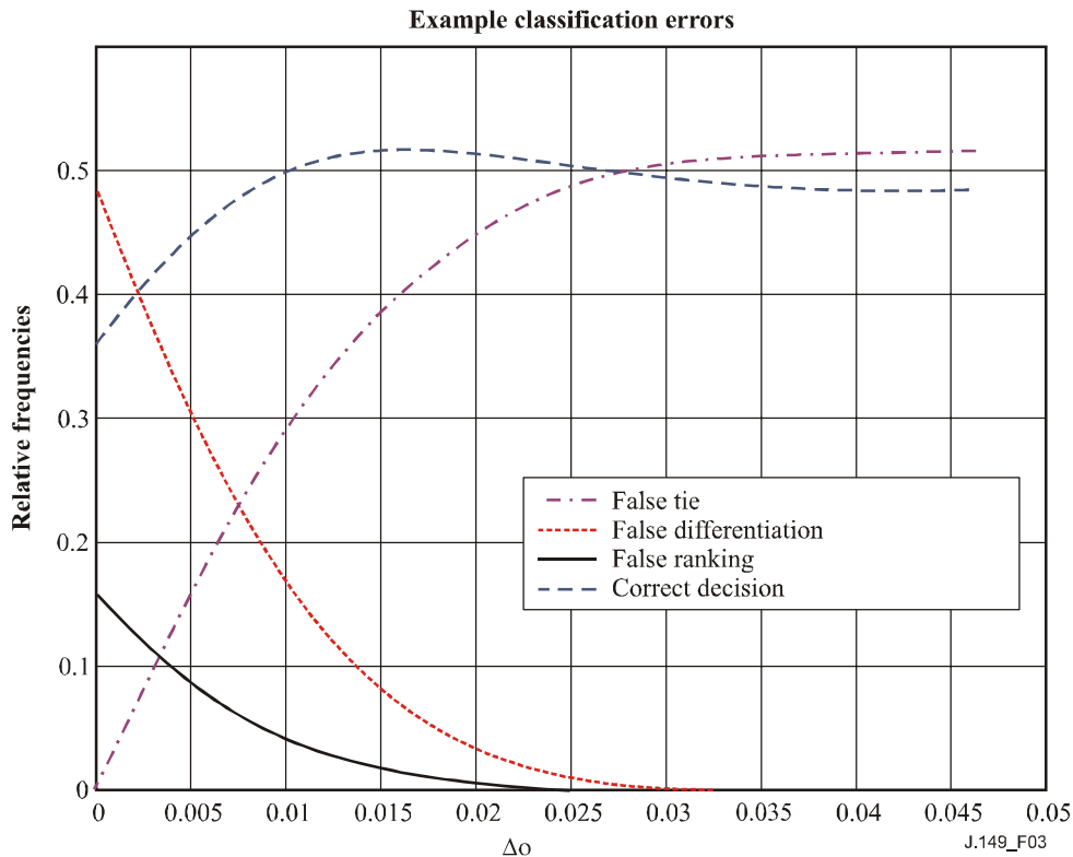
Figure 3 – Sample plot of frequencies of classification error
