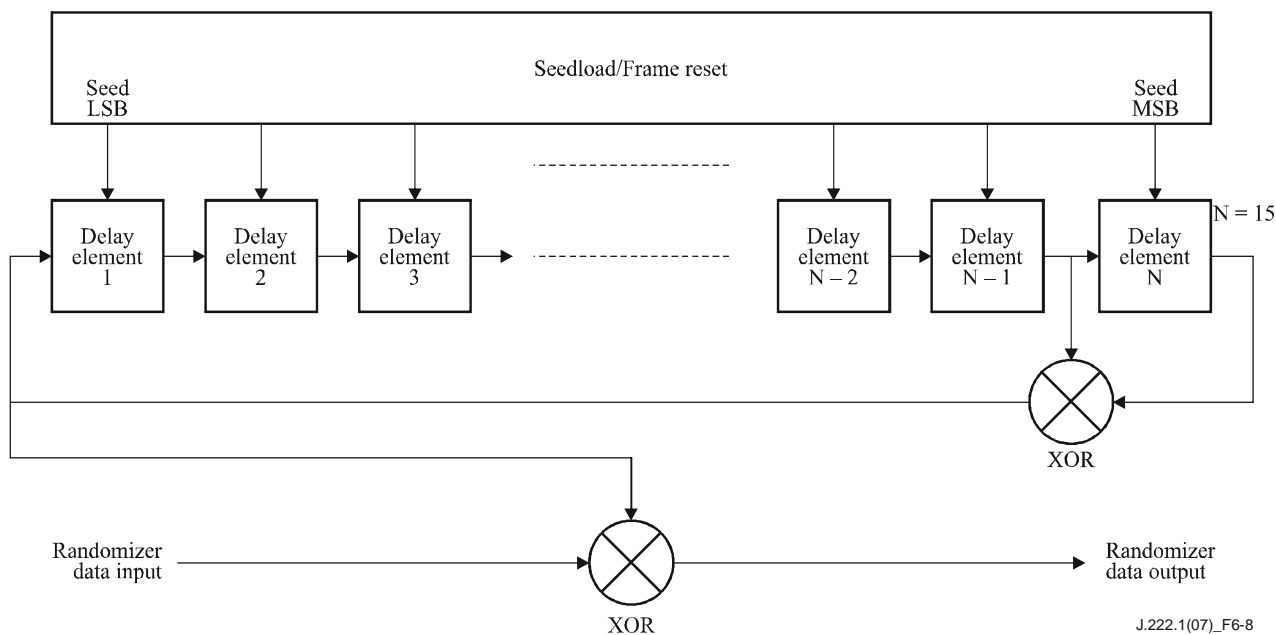
Figure 6-8 – Scrambler structure
