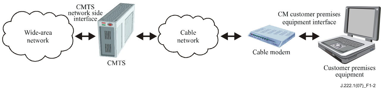
Figure 1-2 – Transparent IP traffic through the data-over-cable system
