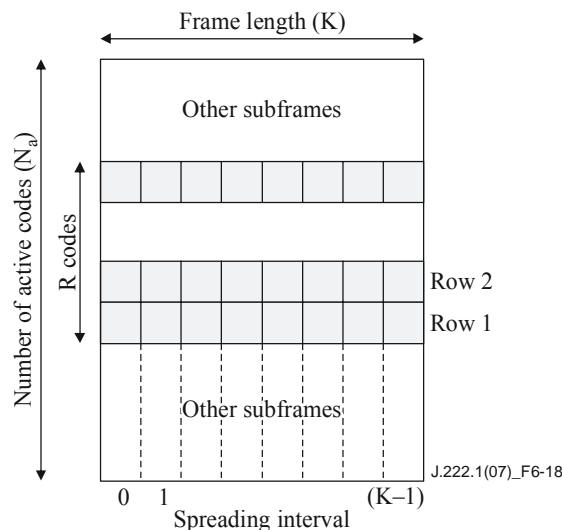
Figure 6-18 – Subframe structure
