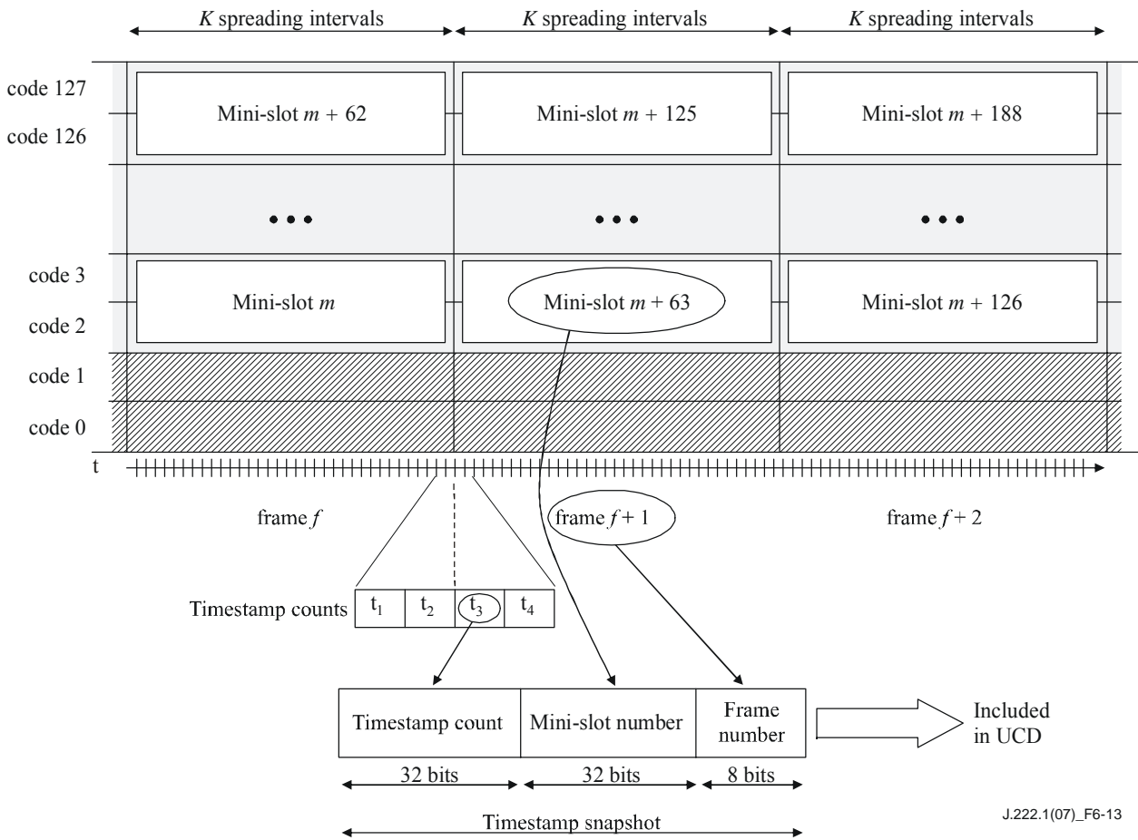
Figure 6-13 – Timestamp snapshot
