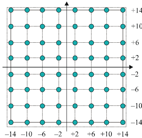
Figure 6-20 – Symbol constellations
