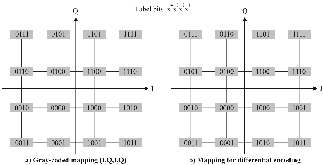
Figure 6-23 – 16 QAM symbol mapping
