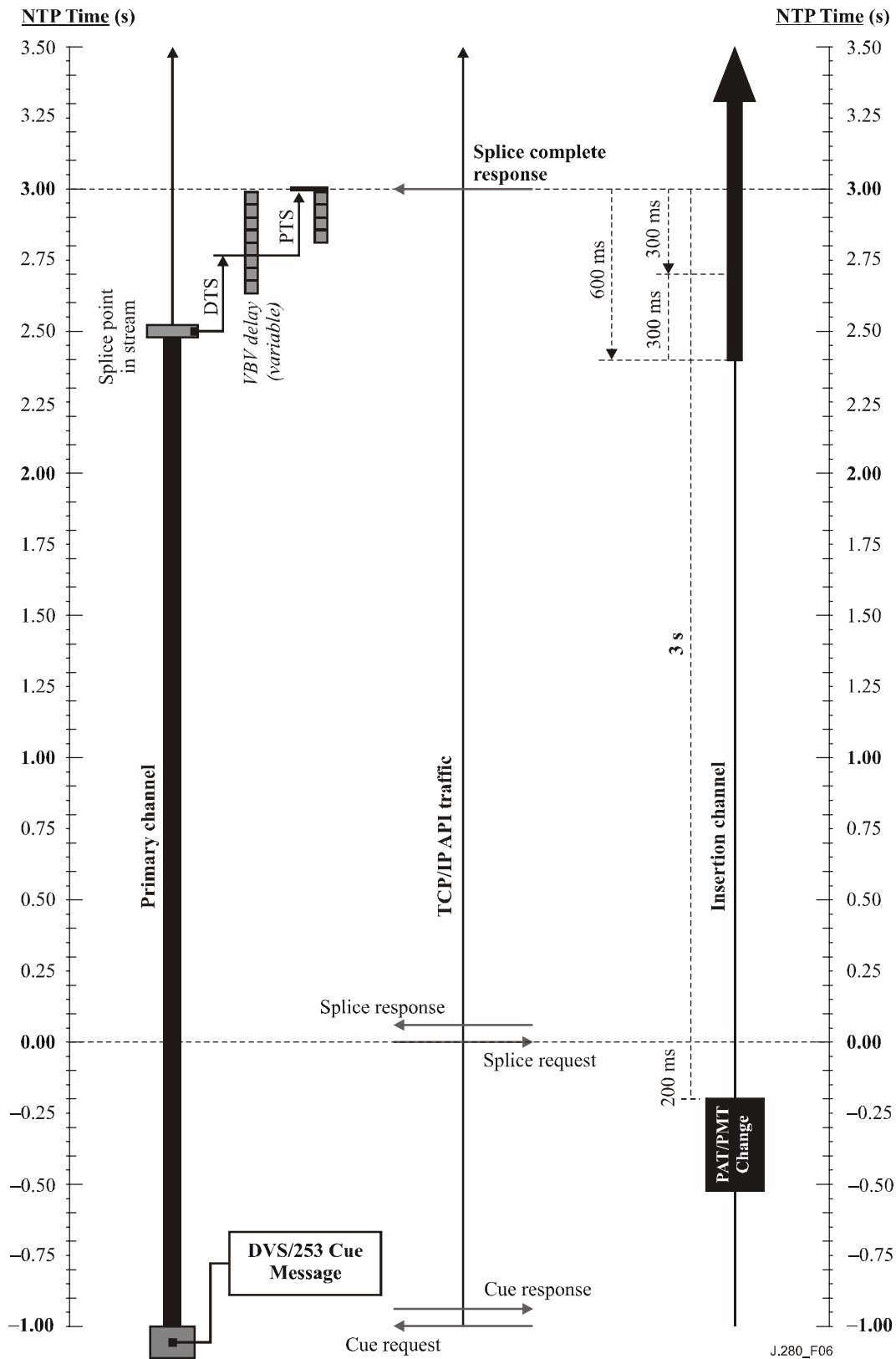
Figure 6/J.280 – DPI splice initiation timeline
