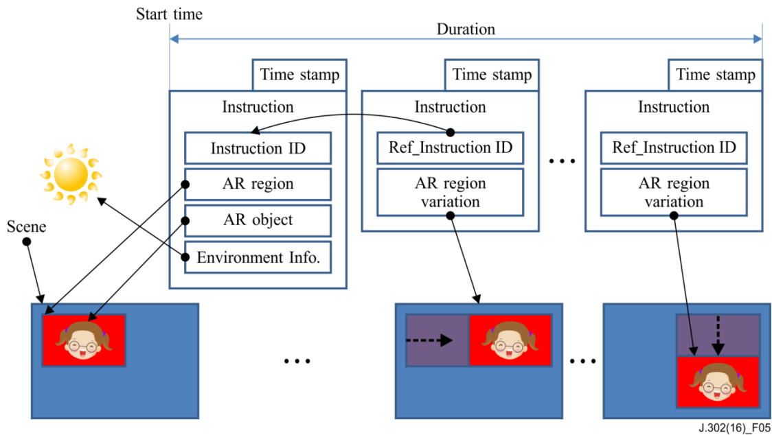
Figure 5 – Streaming strategy for AR-STV metadata
