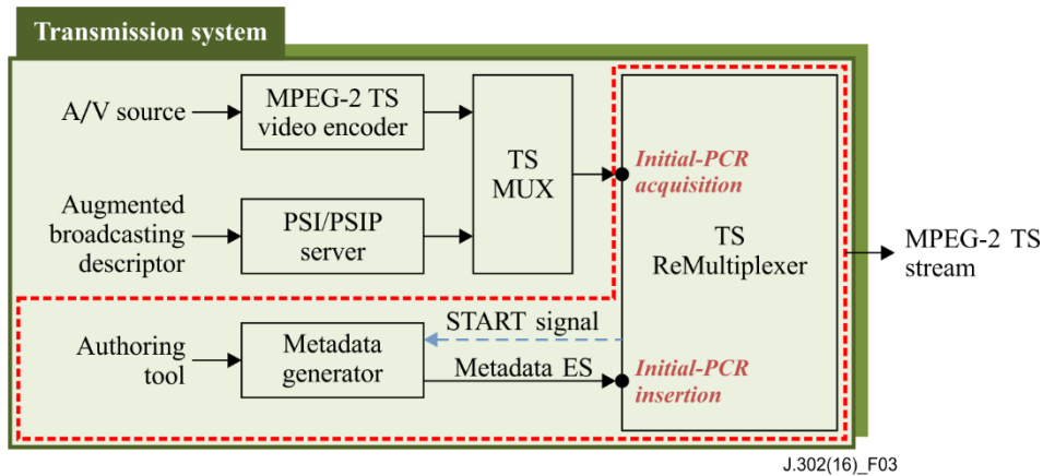
Figure 3 – Structure of transmission system for AR-STV
