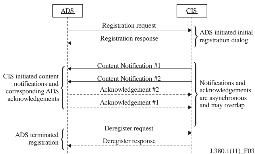
Figure 3 – Typical message sequence diagram
