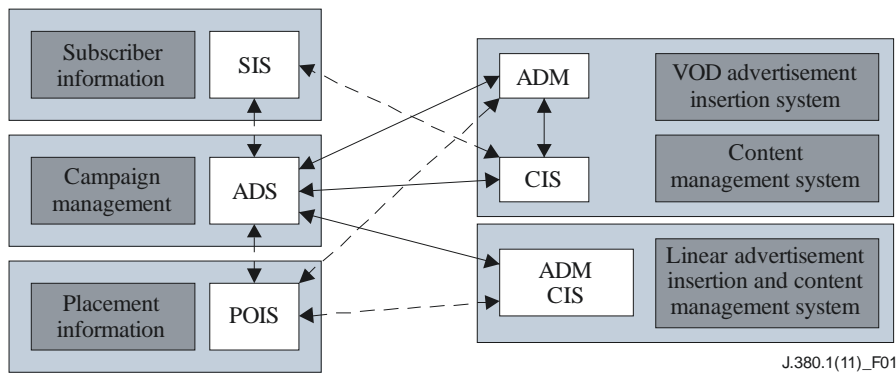
Figure 1 – Example advertising system services configuration
