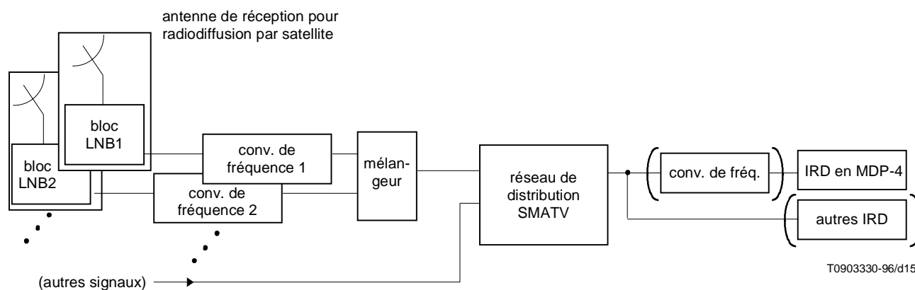
Figure C.2/J.84 – Système SMATV C(II)
