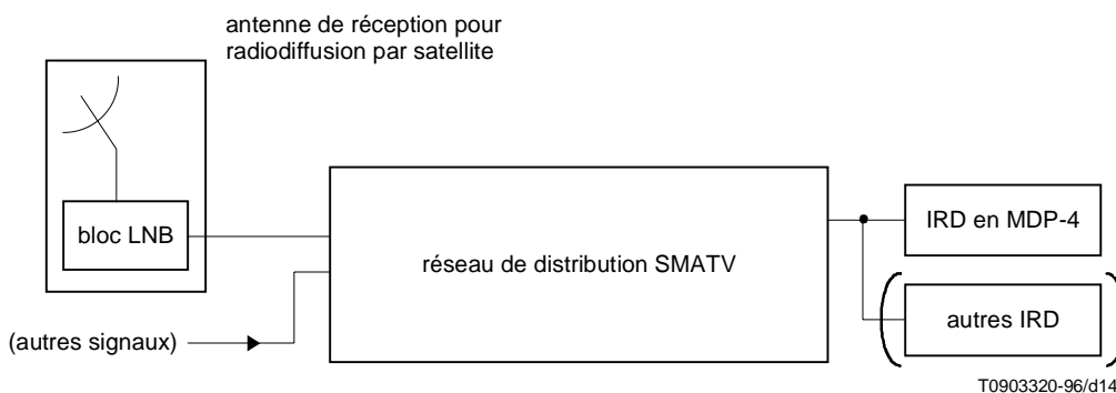
Figure C.1/J.84 – Système SMATV C(I)
