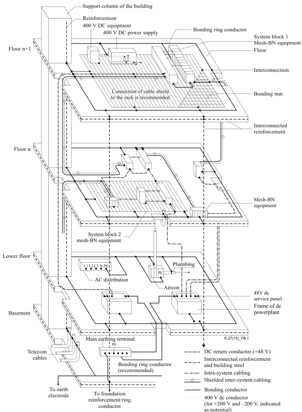
Figure B.1 – Mesh-BN installation inside a telecommunication building
