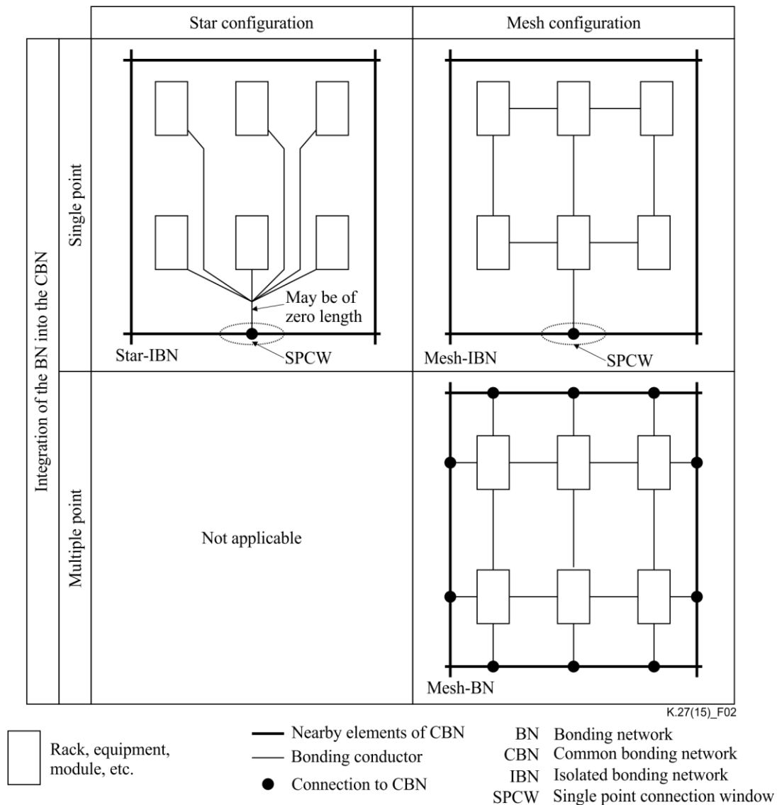
Figure 2 – Connection of system block to the CBN
