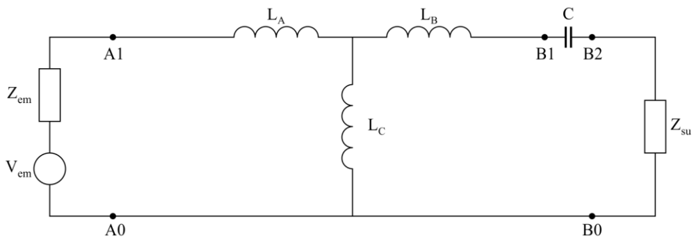
c) Shielding model for CBN-IBN coupling
