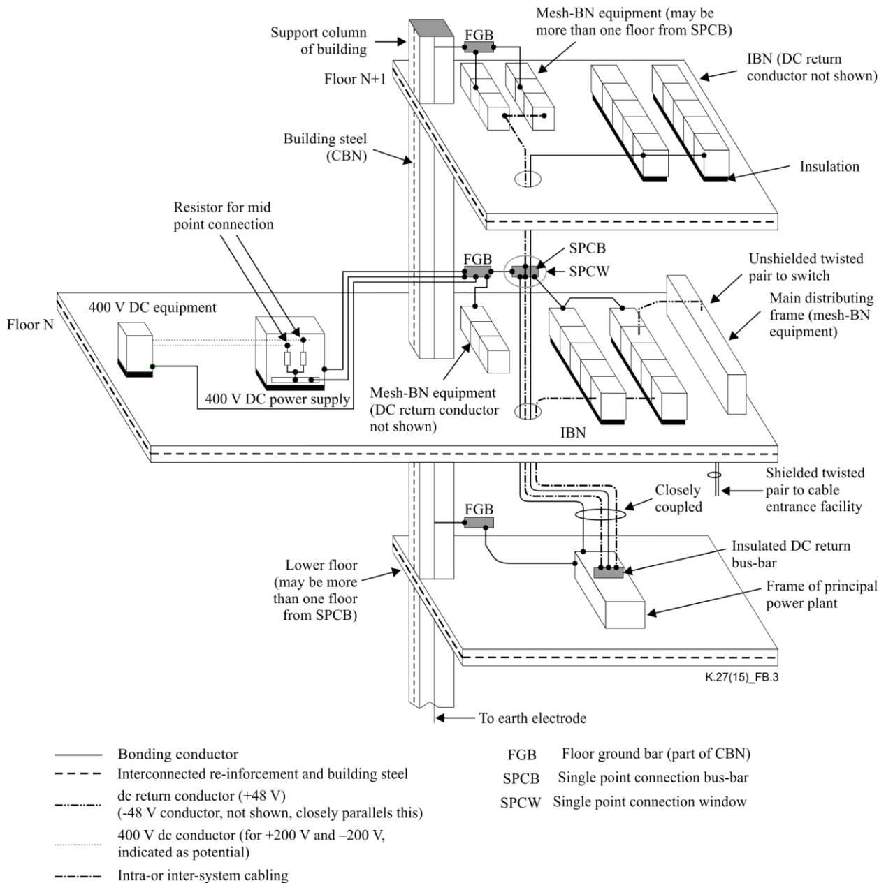
Figure B.3 – Star-IBN with isolation of DC power return
