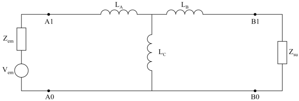
b) Shielding model for intra-CBN coupling
