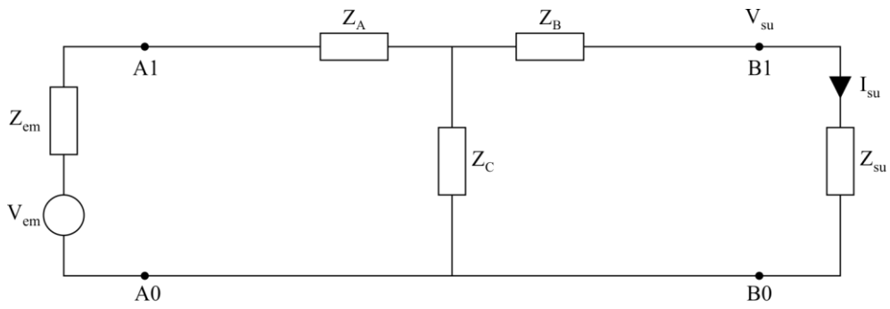
a) Fundamental shielding model
