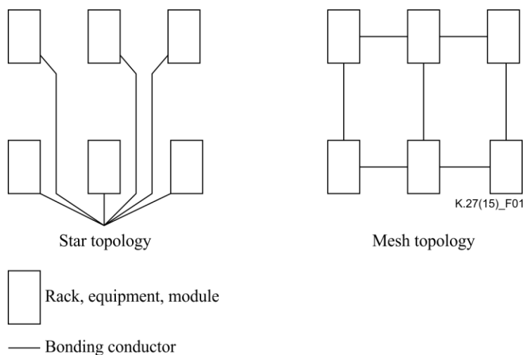
Figure 1 – Bonding network configurations forming a system block
