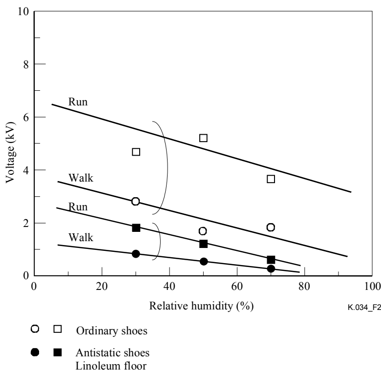
Figure 2/K.34 – Maximum value of electrostatic voltage to which operators may be charged in telecommunication central office
