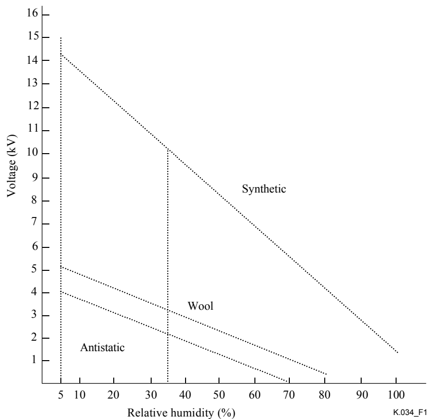
Figure 1/K.34 – Maximum values of electrostatic voltages to which operators may be charged while in contact with the materials in the absence of any electrostatic protection measures
