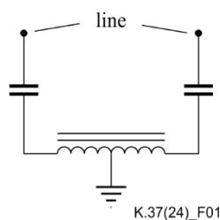
Figure 1 – Drainage coil
