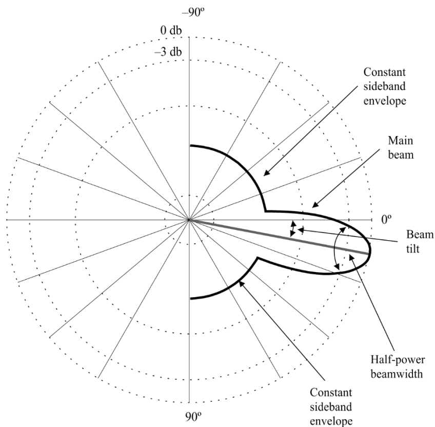
Figure B.7 – Illustration of terms relating to antenna patterns
