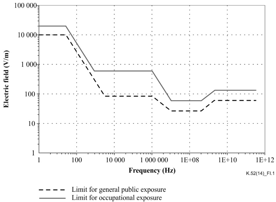
Figure I.1 – ICNIRP reference levels for electric field strength
