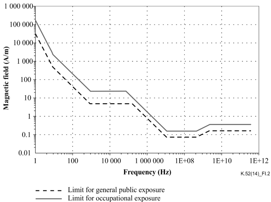
Figure I.2 – ICNIRP reference levels for magnetic field strength
