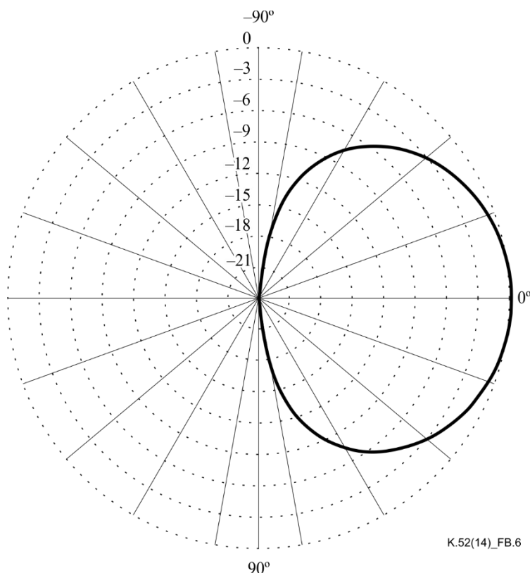
Figure B.6 – Vertical pattern for a half-wave dipole in vertical polarization
