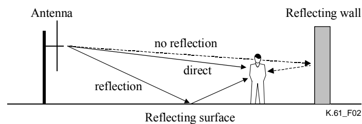
Figure 2 – An illustration of a multi-path alteration due to the presence of a human body
