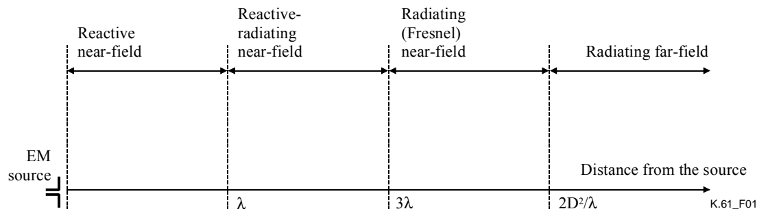
Figure 1 – Field regions around an EM source (the antenna maximum dimension D is supposed to be large compared with the wavelength \lambda )
