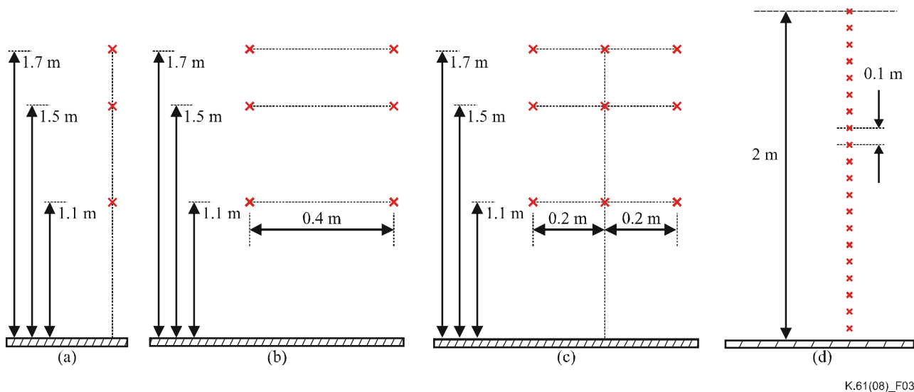
Figure 3 – Measurement points for spatial averaging
