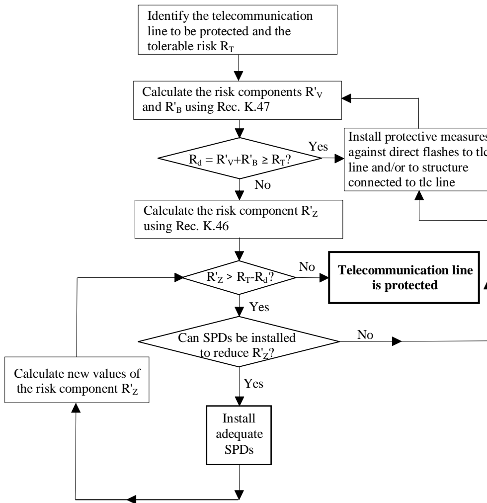
Figure 4 – Procedure for selecting protection measures in a telecommunication line
