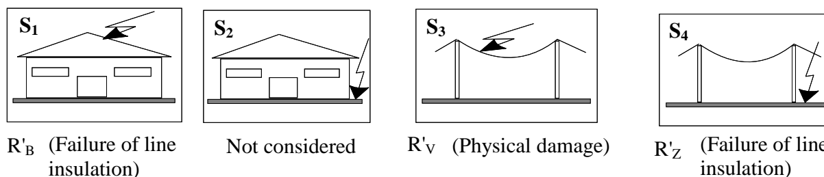
Figure 3 – Risk components causing the risk of loss of service in a telecommunication network related to each source of damage
