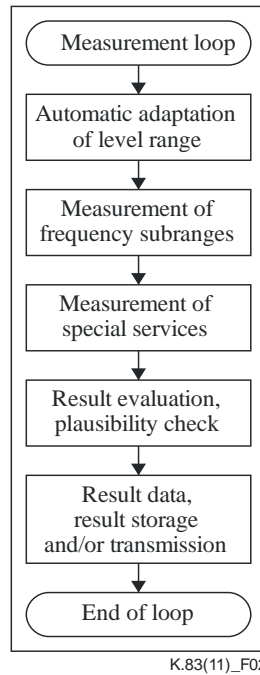
Figure 2 – Measurement loop
