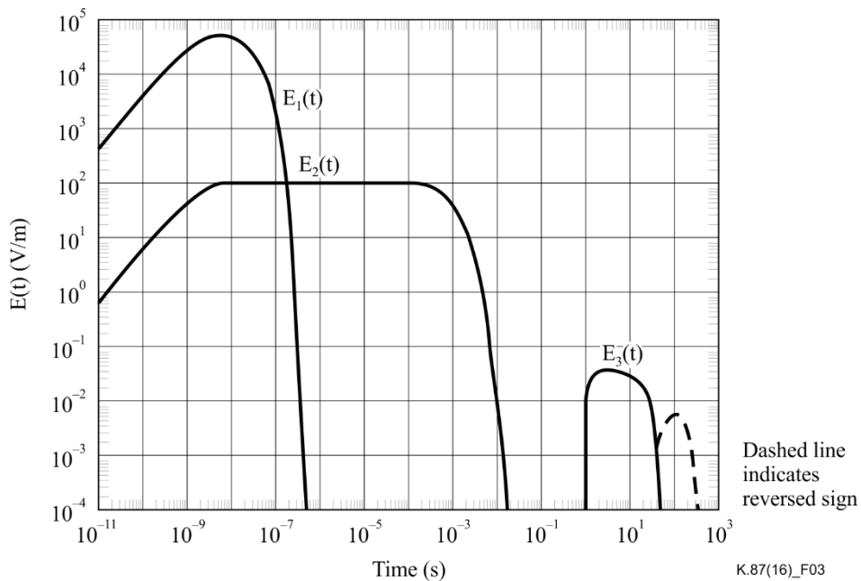
Figure 3 – Pulse characteristics
