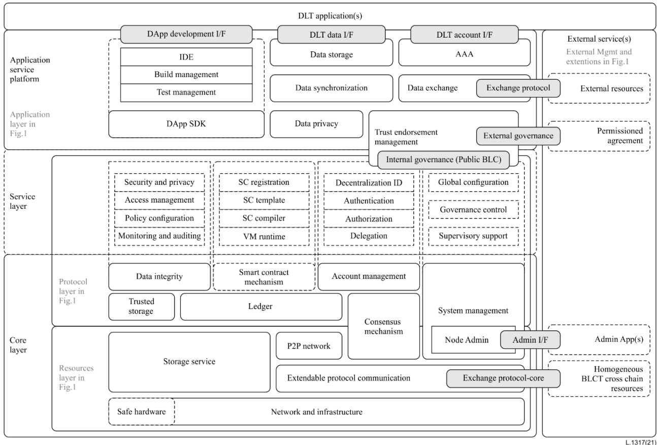
Figure 16 – Schematic diagram of the detailed architecture [ITU-T F.751.2]
