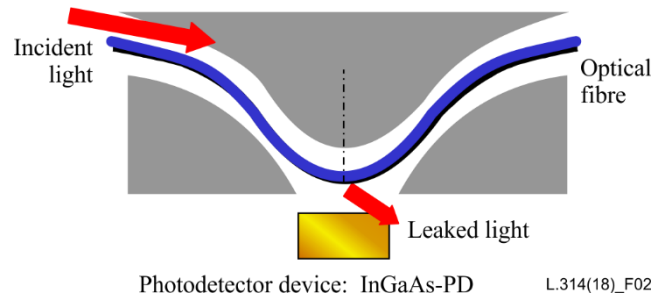
Figure 2 – Typical configuration of bent part of optical fibre identifier
