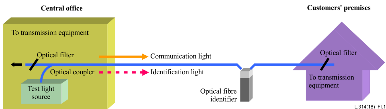
Figure I.1 – Configuration of optical fibre identification
