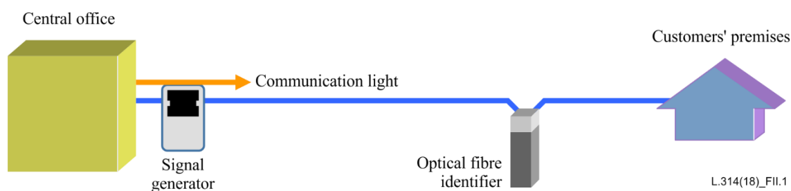
Figure II.1 – Configuration for optical fibre identification without identification light
