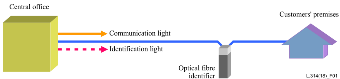
Figure 1 – Configuration for optical fibre identification
