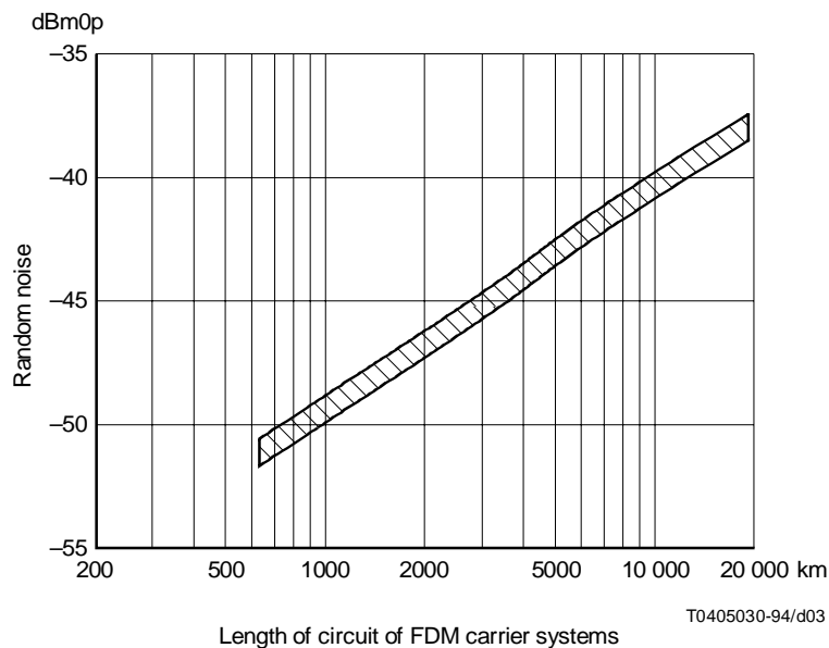
FIGURE A.1/M.1025
