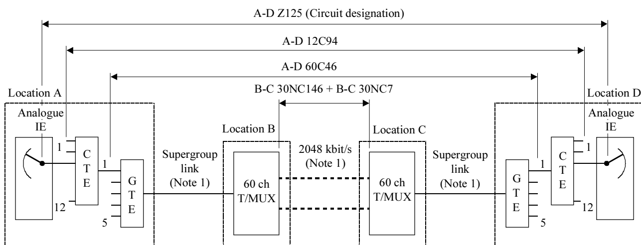
b) Analogue-digital-analogue route
