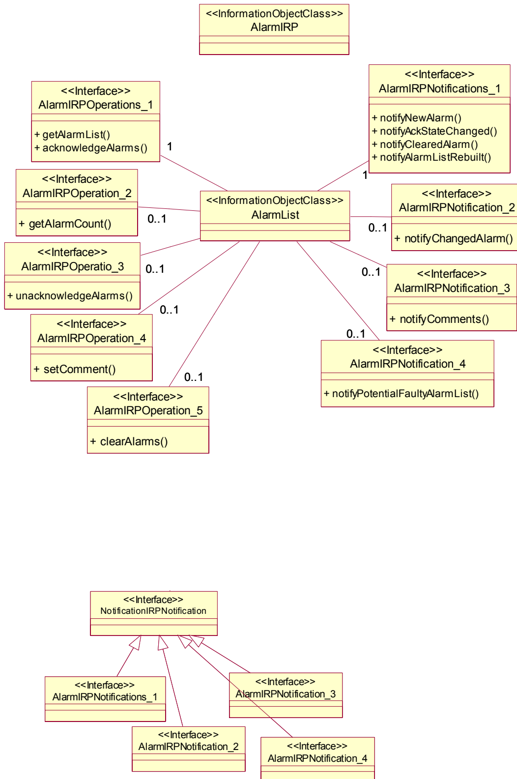
Figure II.4 – Alarm management IRP class diagram
