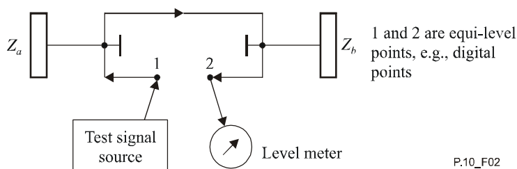
Figure 2 – Open-loop loss (OLL)
