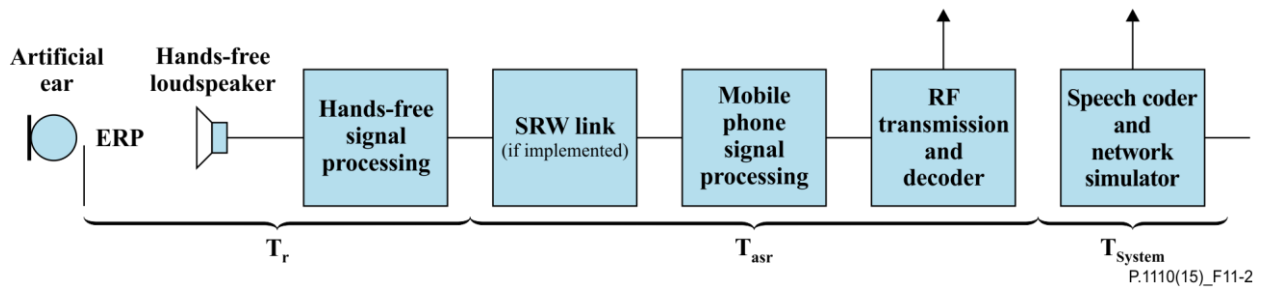
Figure 11-2 – Different blocks contributing to the delay in receive direction
