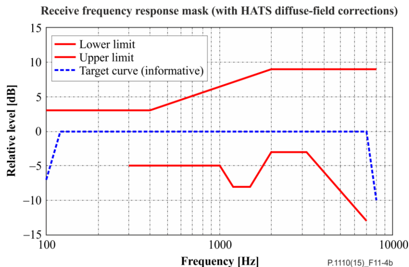
Figure 11-4b – Receive frequency response mask (with HATS diffuse-field corrections)
