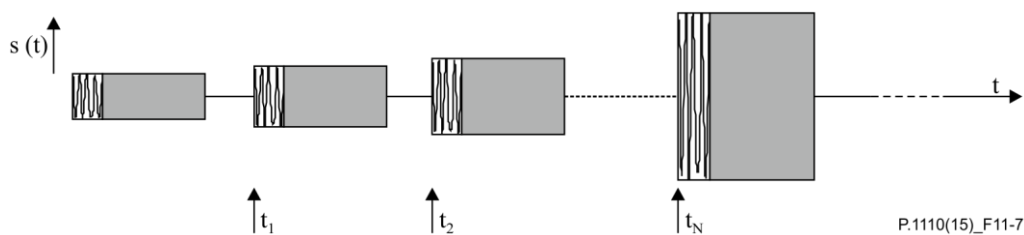
Figure 11-7 – Test signal to determine the minimum activation level and the built-up time
