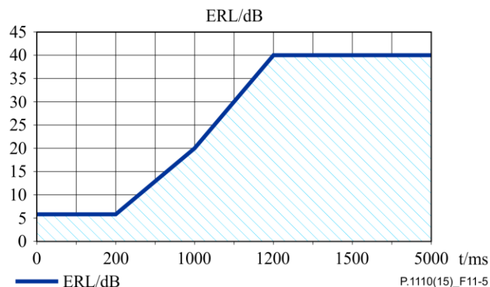
Figure 11-5 – Initial convergence, ERL vs. time
