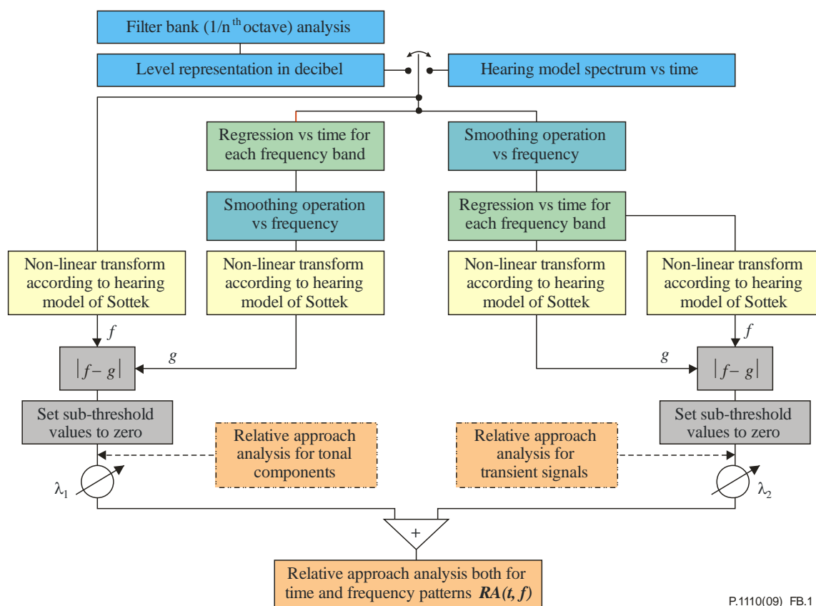
Figure B.1 – Block diagram of Relative Approach
