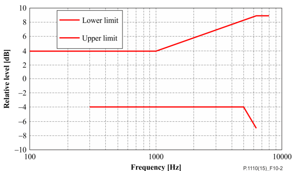
Figure 10-2 – Send frequency response mask
