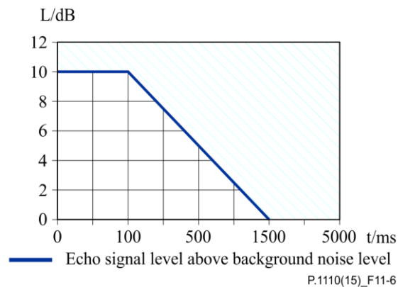
Figure 11-6 – Initial convergence with background noise, requirement on echo signal level vs. time
