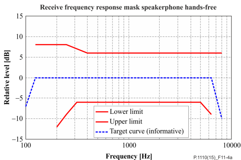
Figure 11-4a – Receive frequency response mask speakerphone hands-free
