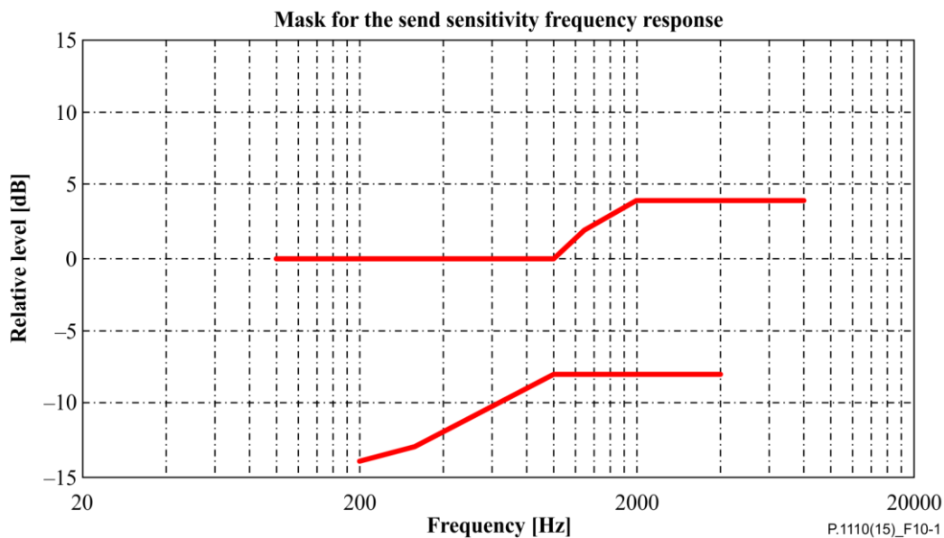
Figure 10-1 – Microphone send frequency response mask (this figure is informative)
