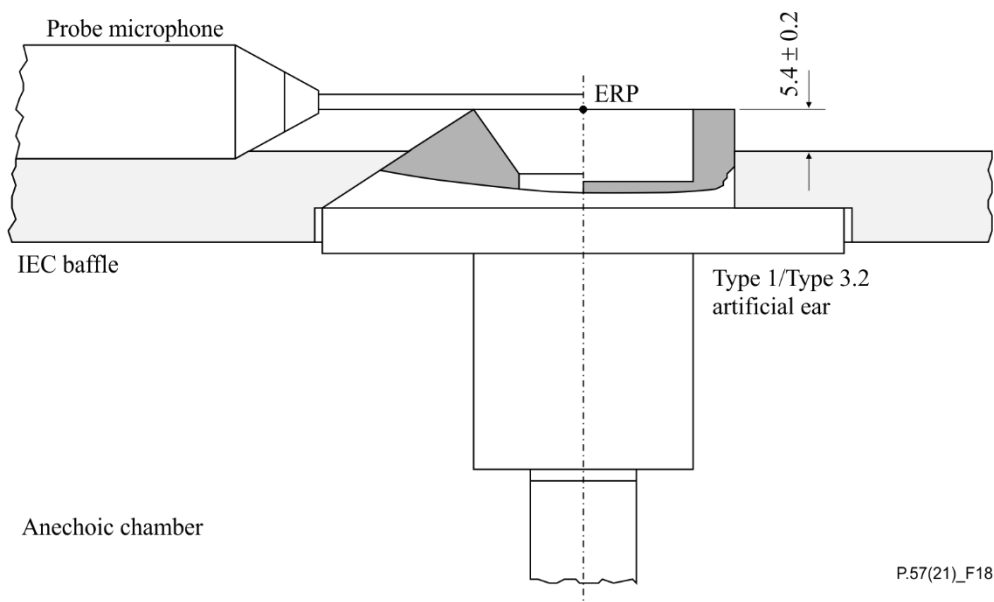
Figure 18 – Set-up for measuring the frequency sensitivity response (open ear conditions) of type 1 and type 3.2 artificial ears
