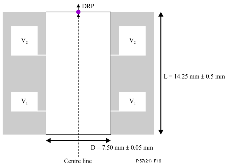
Figure 16 – Geometry of cylindrical cavity of the inner part of the ear canal
