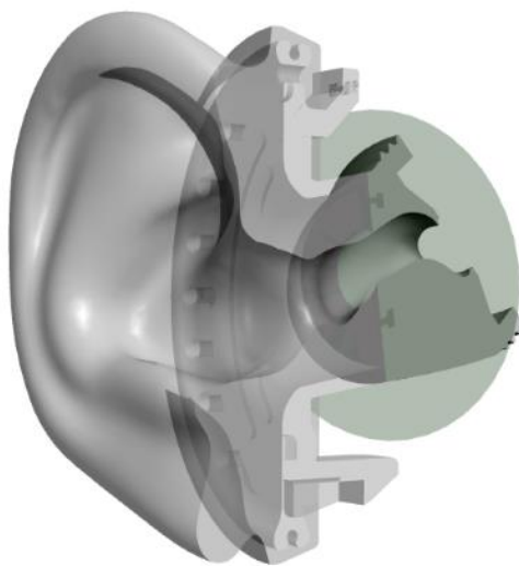
Figure 9 – The type 4.3 ear simulator, showing an average human ear canal with the type 3.3 based pinna simulator attached
