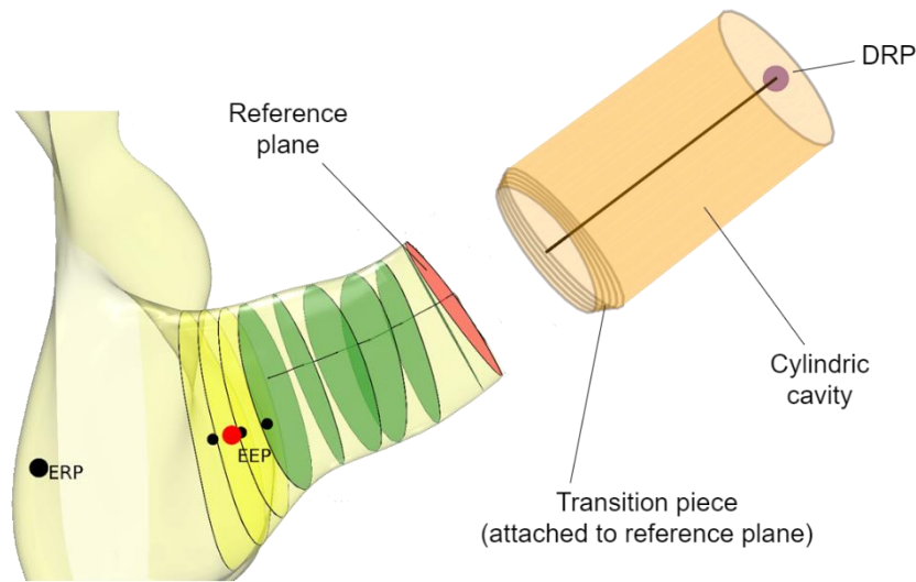
Figure 15 – Cross sectional areas of the anatomically shaped ear canal and concha bottom of the type 4.4 ear simulator
