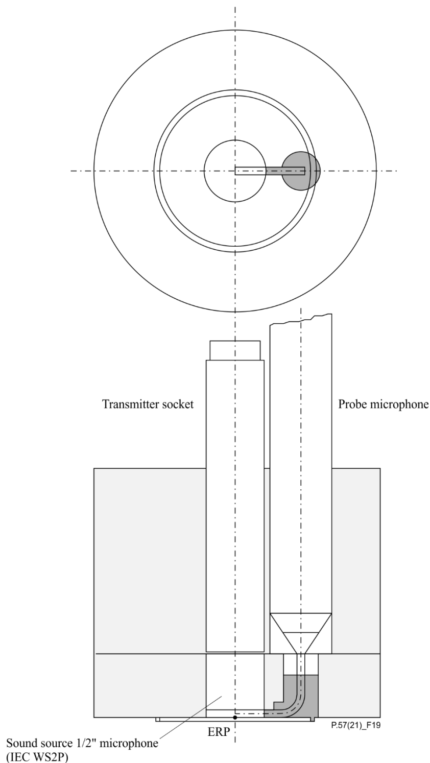
Figure 19 – Practical implementation of a calibration device (impedance probe) for measuring acoustical input impedance of type 1 and type 3.2 artificial ears
