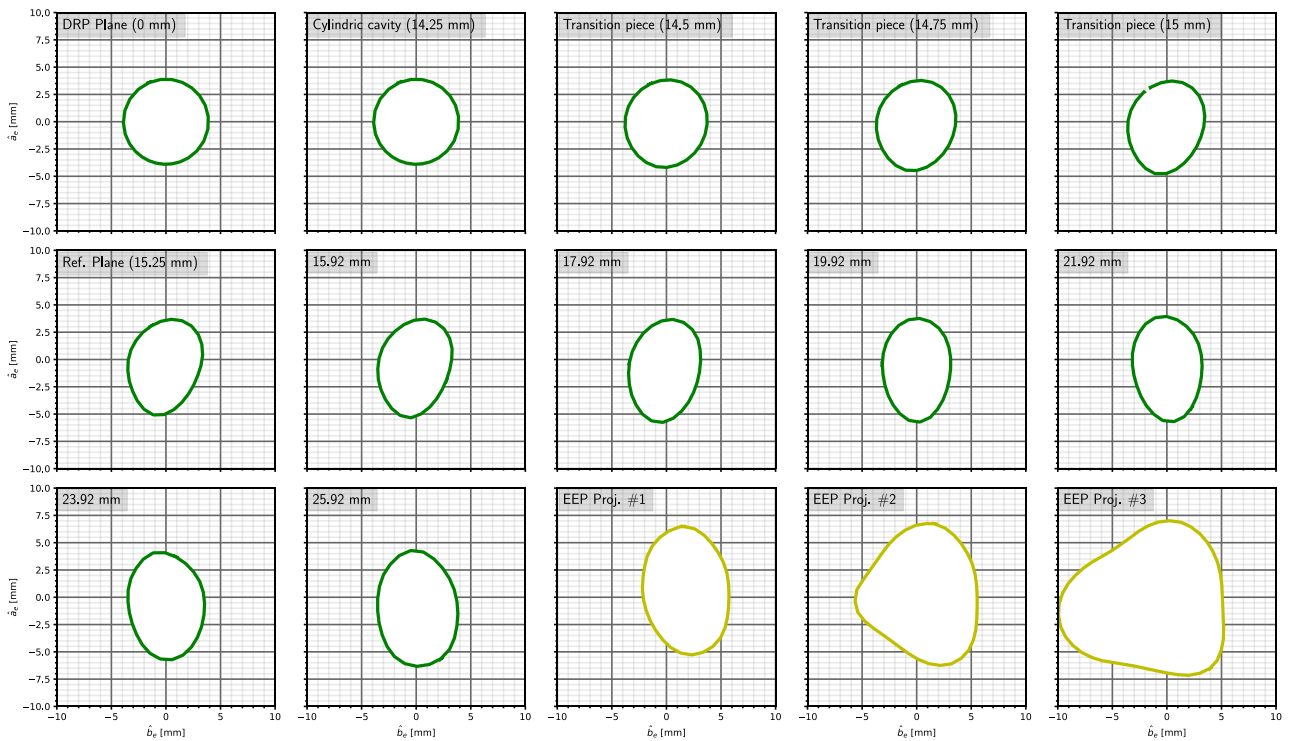
Figure 17 – Cross sectional areas in the \hat{b}_e, \hat{a}_e plane of the two unit vectors
