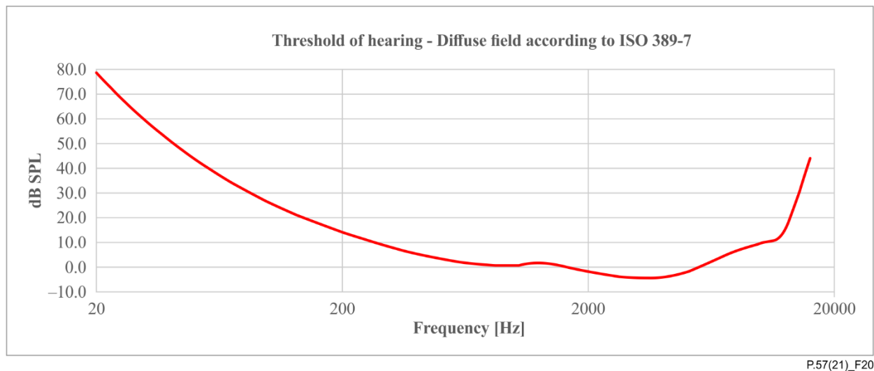
Figure 20 – Hearing threshold according to [ISO 389-7]
