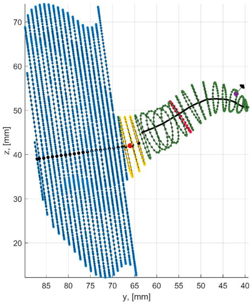
Figure 13-a – Points on the periphery of the cross-sectional areas of the anatomically shaped ear canal, concha bottom and pinna simulator of the type 4.3 ear simulator. The green and yellow cross sections represent the ear canal and concha bottom, the red cross section is the reference plane of the ear canal. The purple point is the DRP and the vector is the normal vector of the measurement plane. The blue cross sections represent the pinna.
