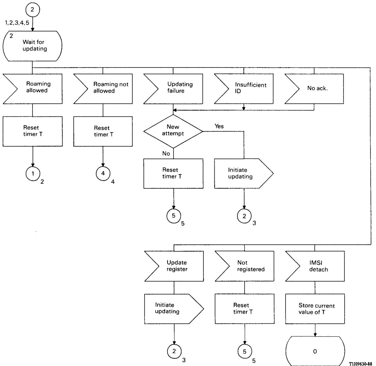
FIGURE 1/Q.1003 (Sheet 3 of 5) Logic procedures in the MS for location updating
