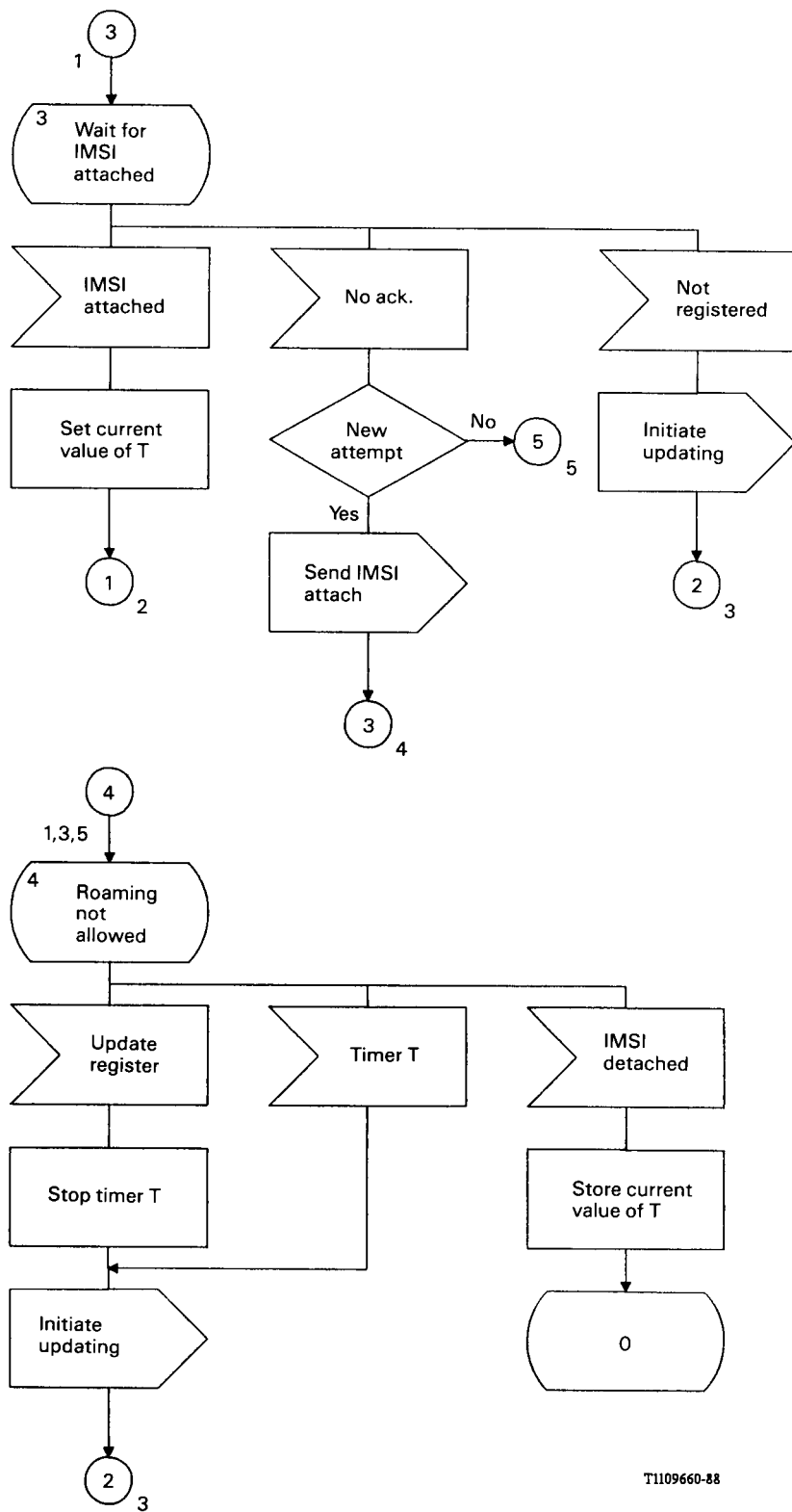
FIGURE 1/Q.1003 (Sheet 4 of 5) Logic procedures in the MS for location updating
