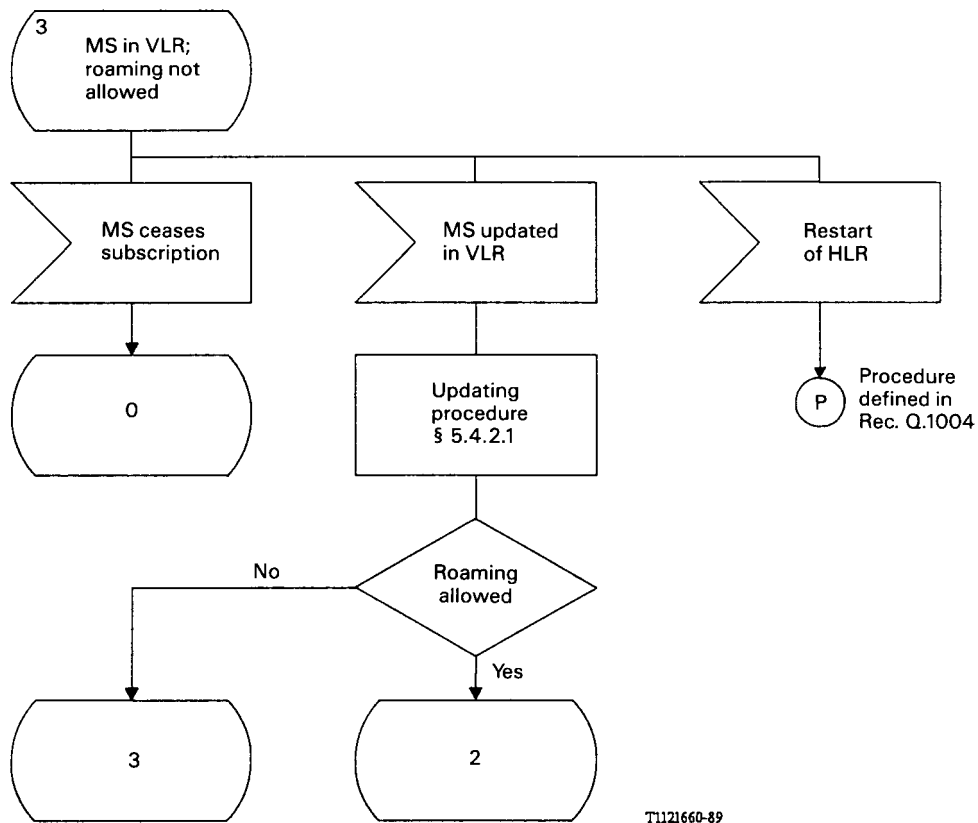
FIGURE 2/Q.1003 (Sheet 3 of 3) State diagram for home location register
