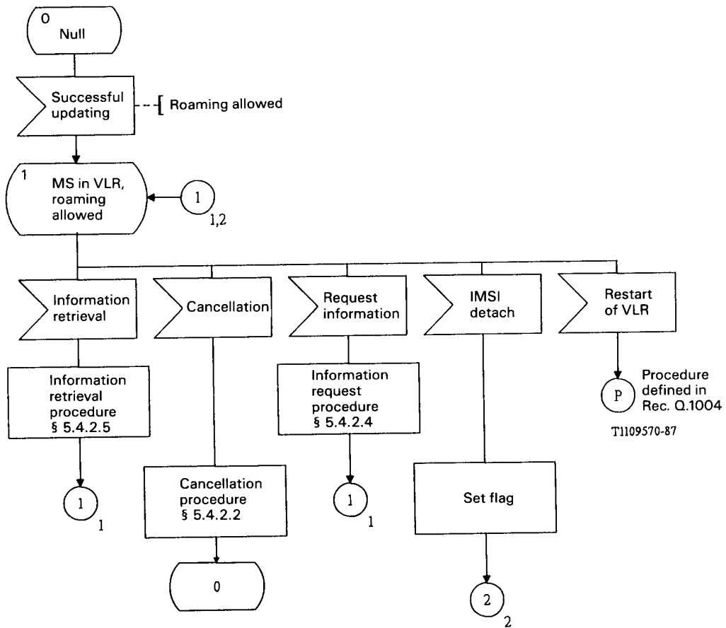
FIGURE 3/Q.1003 (Sheet 1 of 2) State diagram for visitor location register
