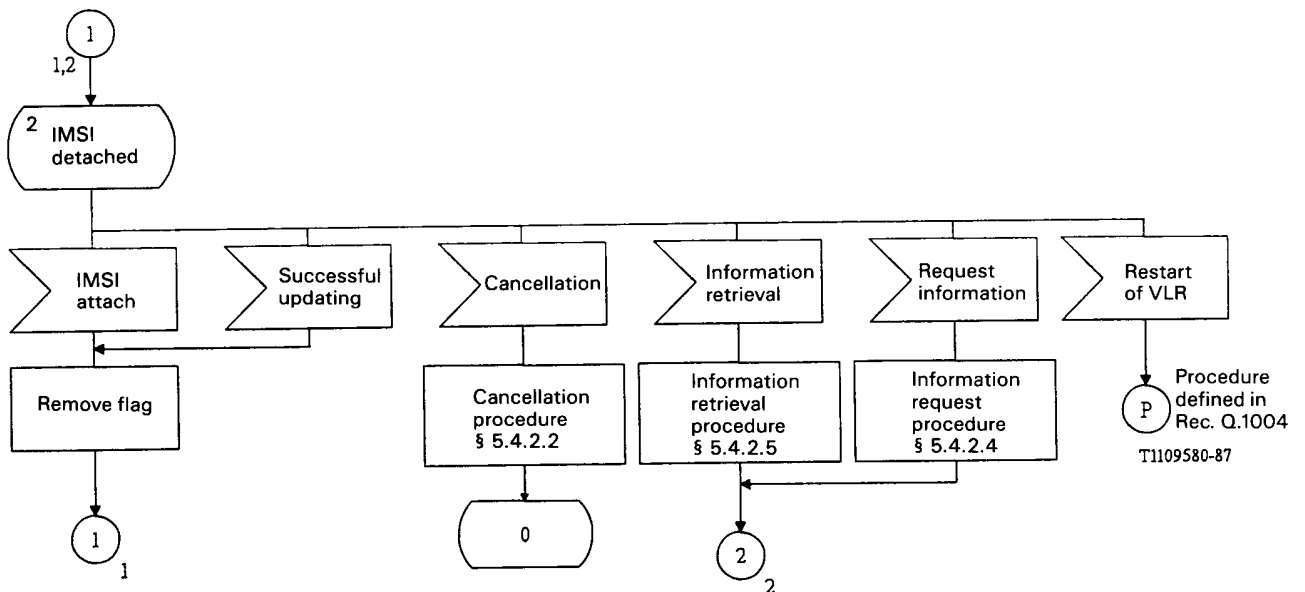
FIGURE 3/Q.1003 (Sheet 2 of 2) State diagram for visitor location register
