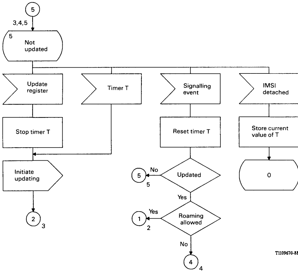
FIGURE 1/Q.1003 (Sheet 5 of 5) Logic procedures in the MS for location updating
