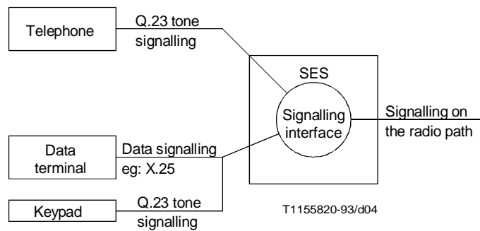
FIGURE 4/Q.1111 SES signalling interface for non-ISDN terminals
