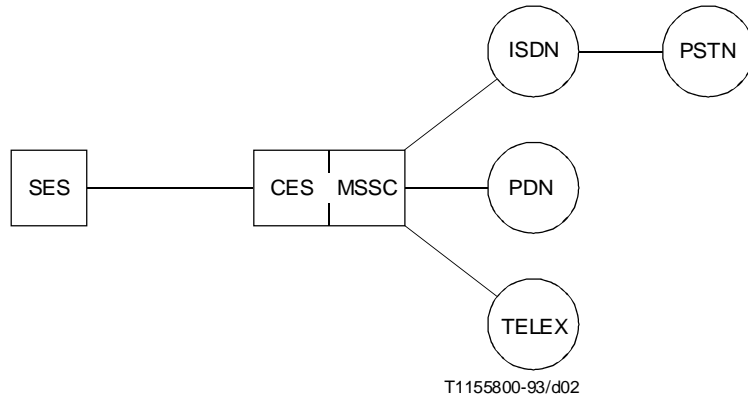
FIGURE 2/Q.1111 Interim interworking scenario with interfaces to ISDN and other fixed networks
