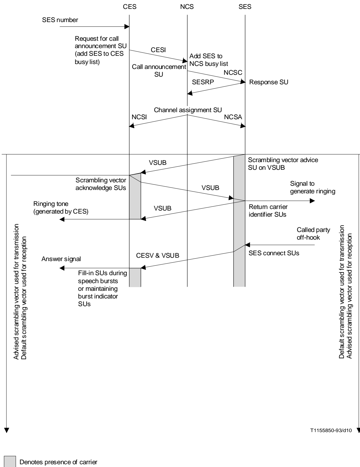
FIGURE I.5/Q.1111 Standard-B shore originated telephone call set-up sequence
