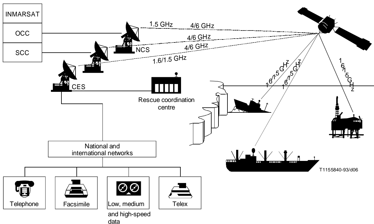
FIGURE I.1/Q.1111 Standard-B network configuration
