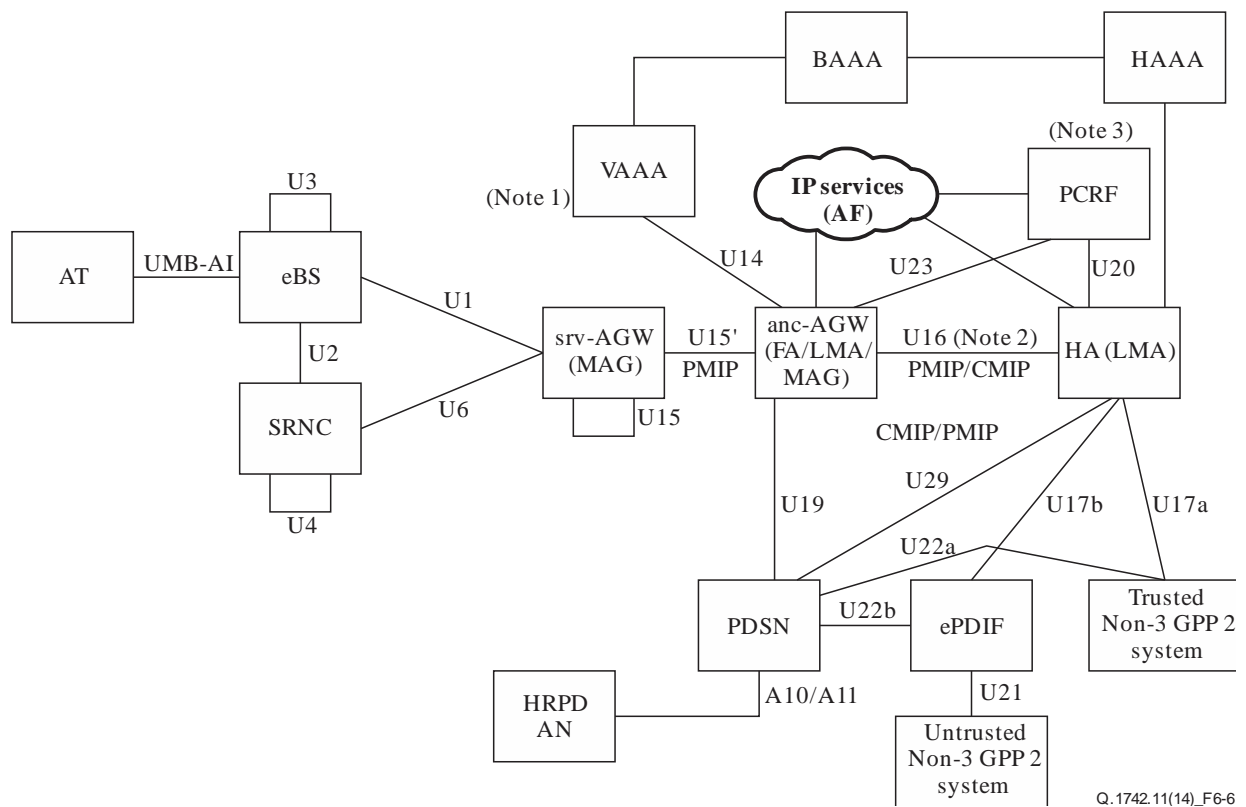
Figure 6-6 – Converged access network reference model – non-roaming
