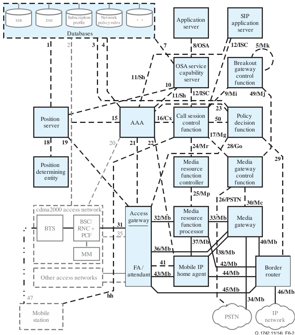
Figure 6-2 – ANSI-41-evolved core network with cdma2000 access network IP MMD core network architecture model
