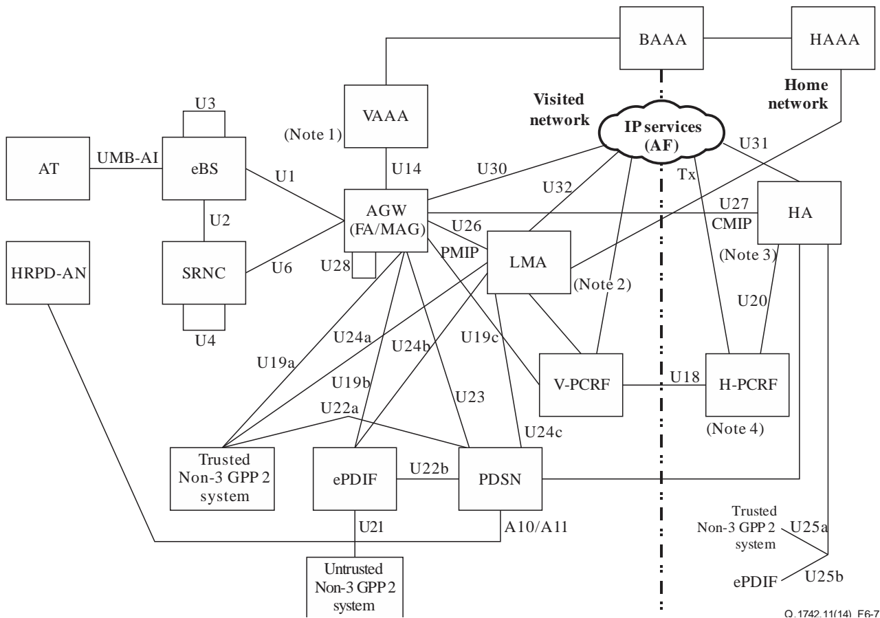
Figure 6-7 – Converged access network reference model – roaming
