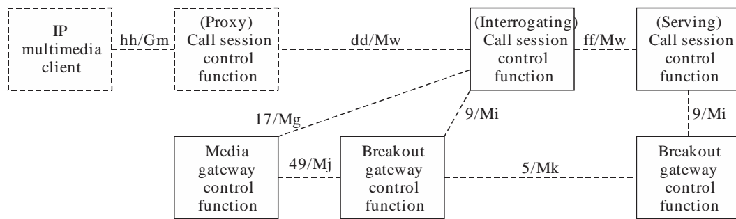
Figure 6-5 – Session control reference model
