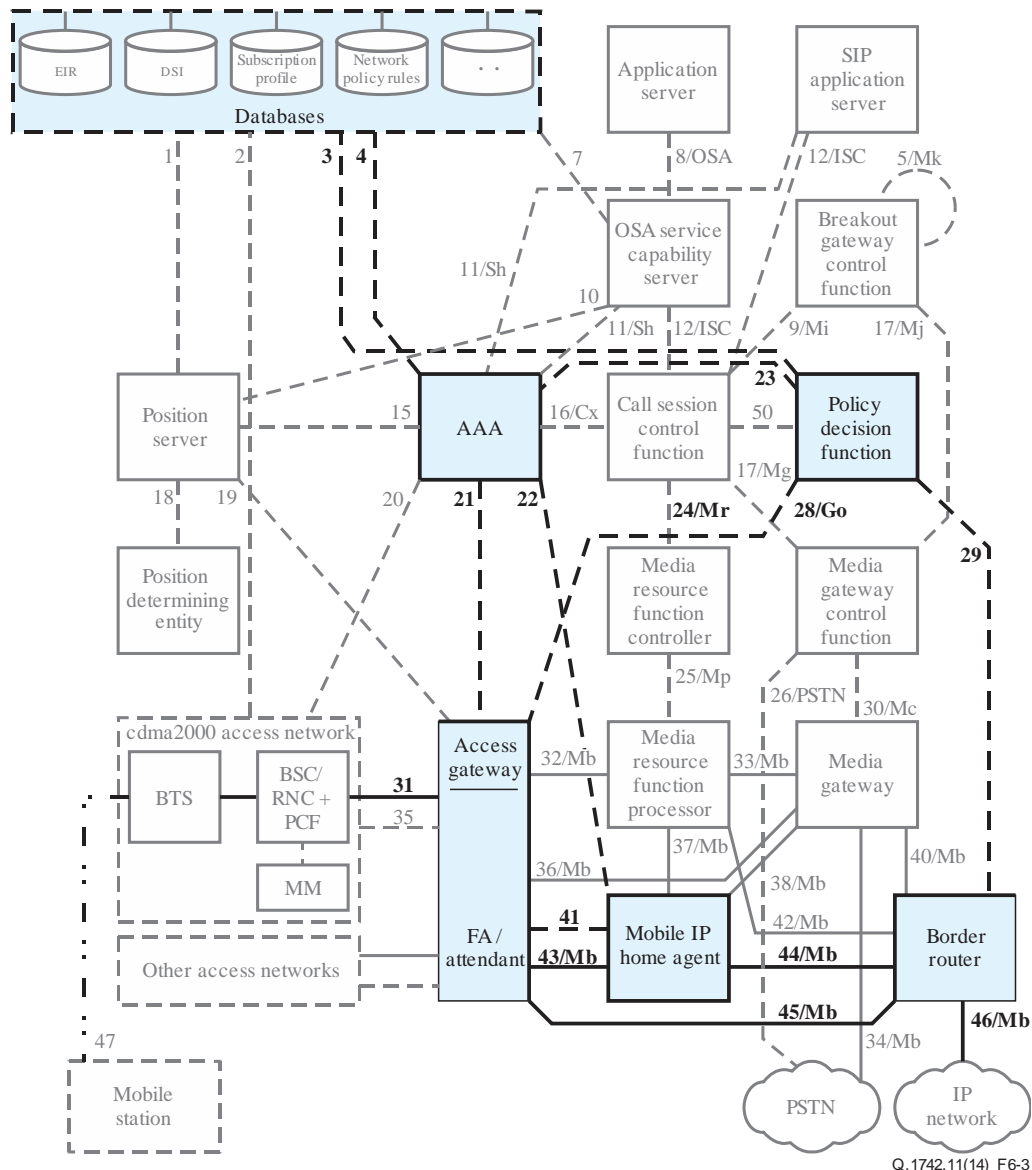
Figure 6-3 – ANSI-41-evolved core network with cdma2000 access network packet data subsystem core network architecture model
