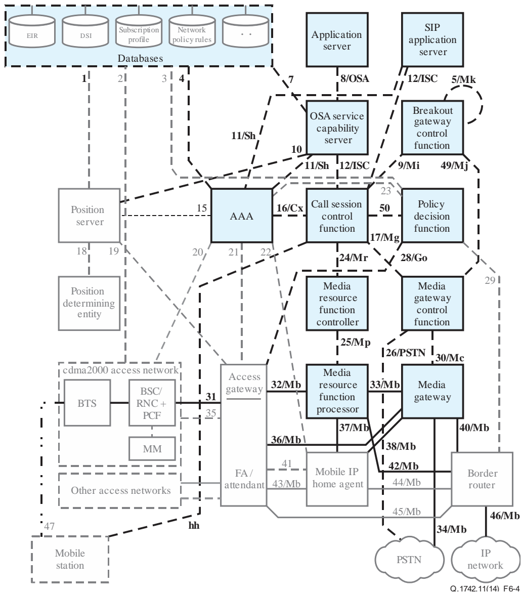
Figure 6-4 – ANSI-41-evolved core network with cdma2000 access network IP multimedia session subsystem core network architecture model
