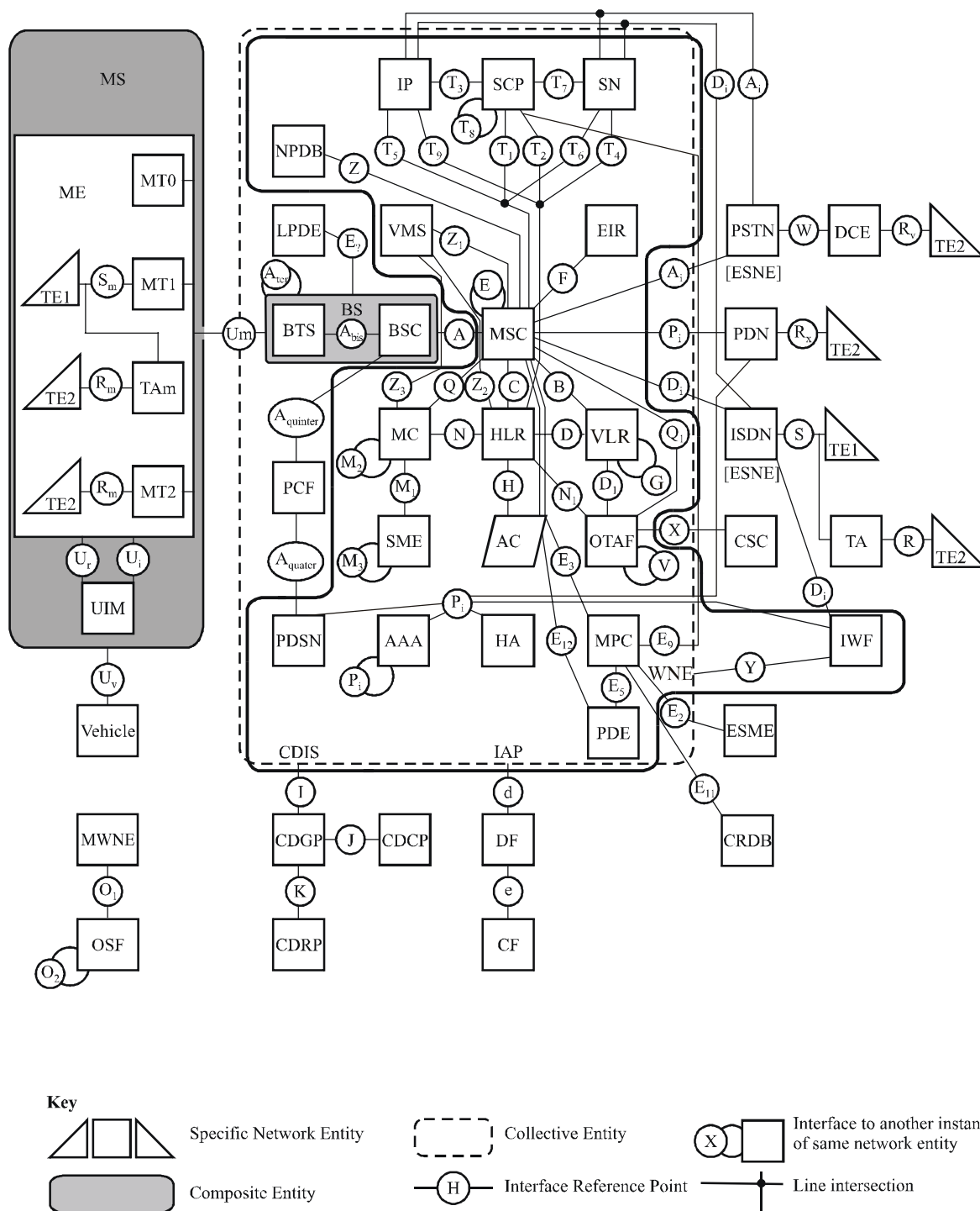
Figure 6-1 – ANSI-41 evolved core network with cdma2000 access network reference model
