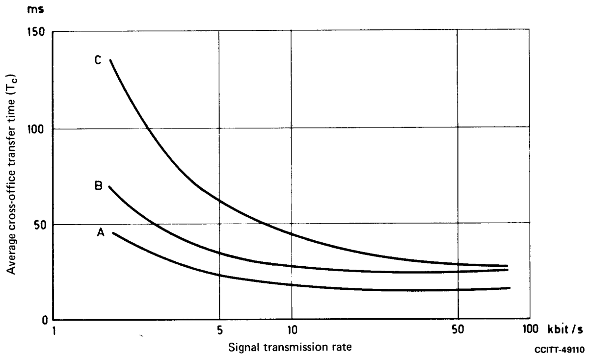
FIGURE 23/Q.287
