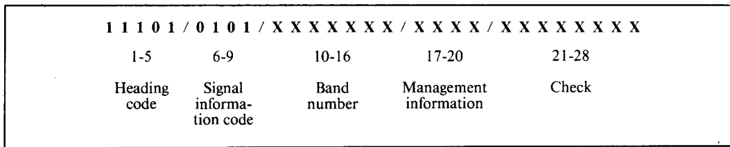
FIGURE 14/Q.260 Format of a one-unit signalling-network-management message
