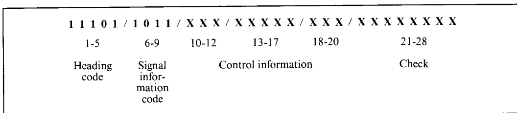
FIGURE 11/Q.259
