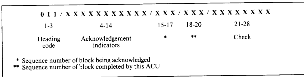
FIGURE 8/Q.259 Format of the acknowledgement signal unit
