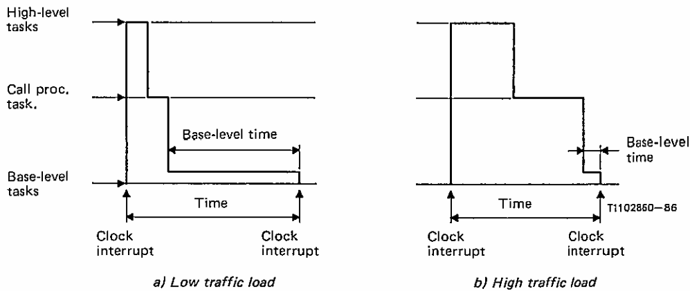
FIGURE B-2/Q.543 Allocation of processor time to tasks
