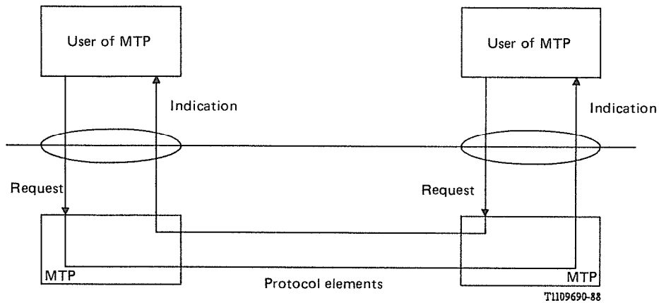
FIGURE 2/Q.701
