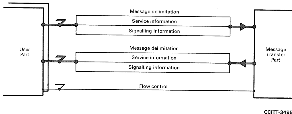
FIGURE 5/Q.701
