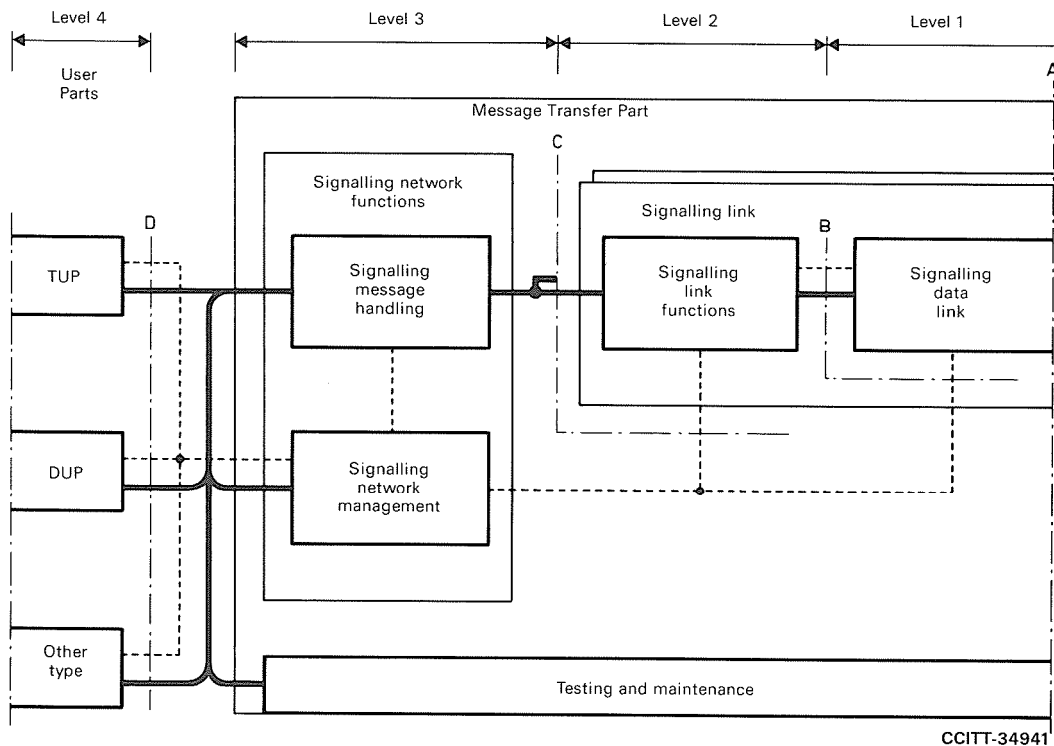
FIGURE 4/Q.701
