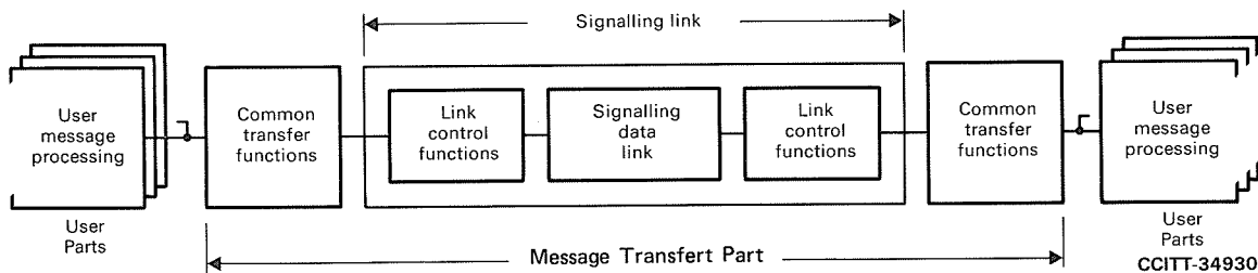
FIGURE 3/Q.701
