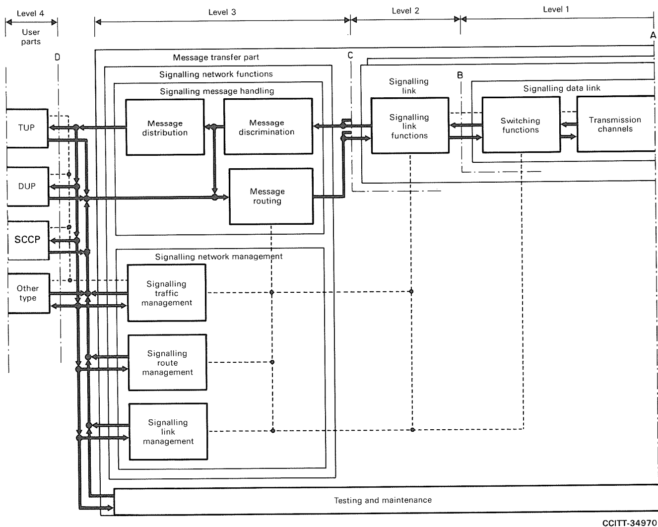
FIGURE 6/Q.701
