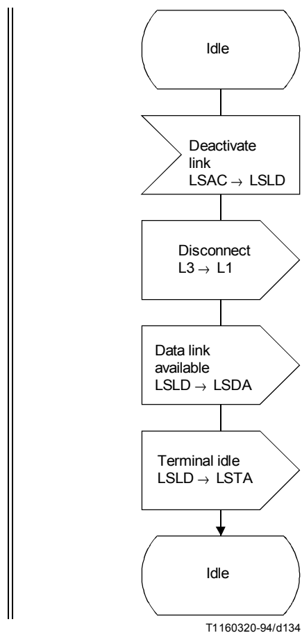
FIGURE 40/Q.704
