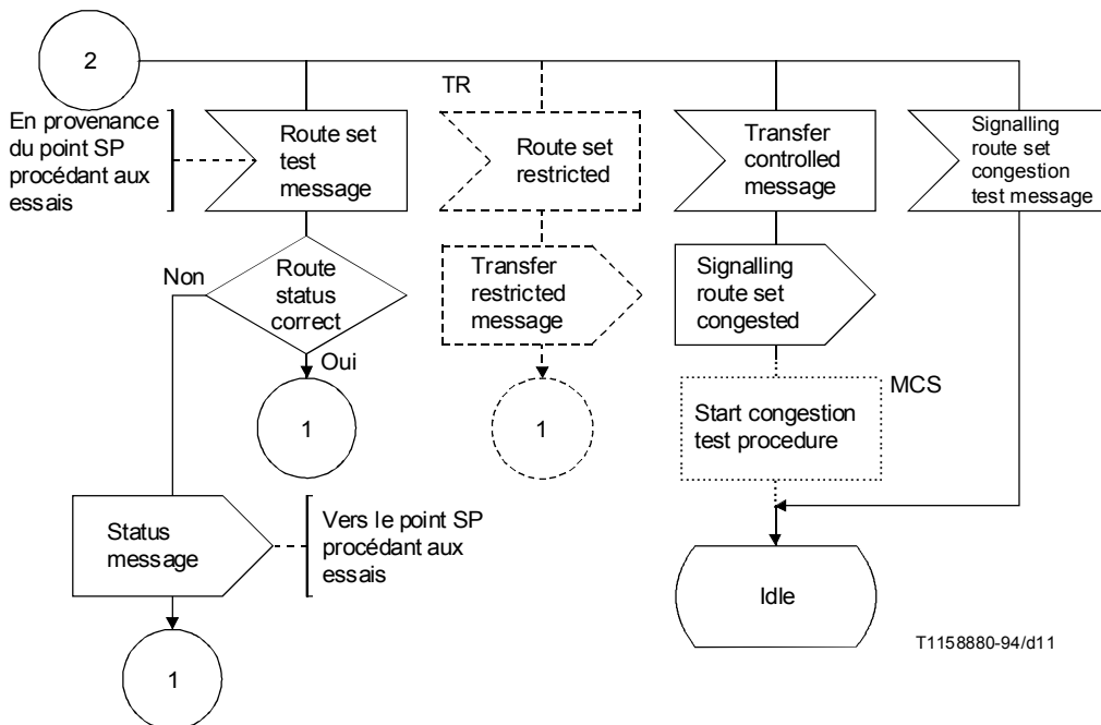
FIGURE 8/Q.704
