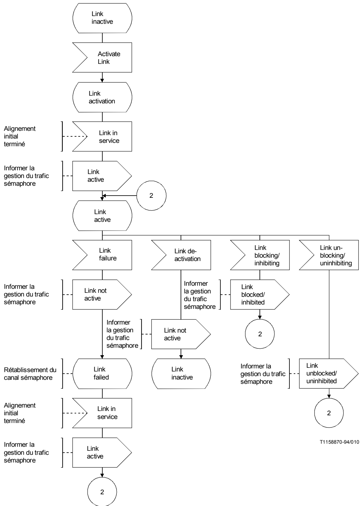
FIGURE 7/Q.704
