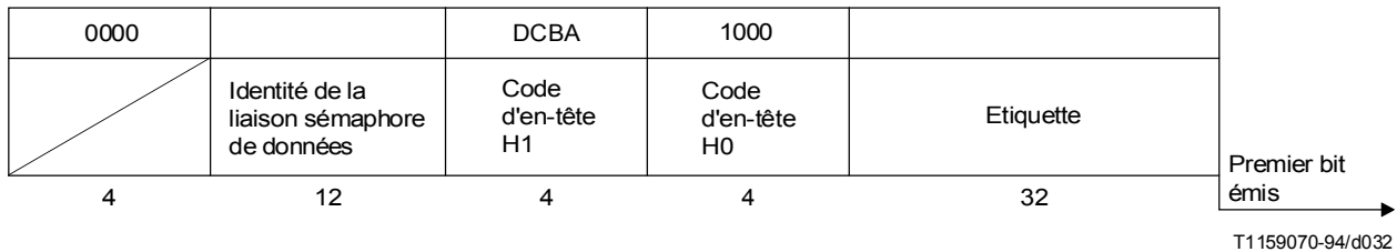
FIGURE 22/Q.704
