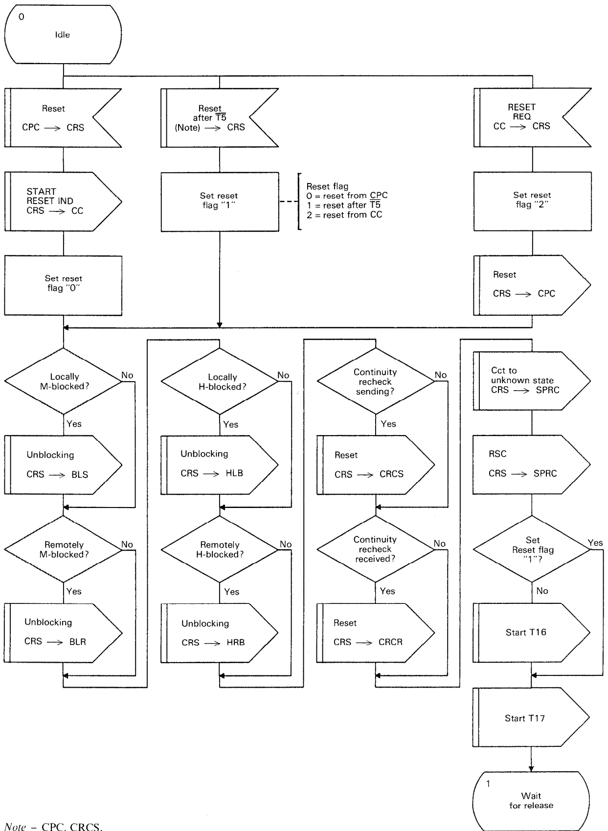
FIGURE B-33/Q.764 (Sheet 1 of 3)
