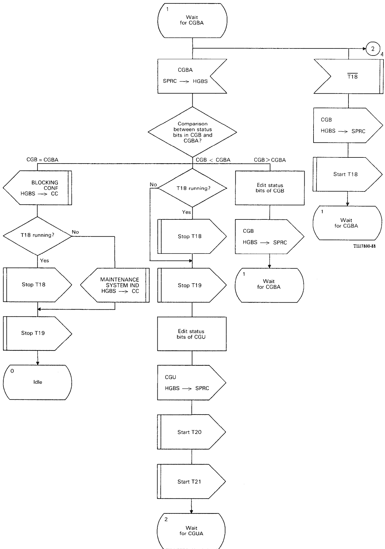
FIGURE B-31/Q.764 (Sheet 3 of 6)
