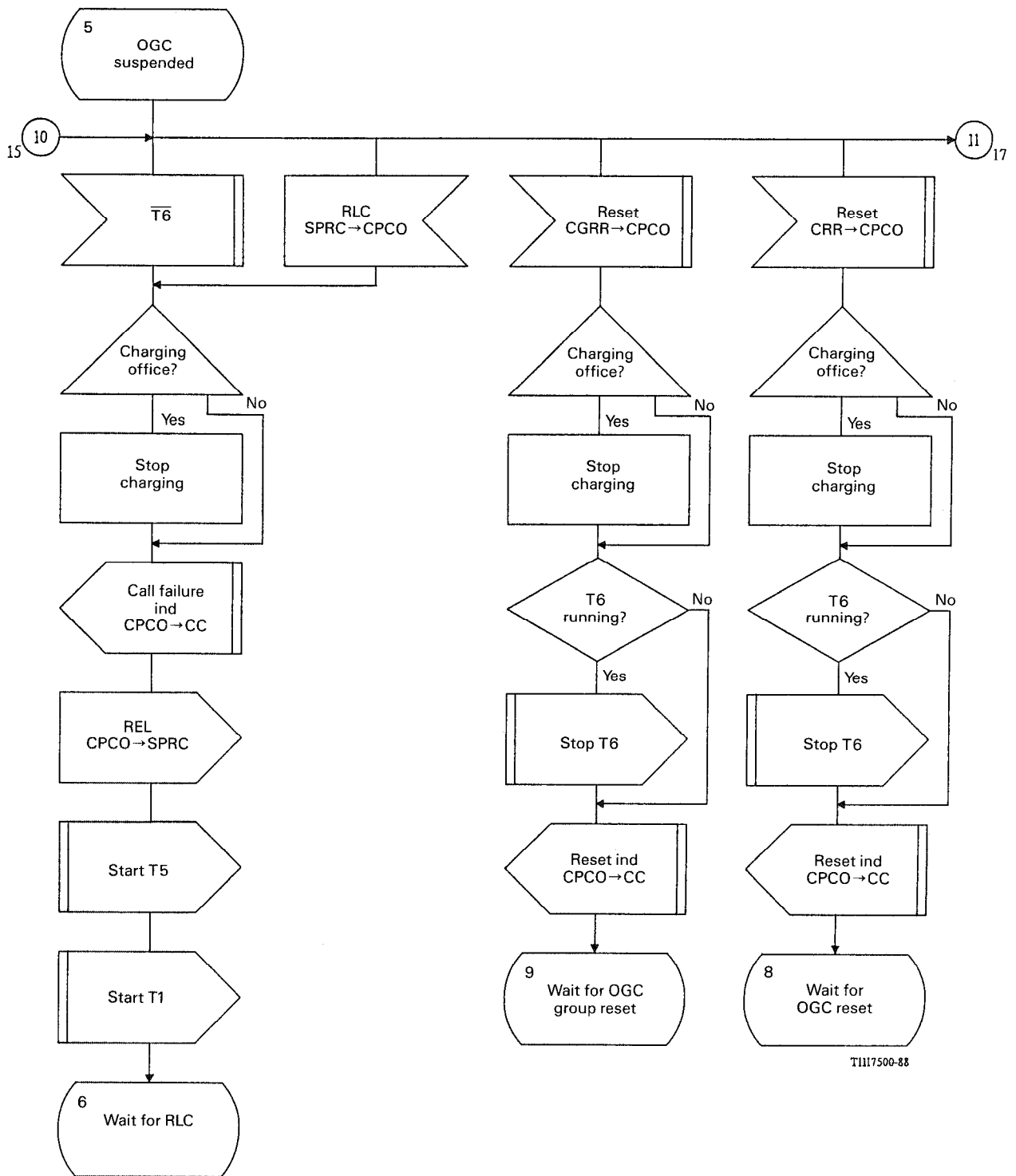
FIGURE B-22/Q.764 (Sheet 16 of 21) Call Processing Control Outgoing (CPCO)
