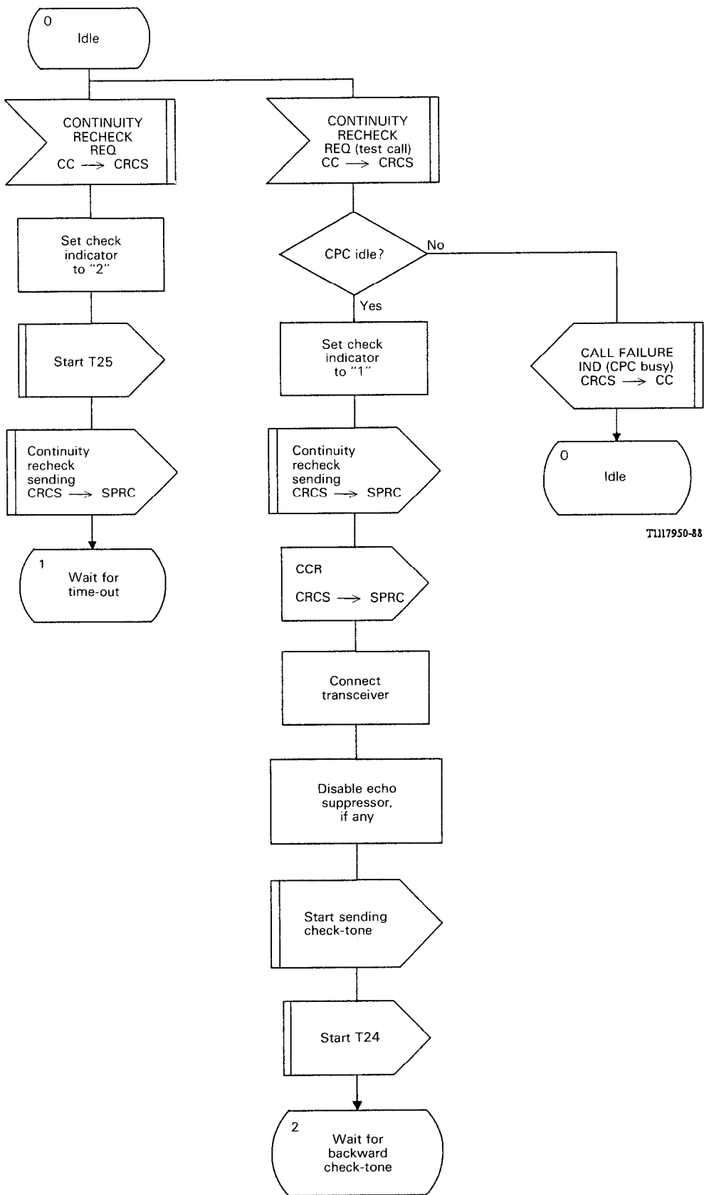
FIGURE B-37/Q.764 (Sheet 1 of 6)
