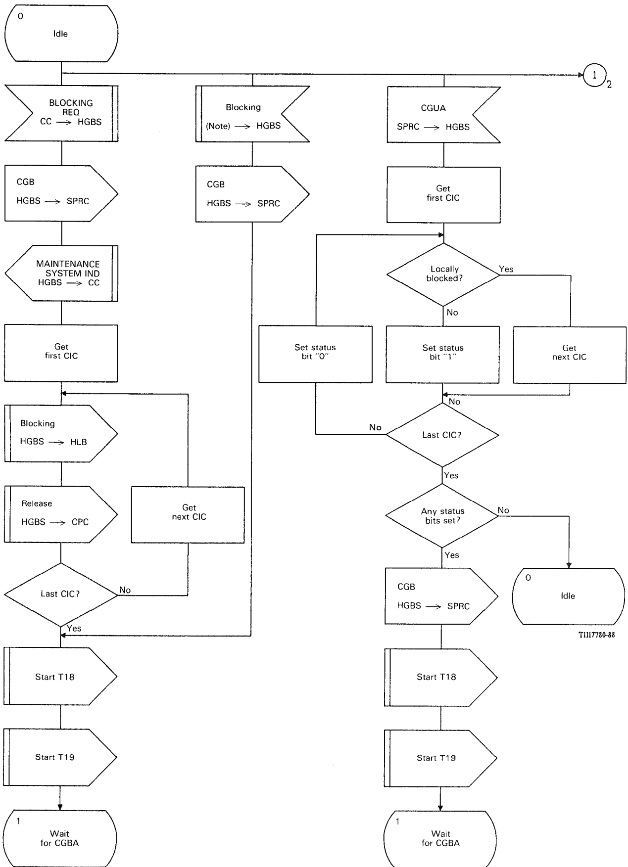
FIGURE B-31/Q.764 (Sheet 1 of 6)
