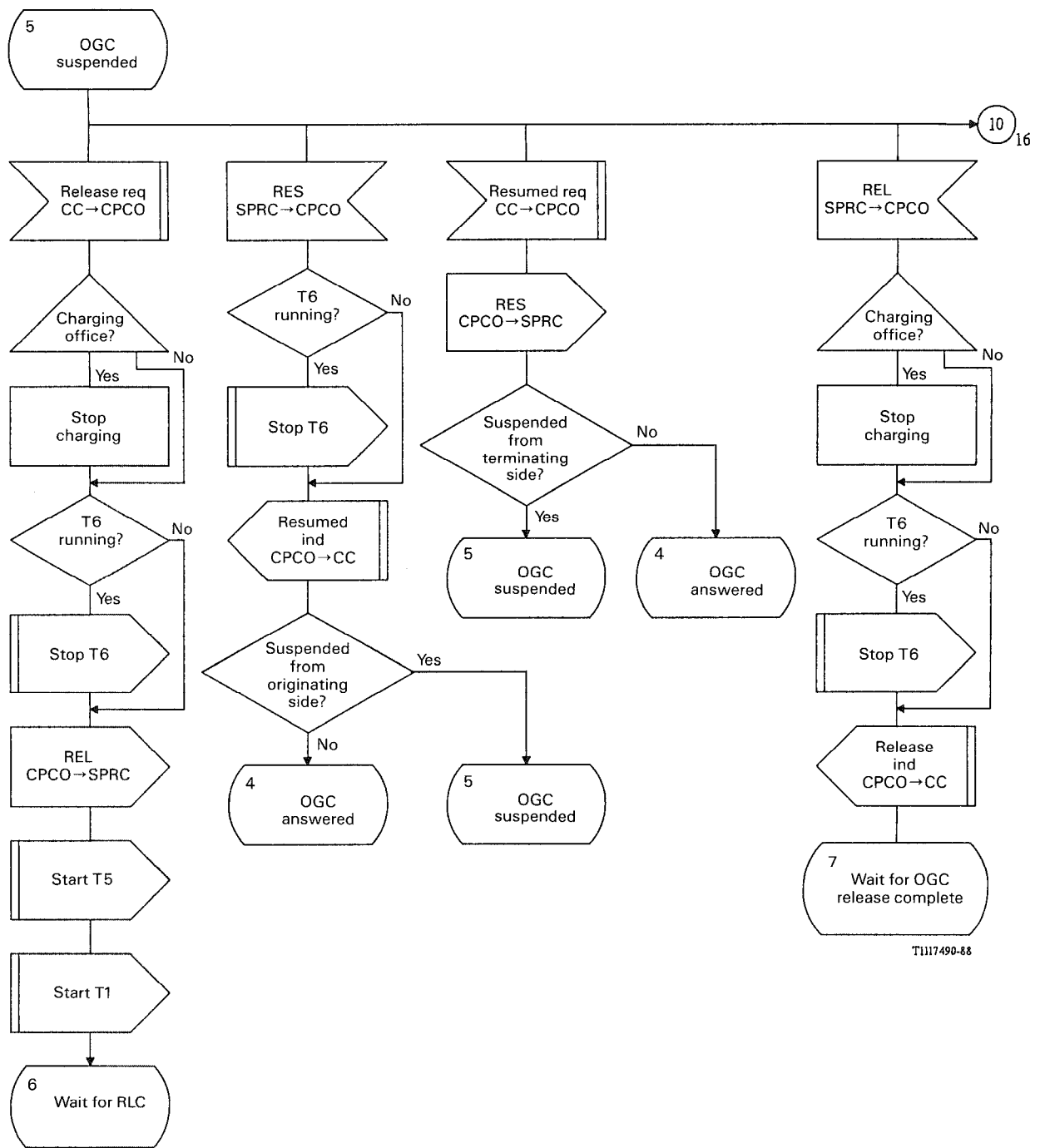
FIGURE B-22/Q.764 (Sheet 15 of 21) Call Processing Control Outgoing (CPCO)
