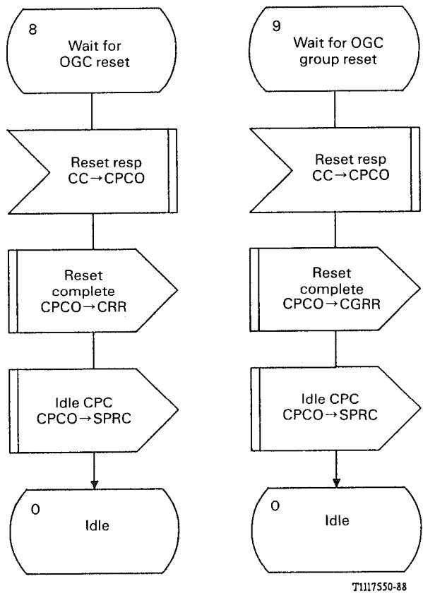
FIGURE B-22/Q.764 (Sheet 21 of 21) Call Processing Control Outgoing (CPCO)
