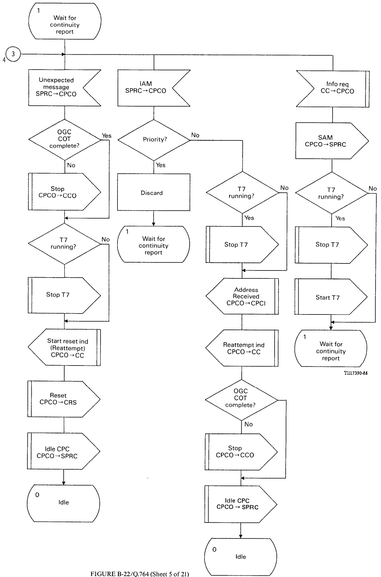
FIGURE B-22/Q.764 (Sheet 5 of 21)
