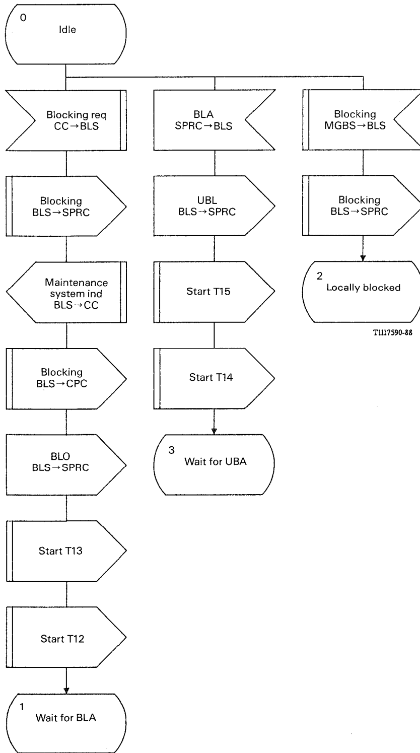
FIGURE B-25/Q.764 (Sheet 1 of 5)
