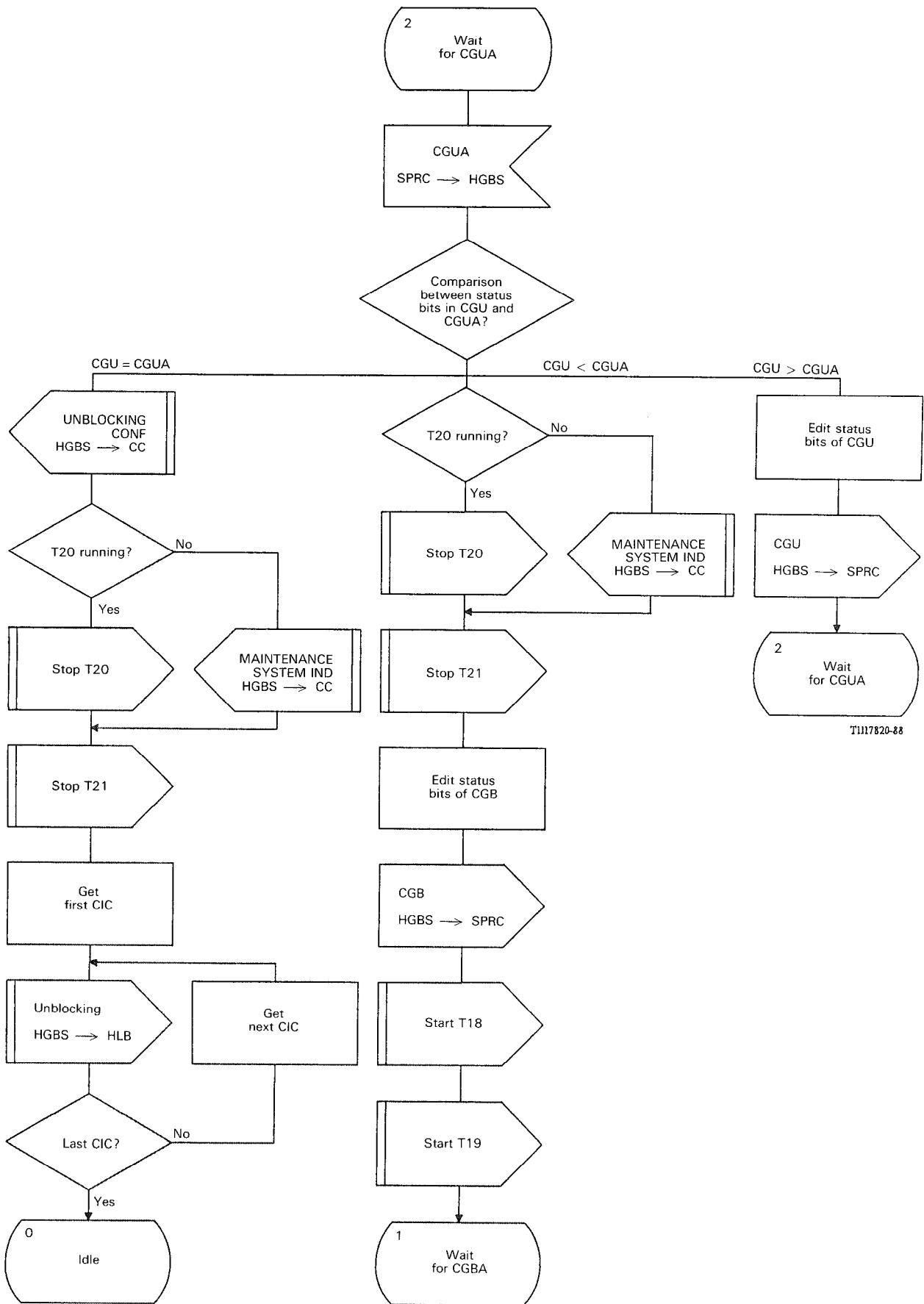
FIGURE B-31/Q.764 (Sheet 5 of 6)
