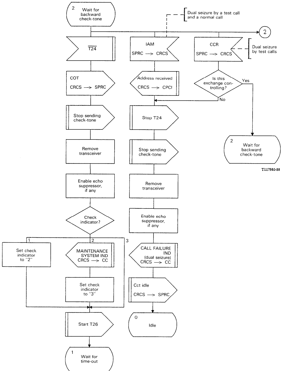
FIGURE B-37/Q.764 (Sheet 4 of 6)
