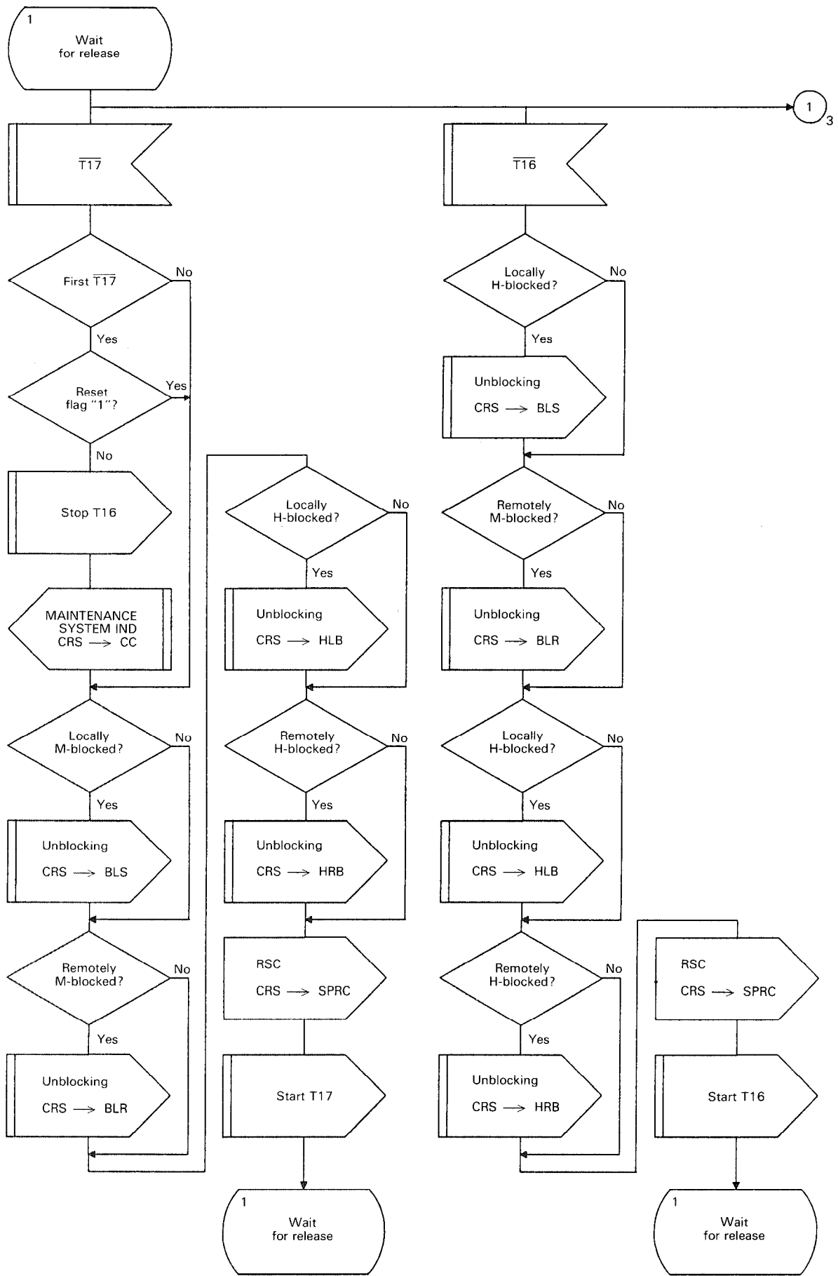
FIGURE B-33/Q.764 (Sheet 2 of 3) Circuit Reset Sending (CRS)
