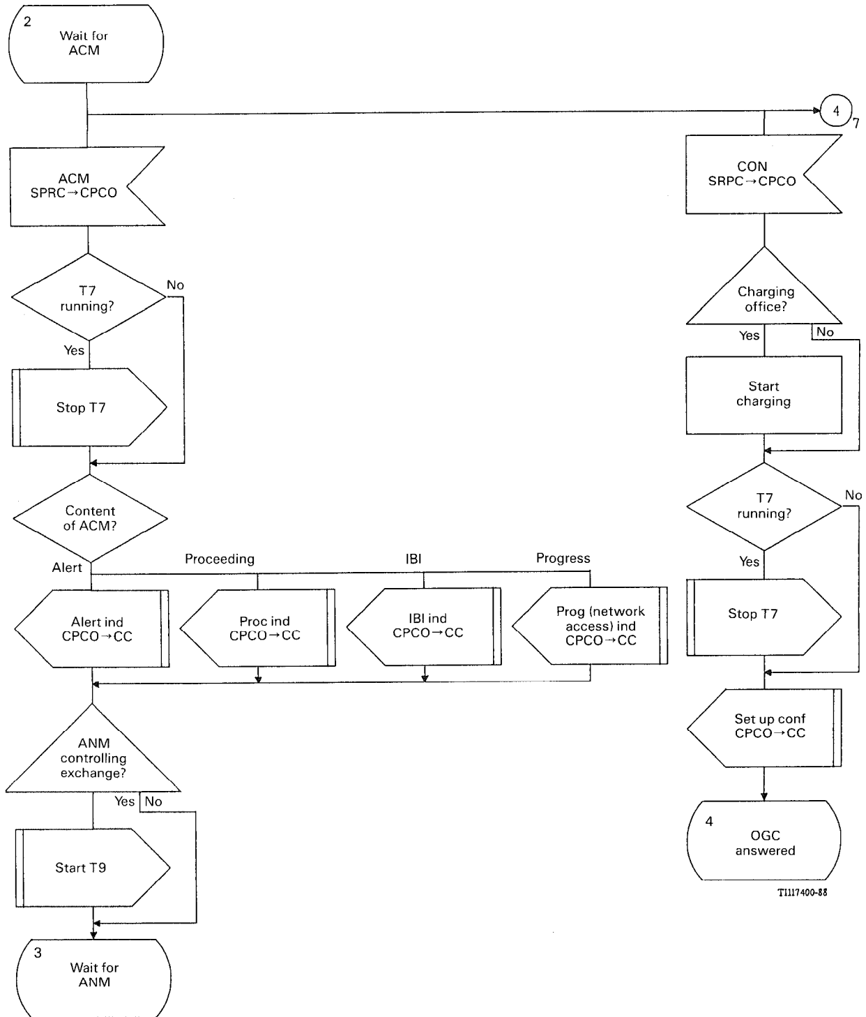
FIGURE B-22/Q.764 (Sheet 6 of 21) Call Processing Control Outgoing (CPCO)
