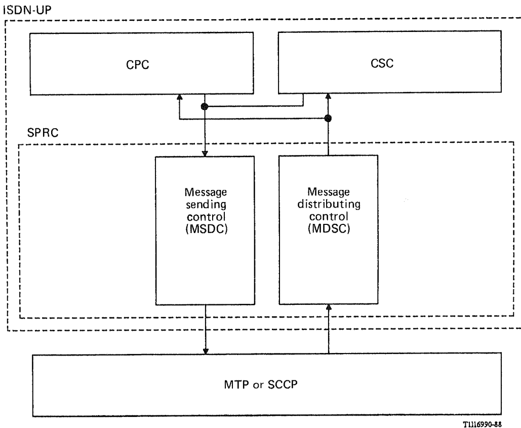
FIGURE B-4/Q.764 Functional block diagram for SPRC
