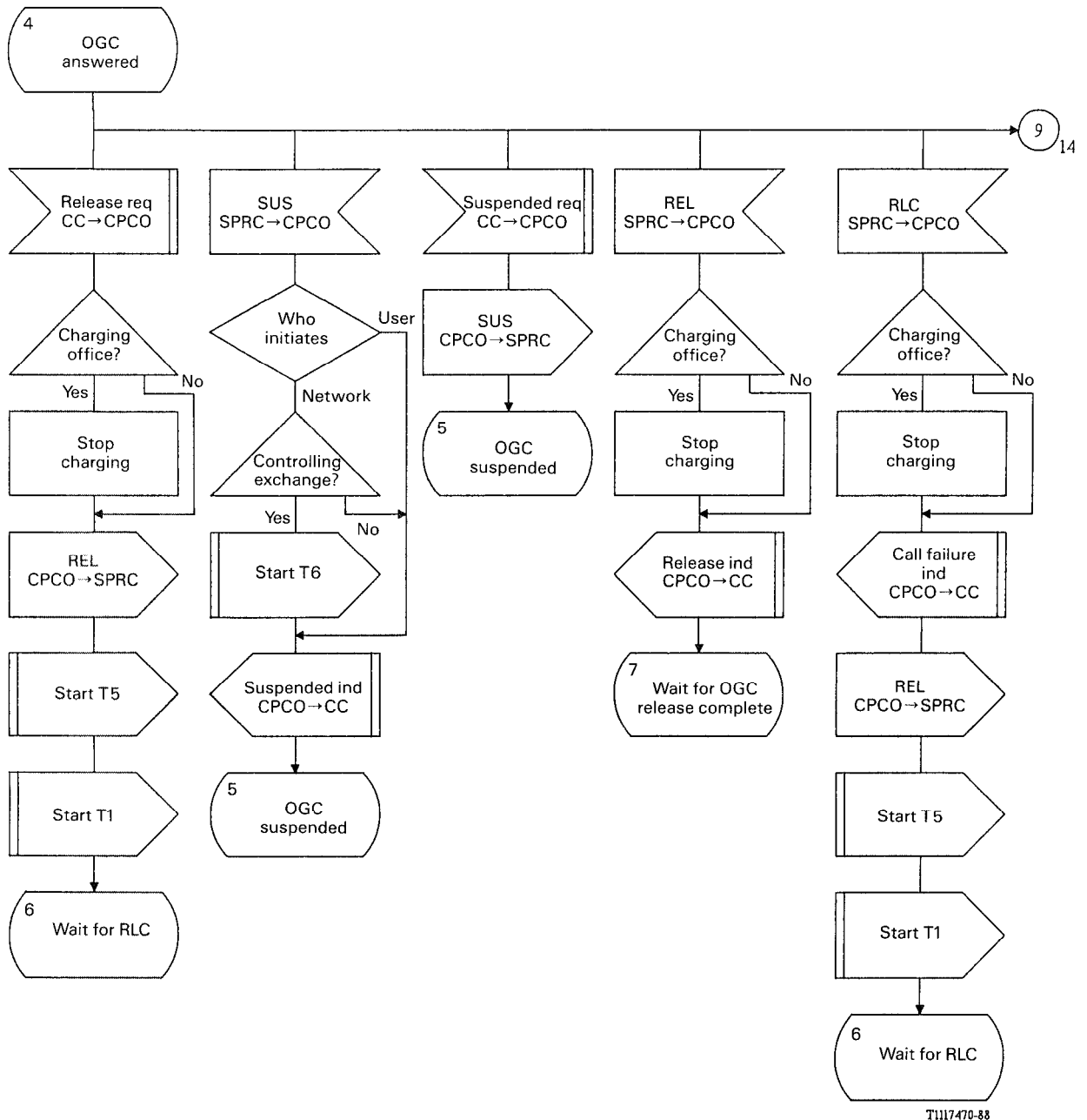
FIGURE B-22/Q.764 (Sheet 13 of 21) Call Processing Control Outgoing (CPCO)
