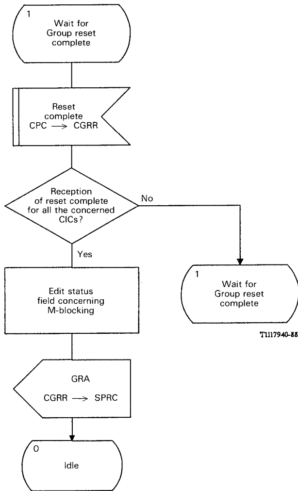
FIGURE B-36/Q.764 (Sheet 2 of 2)
