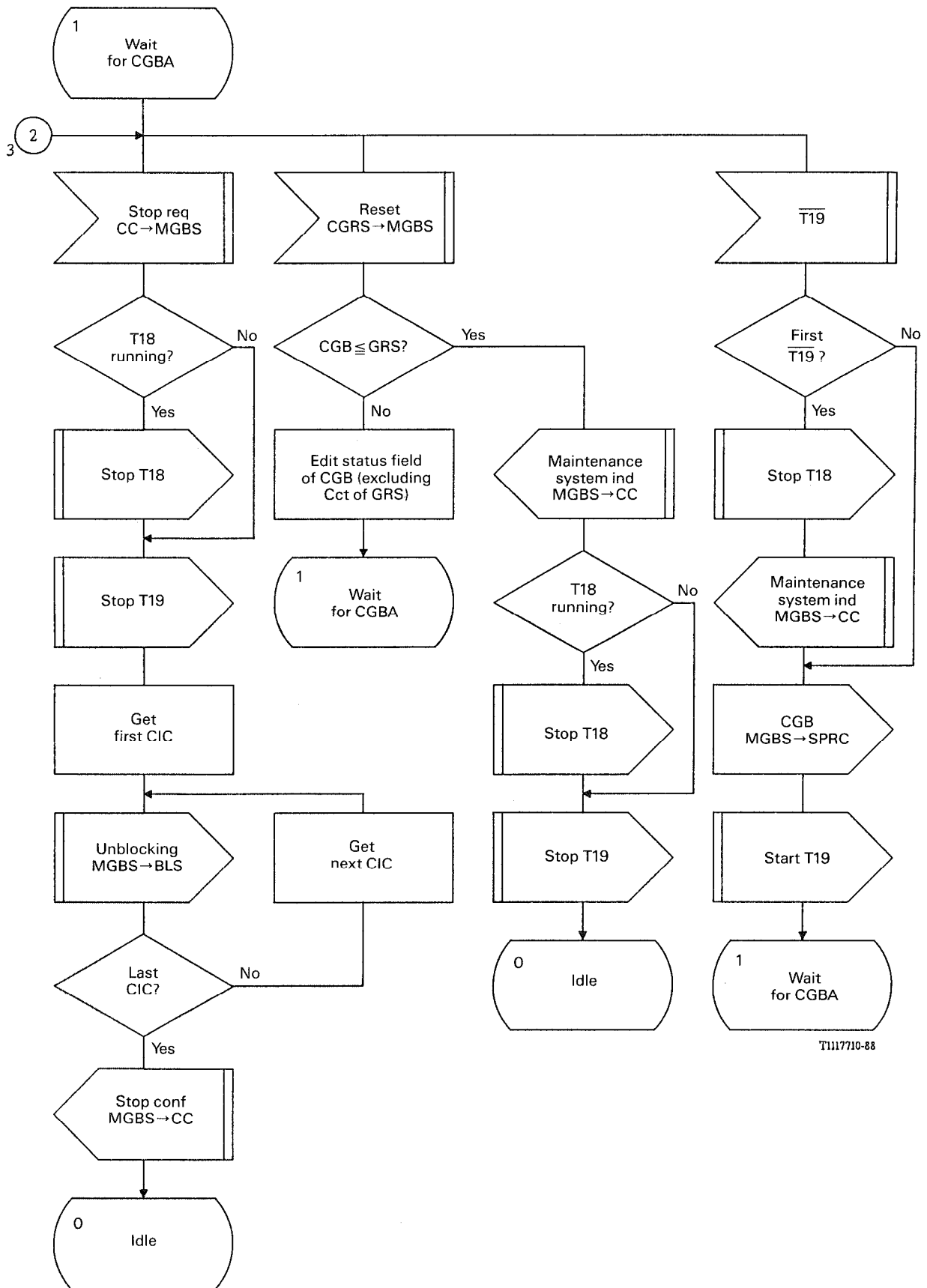
FIGURE B-27/Q.764 (Sheet 4 of 6)
