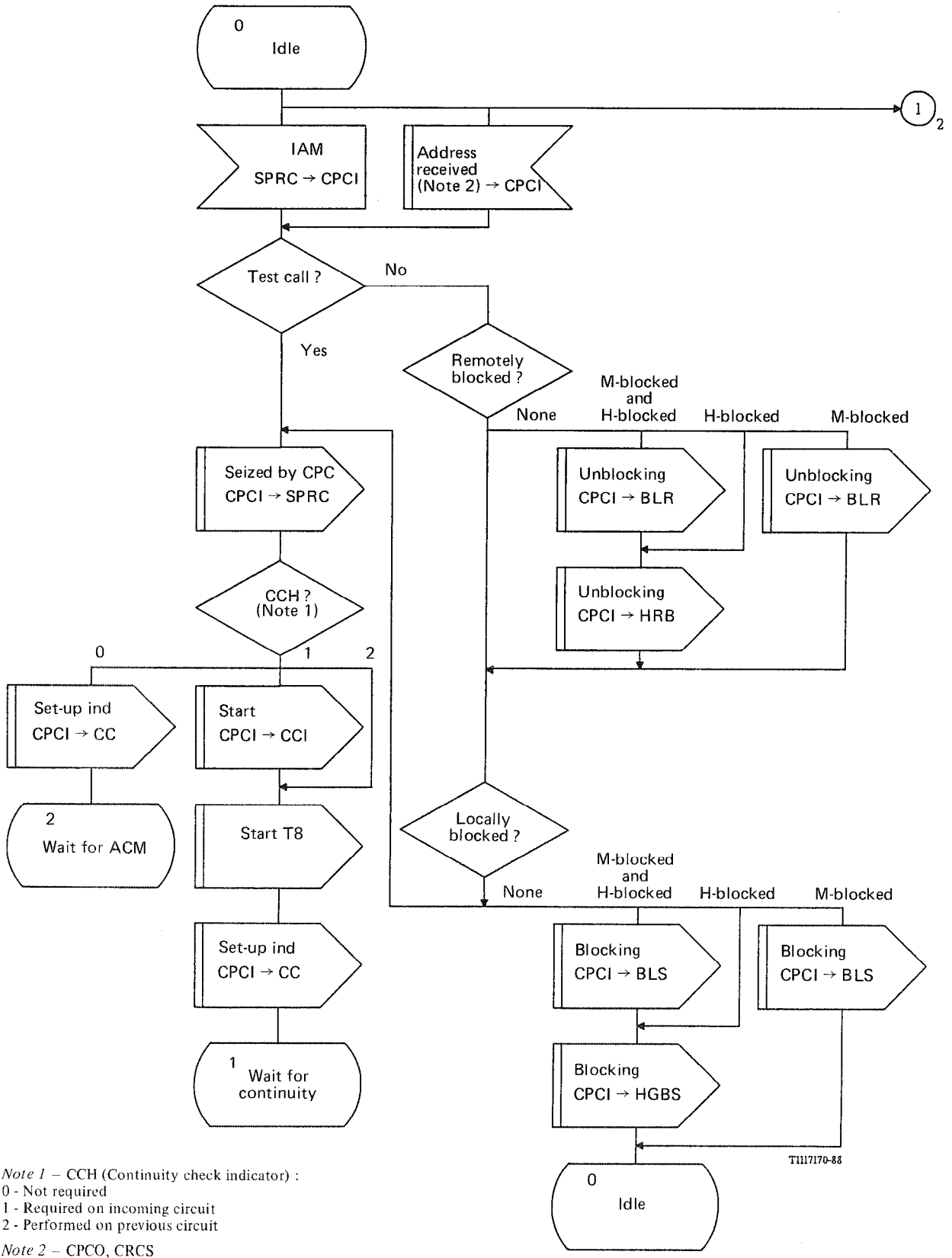
FIGURE B-21/Q.764 (sheet 1 of 18) Call processing control incoming (CPCI)
