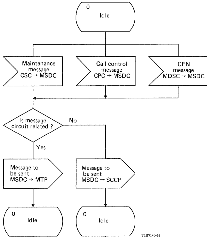
FIGURE B-19/Q.764 Message sending control (MSDC)
