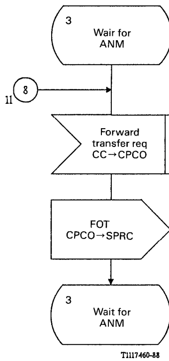
FIGURE B-22/Q.764 (Sheet 12 of 21) Call Processing Control Outgoing (CPCO)
