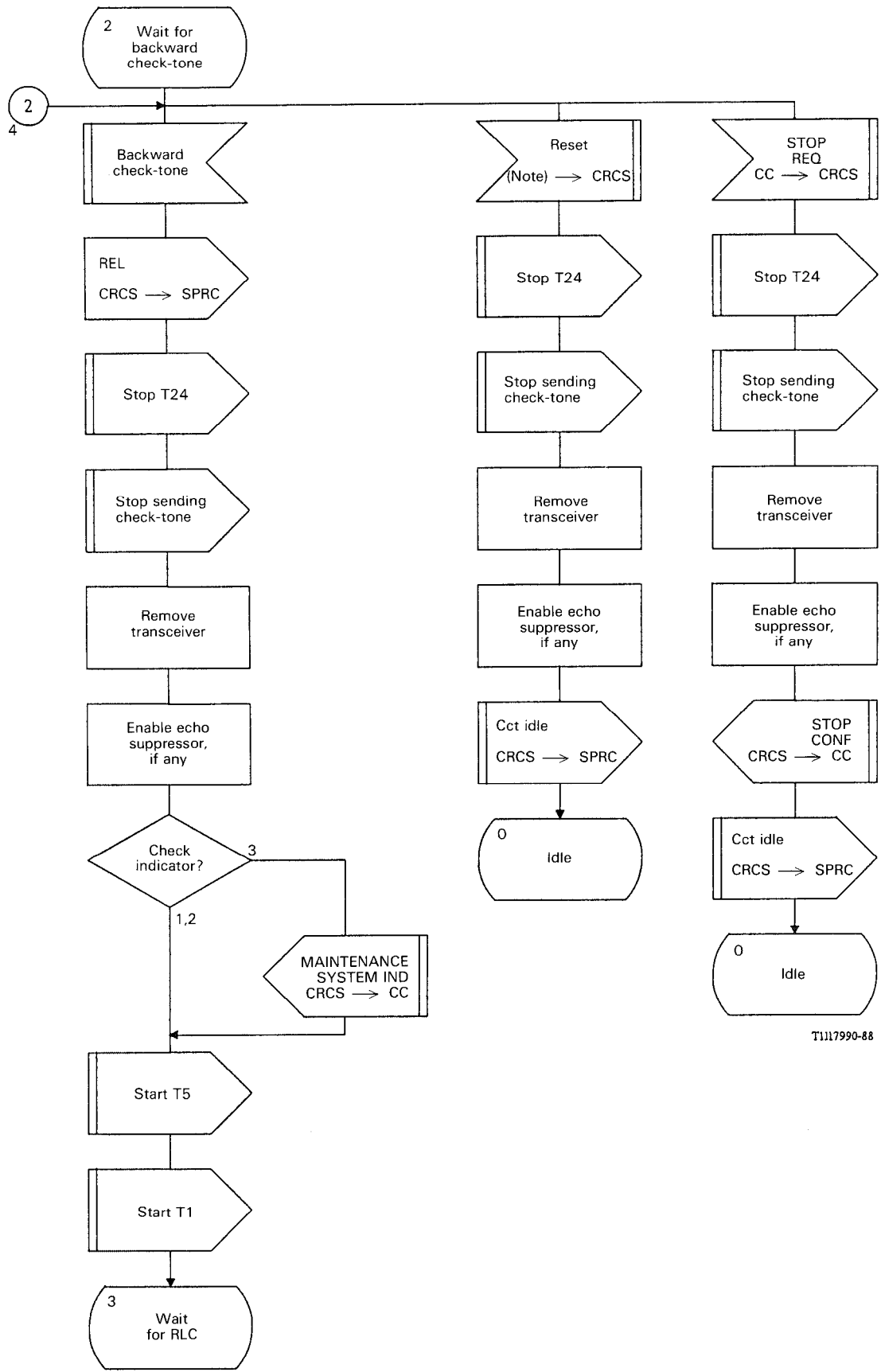
FIGURE B-37/Q.764 (Sheet 5 of 6)
