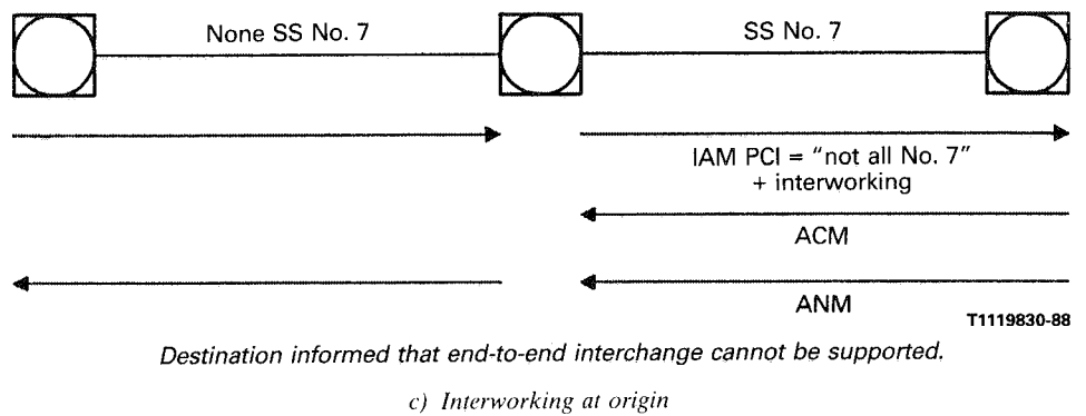
FIGURE 11/Q.764 Operation of end-to-end protocol (pass along method)
