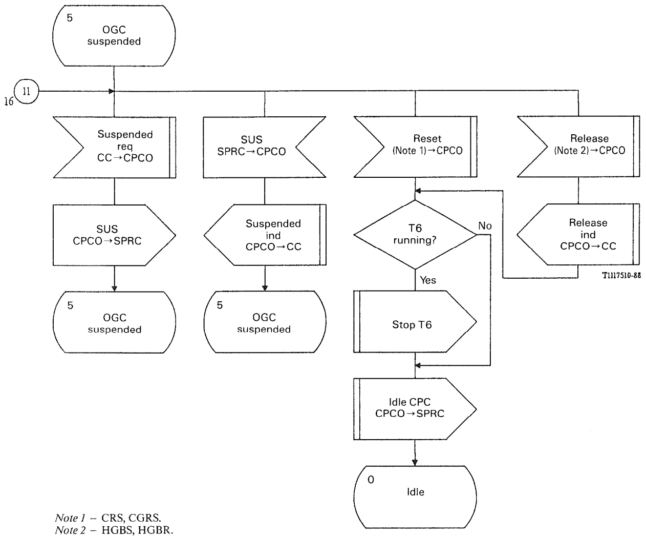
FIGURE B-22/Q.764 (Sheet 17 of 21) Call Processing Control Outgoing (CPCO)
