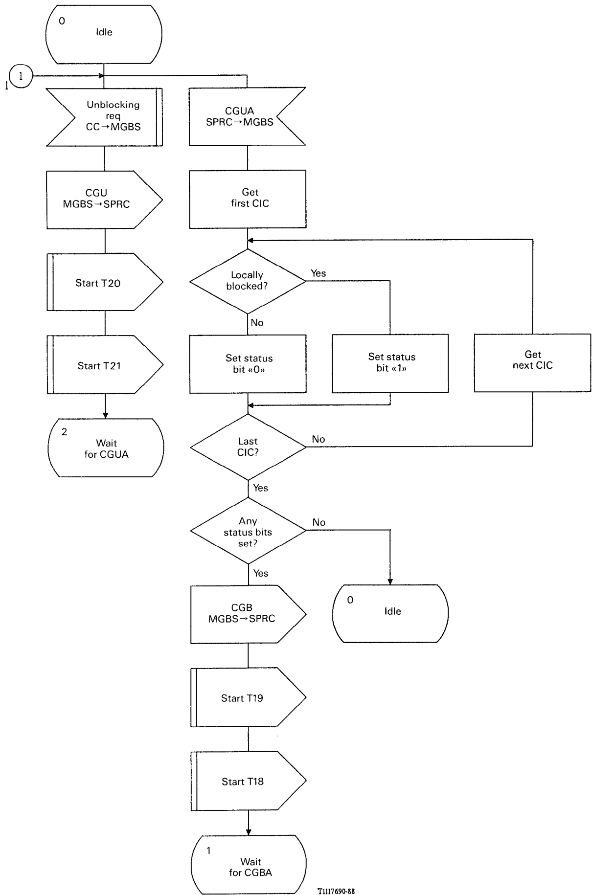
FIGURE B-27/Q.764 (Sheet 2 of 6) Maintenance Oriented Circuit Group Blocking and Unblocking Sending (MGBS)
