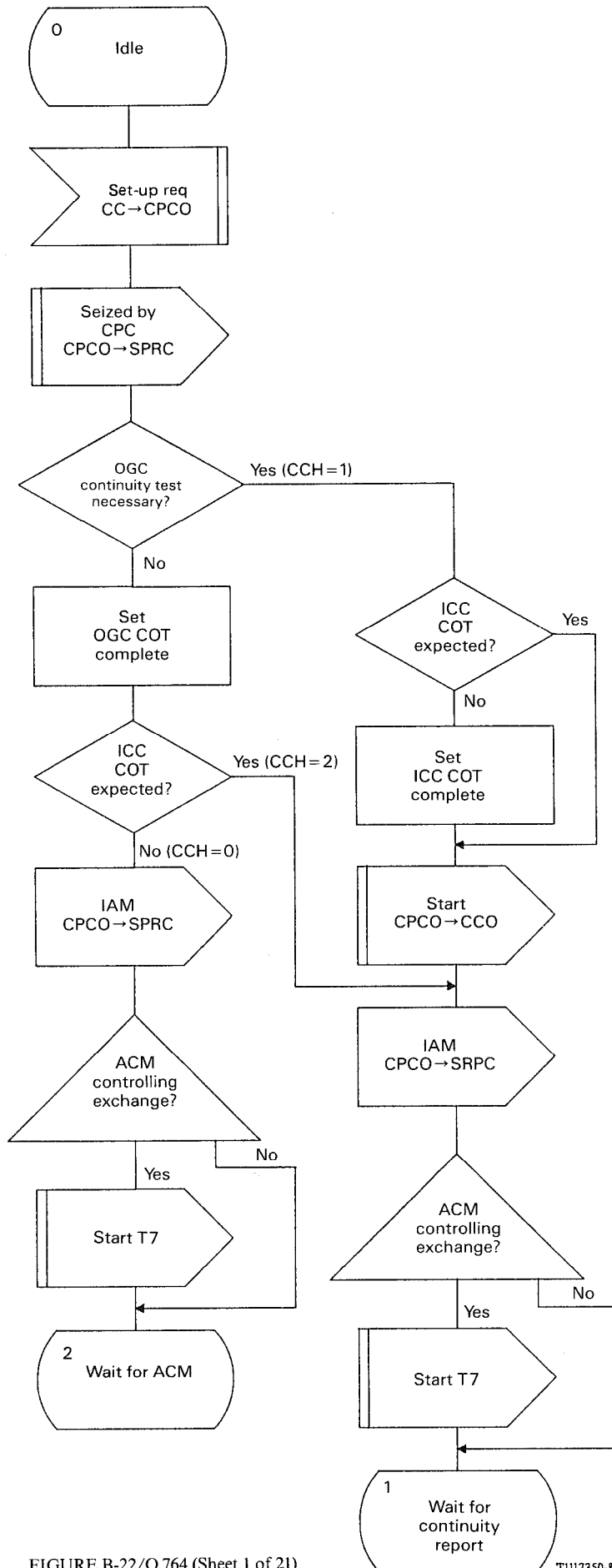
FIGURE B-22/Q.764 (Sheet 1 of 21)
