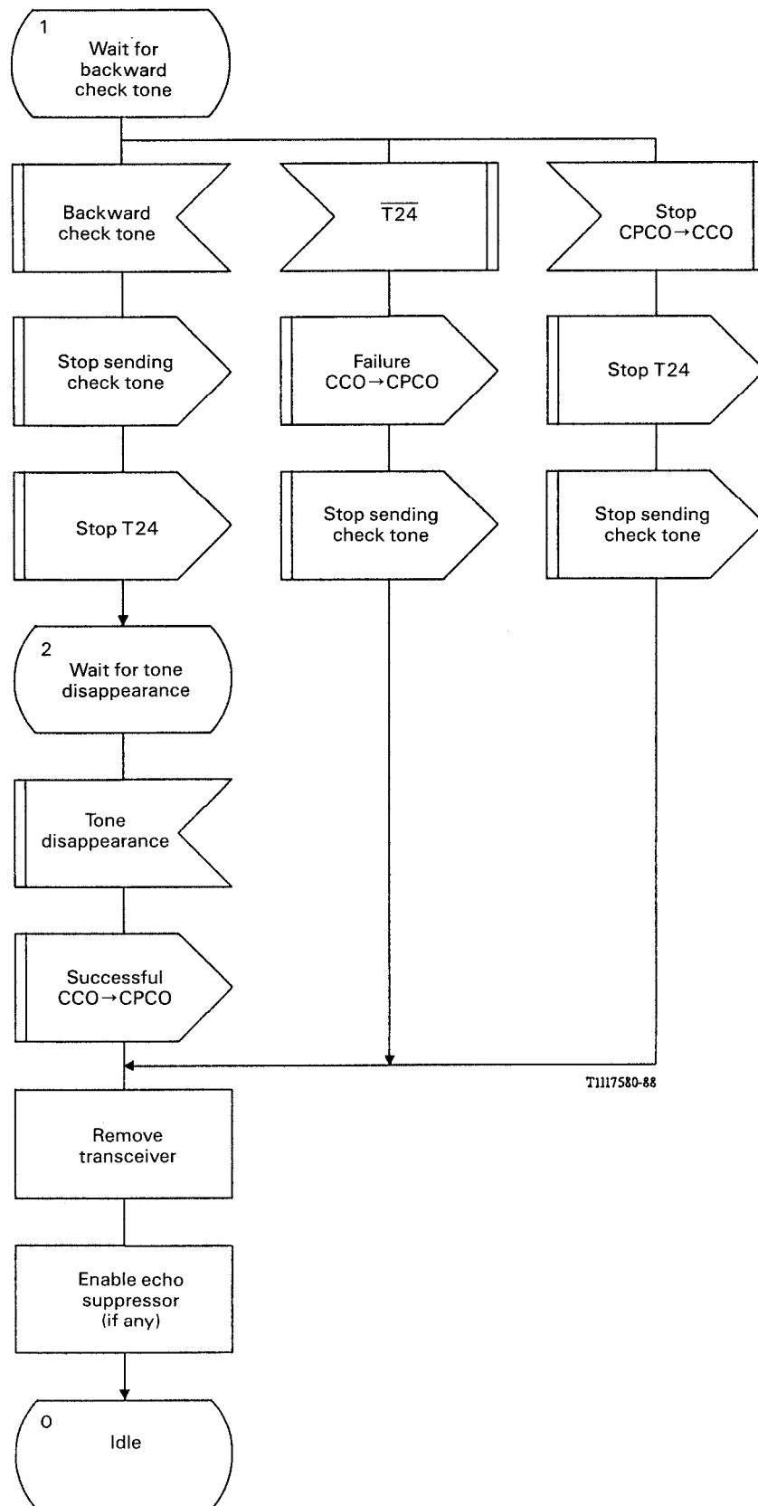
FIGURE B-24/Q.764 (Sheet 2 of 2) Continuity Check Outgoing (CCO)
