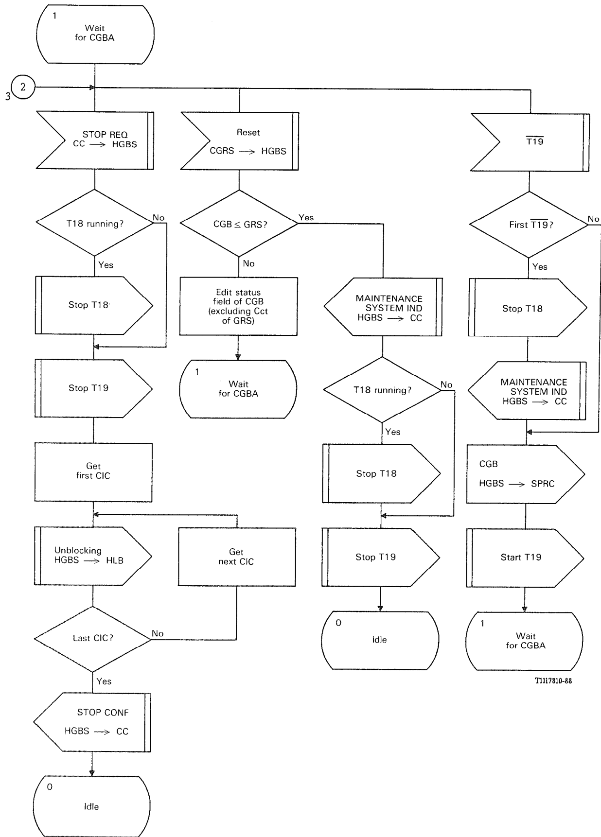
FIGURE B-31/Q.764 (Sheet 4 of 6)
