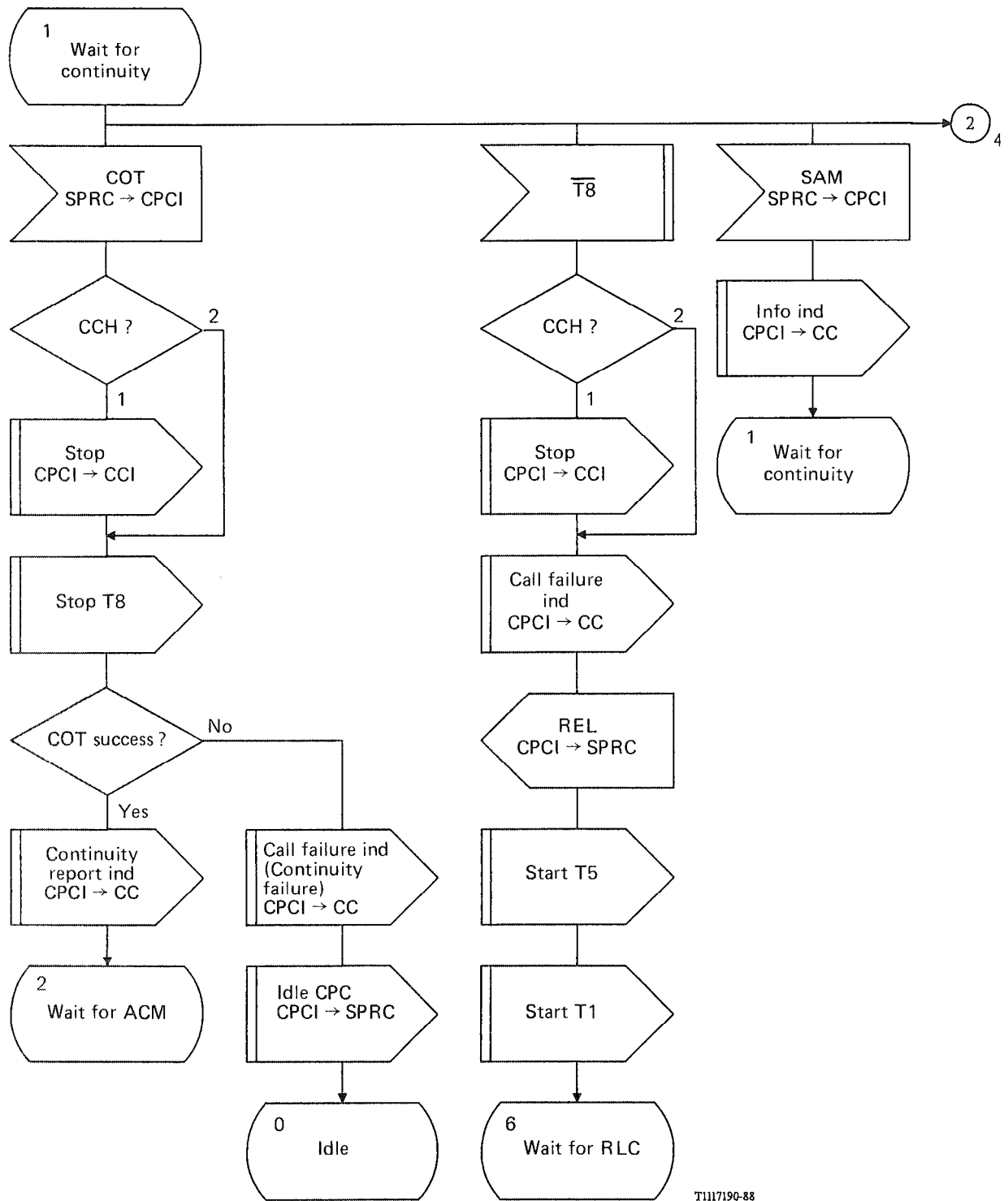
FIGURE B-21/Q.764 (sheet 3 of 18) Call processing control incoming (CPCI)
