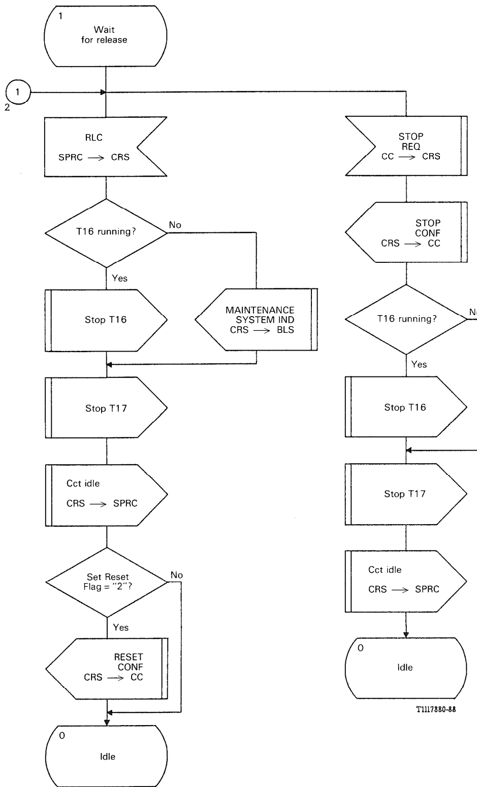
FIGURE B-33/Q.764 (Sheet 3 of 3)
