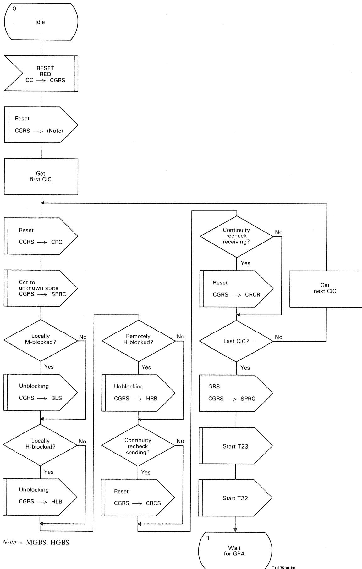
FIGURE B-35/Q.764 (Sheet 1 of 3) Circuit Group Reset Sending (CGRS)
