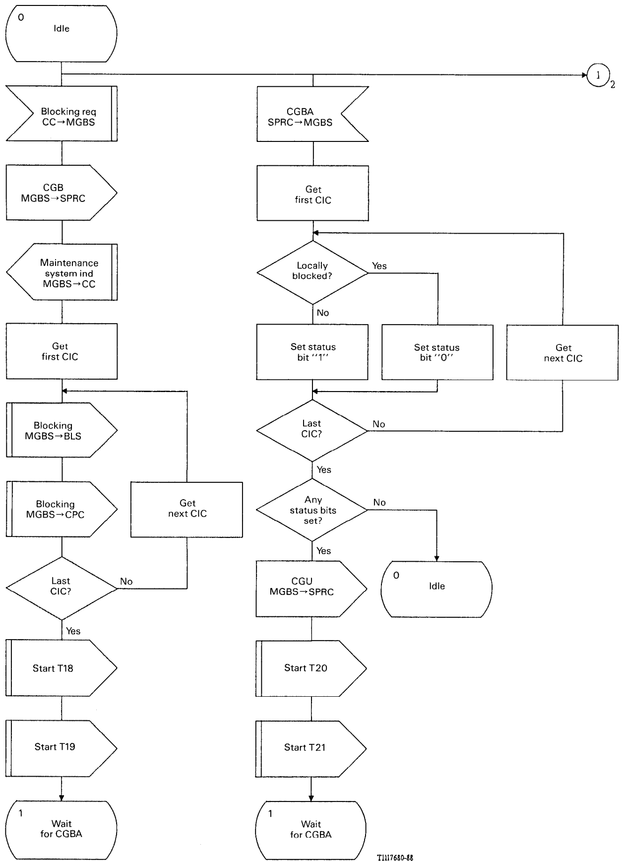
FIGURE B-27/Q.764 (Sheet 1 of 6)
