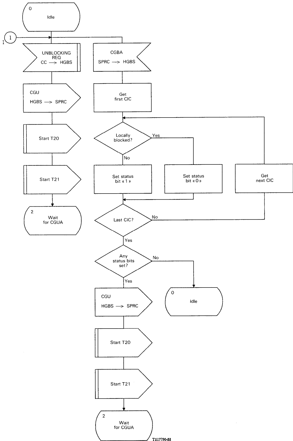
FIGURE B-31/Q.764 (Sheet 2 of 6)
