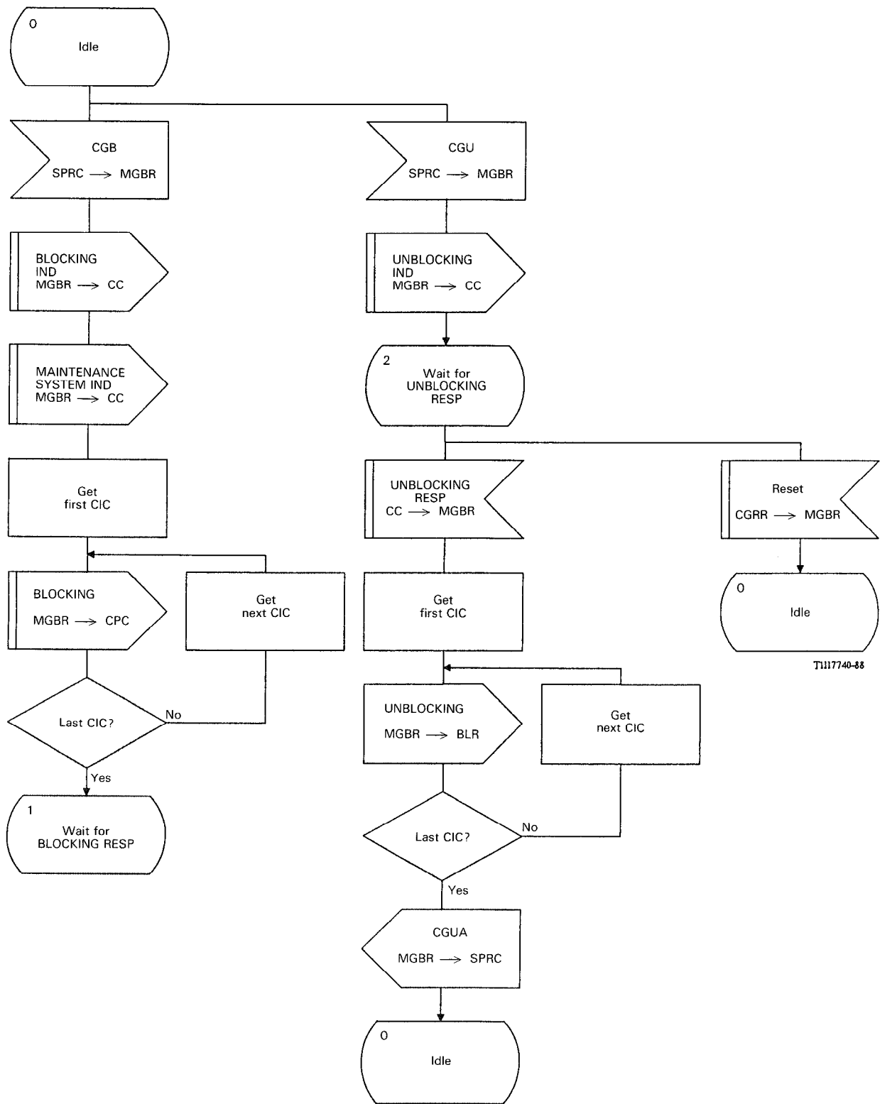
FIGURE B-28/Q.764 (Sheet 1 of 2)
