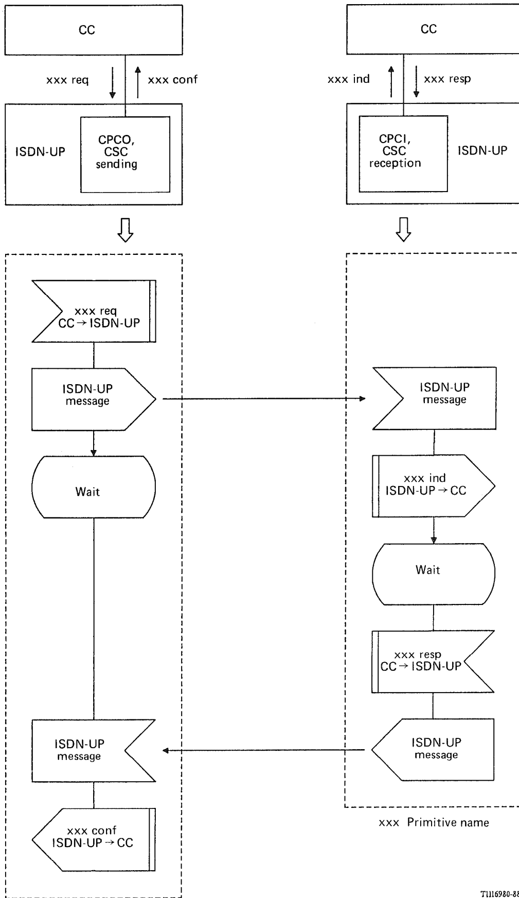
FIGURE B-3/Q.764 SDL convention example
