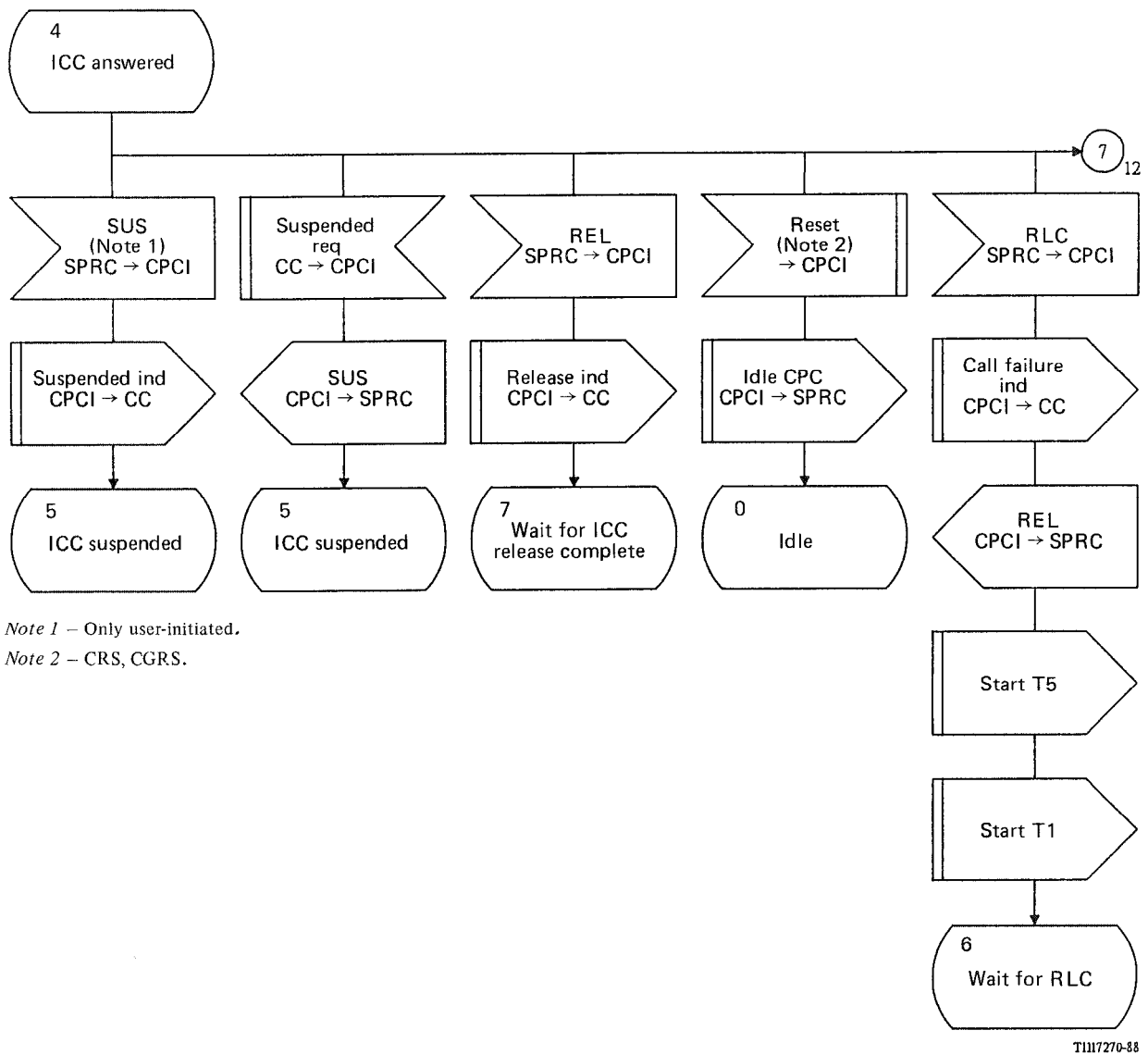
FIGURE B-21/Q.764 (sheet 11 of 18) Call processing control incoming (CPCI)
