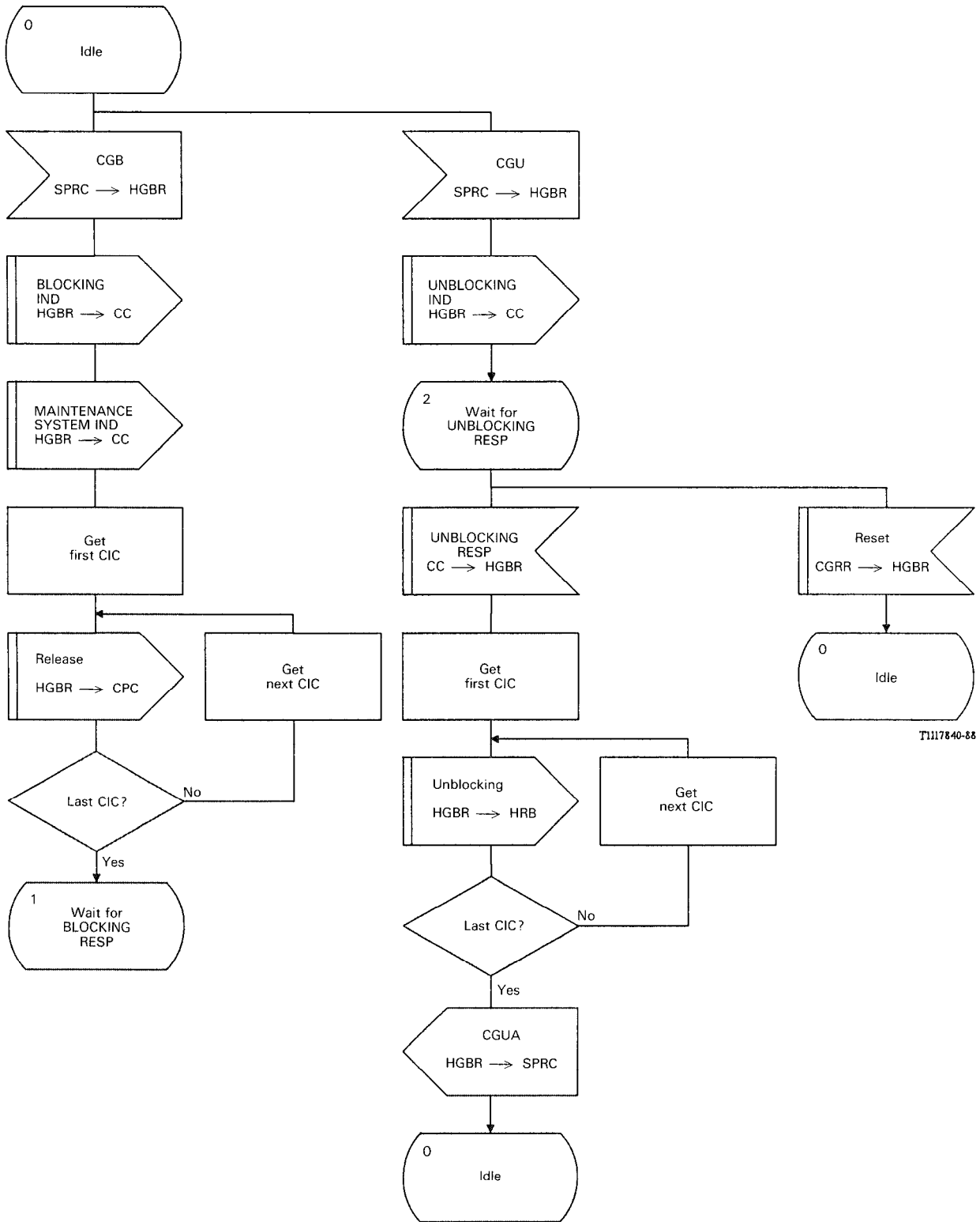
FIGURE B-32/Q.764 (Sheet 1 of 2)
