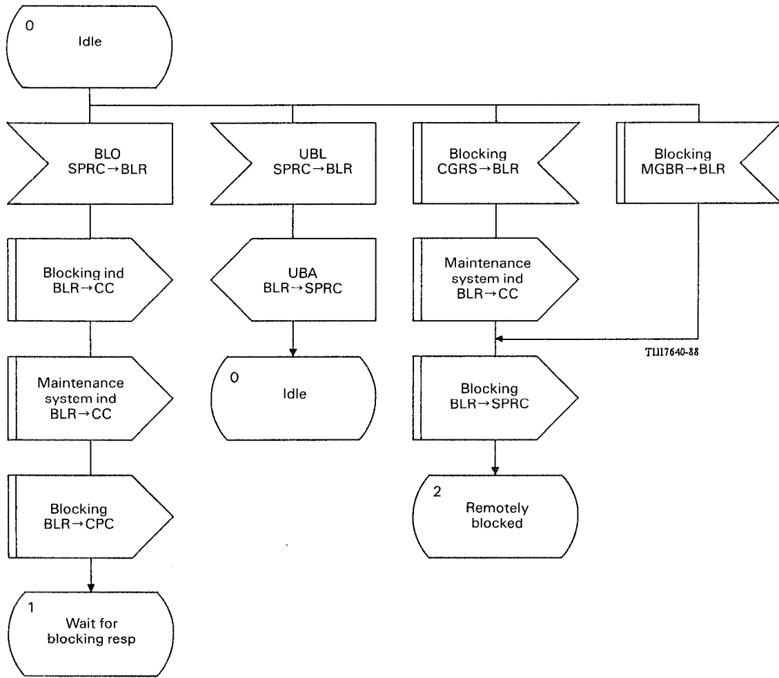
FIGURE B-26/Q.764 (Sheet 1 of 4) Blocking/Unblocking Message Reception (BLR)
