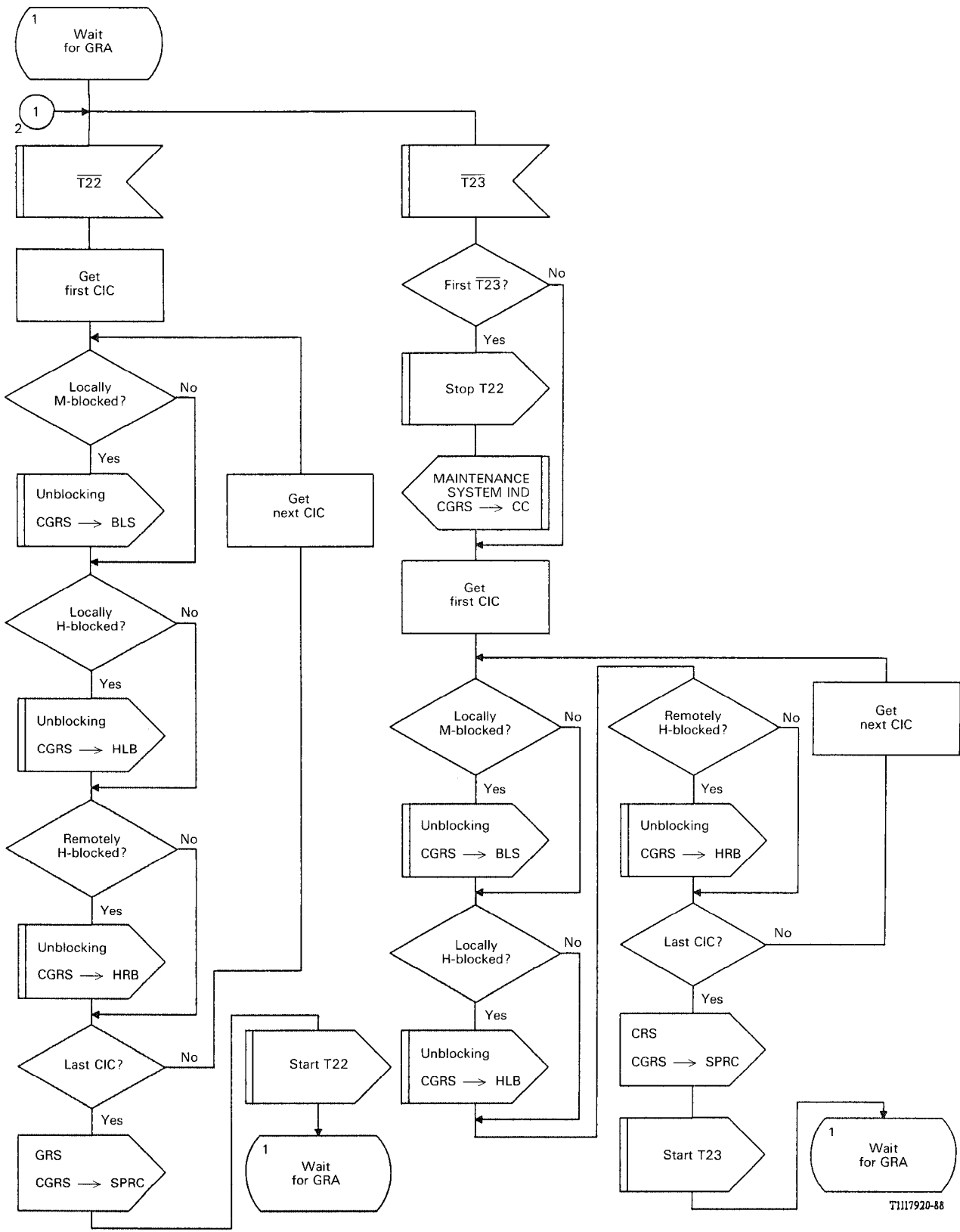
FIGURE B-35/Q.764 (Sheet 3 of 3)
