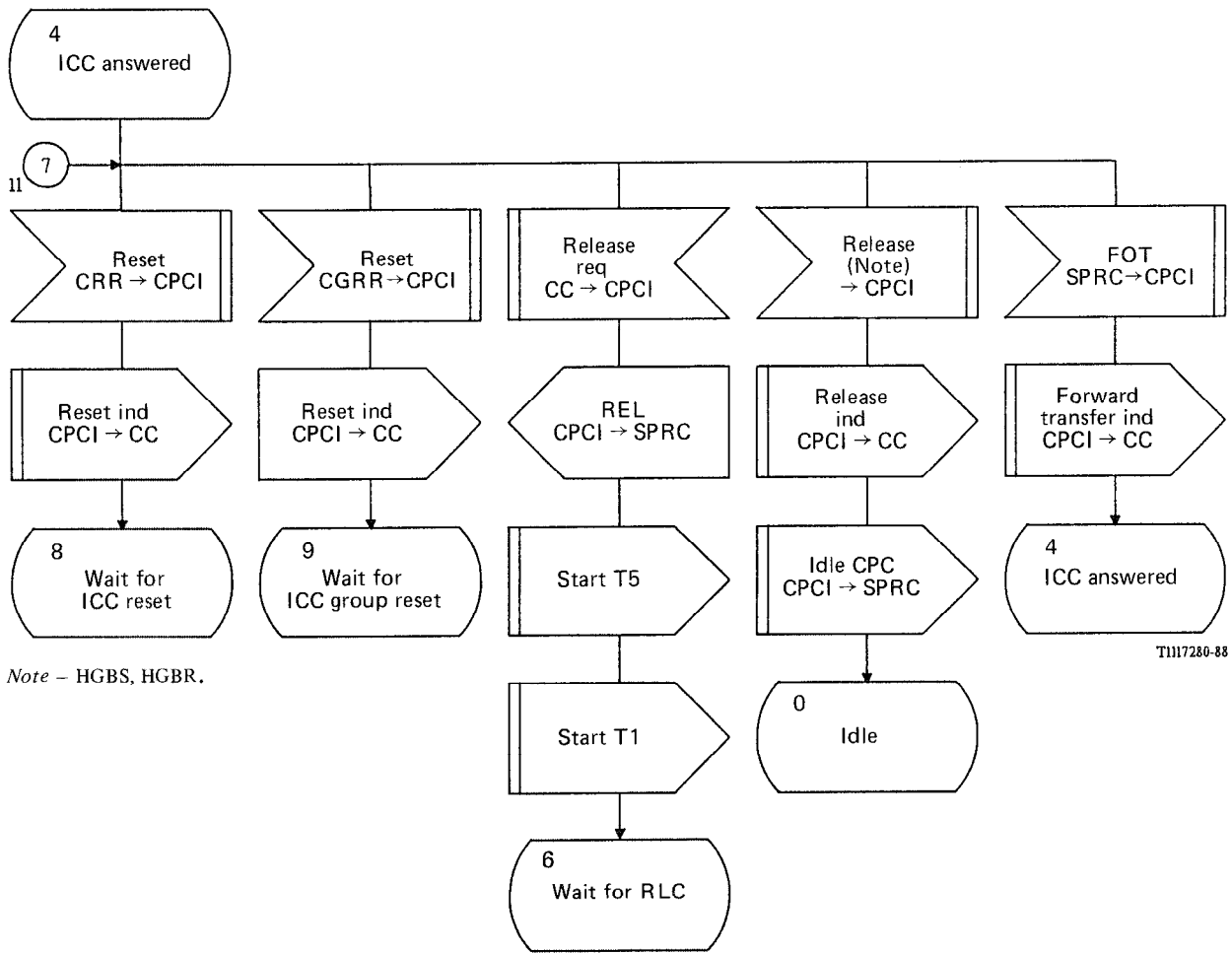
FIGURE B-21/Q.764 (sheet 12 of 18) Call processing control incoming (CPCI)
