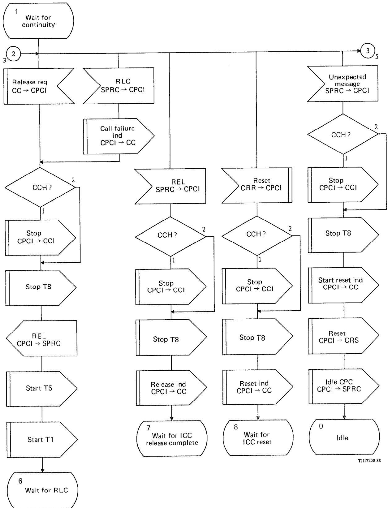
FIGURE B-21/Q.764 (sheet 4 of 18) Call processing control incoming (CPCI)
