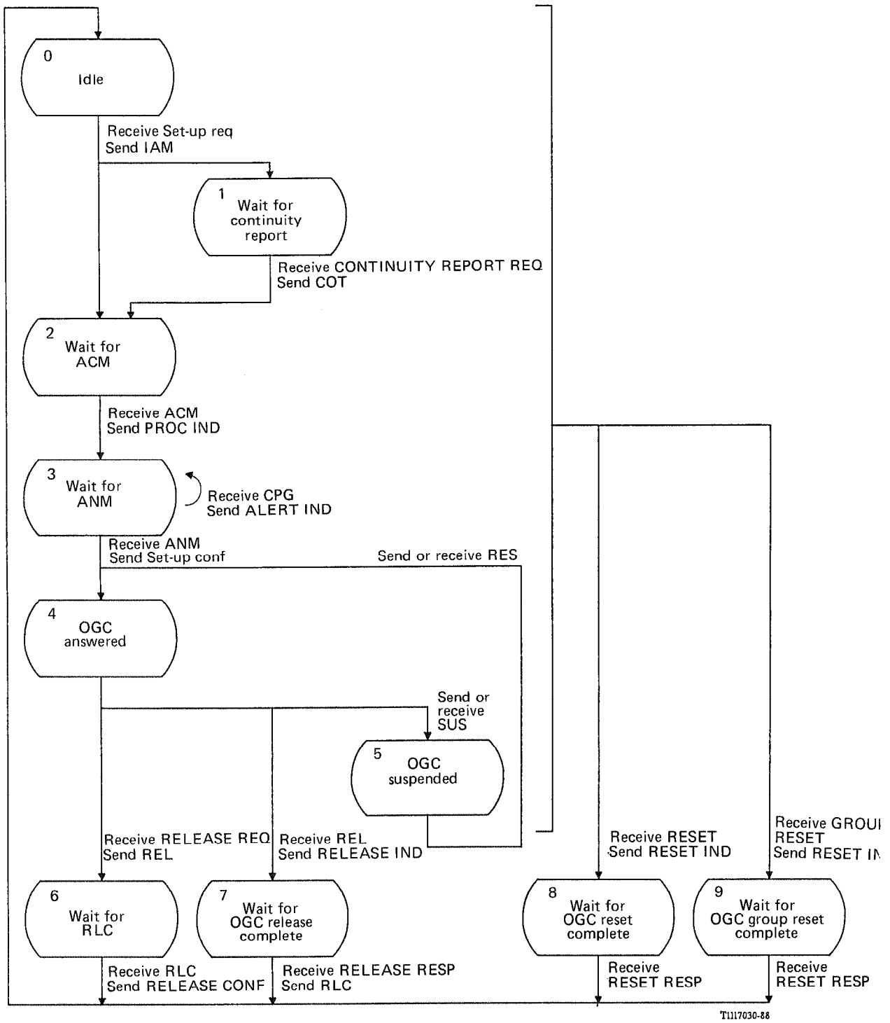
FIGURE B-8/Q.764 State transition diagrams for CPC outgoing (CPCO)
