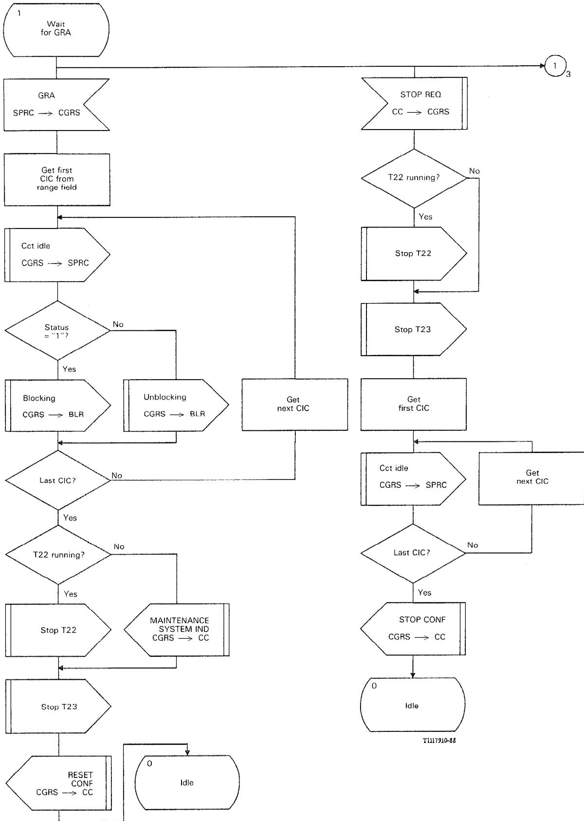
FIGURE B-35/Q.764 (Sheet 2 of 3) Circuit Group Reset Sending (CGRS)
