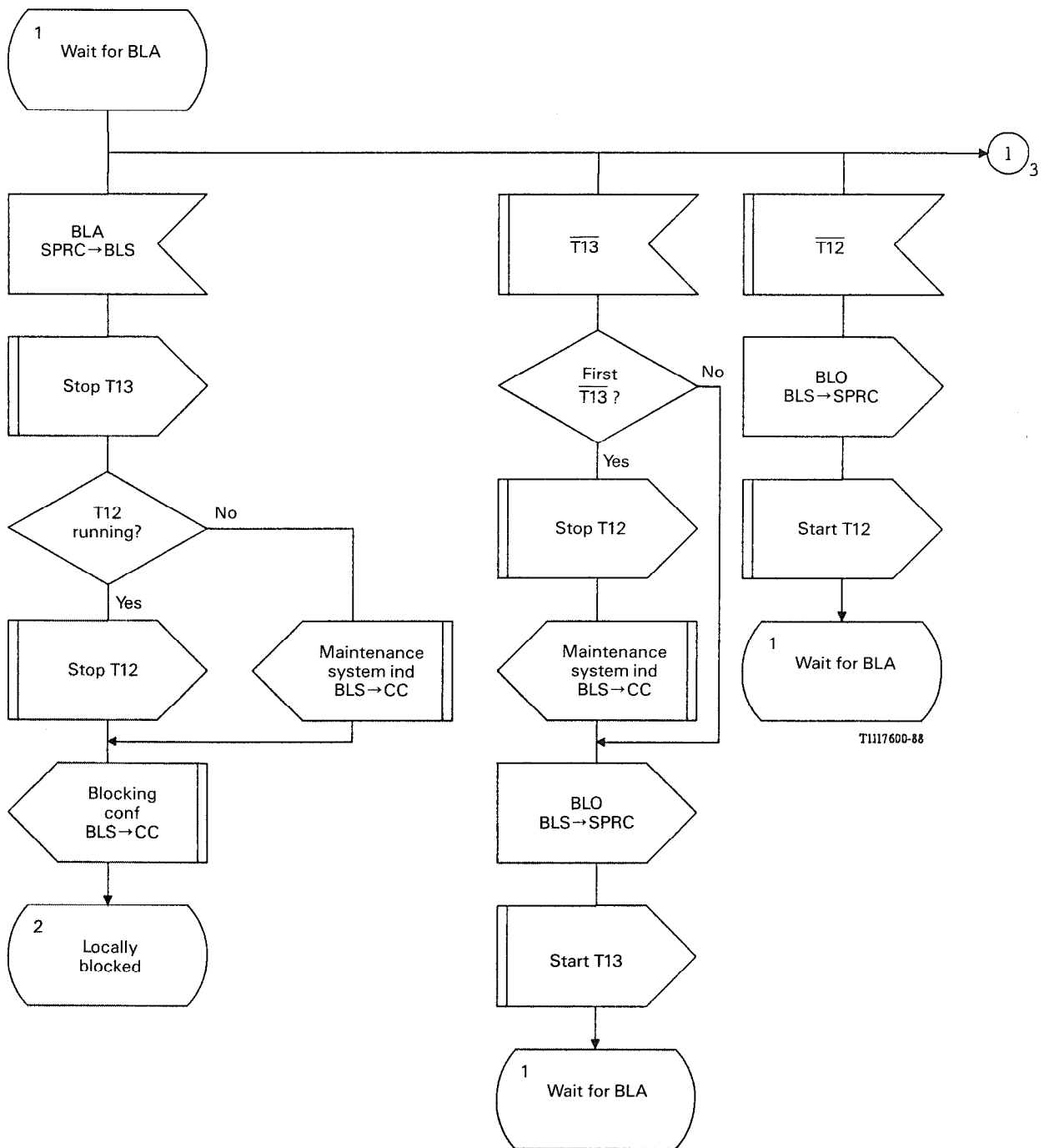
FIGURE B-25/Q.764 (Sheet 2 of 5) Blocking/Unblocking Message Sending (BLS)
