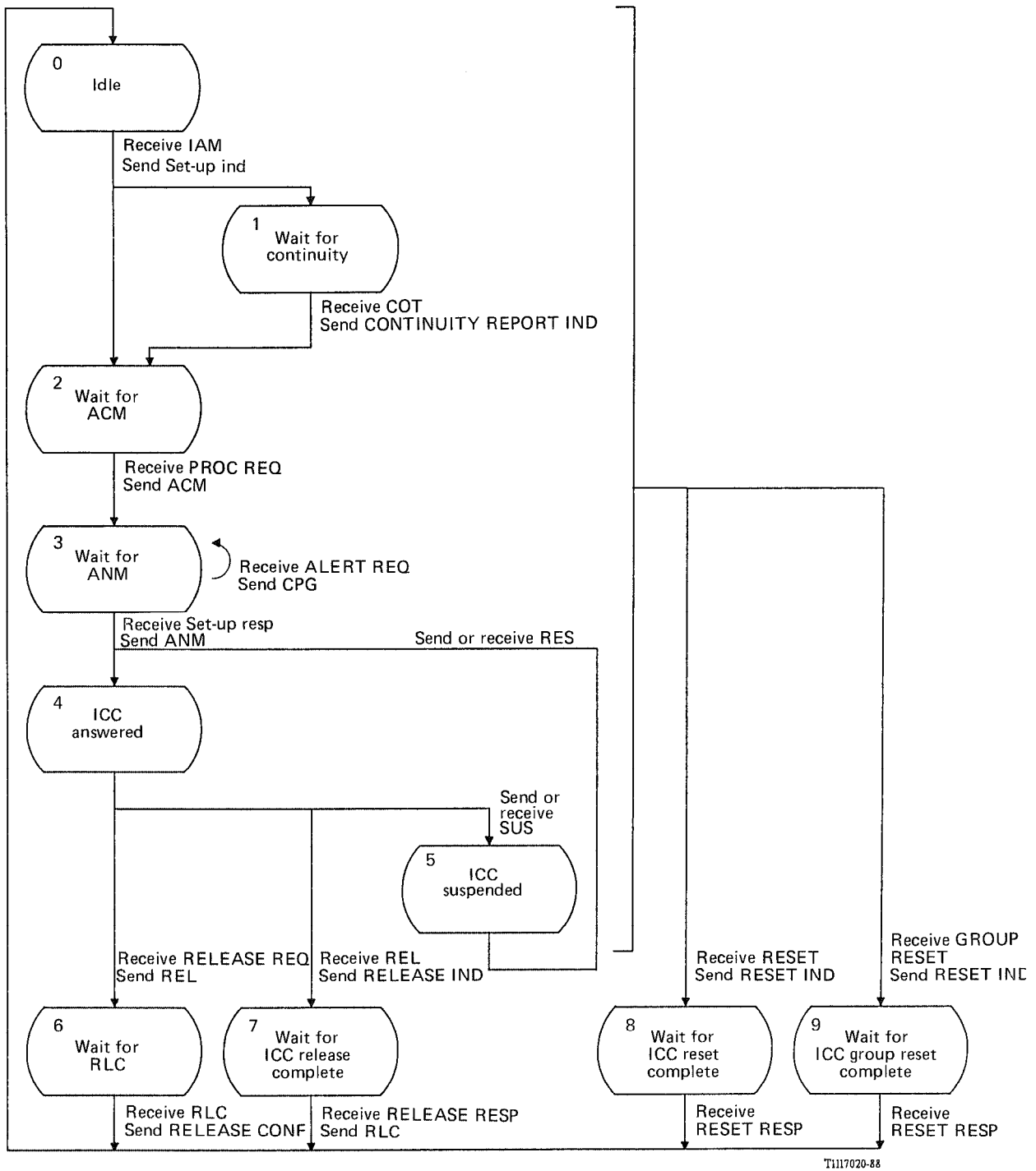
FIGURE B-7/Q.764 State transition diagrams for CPC incoming (CPCI)
