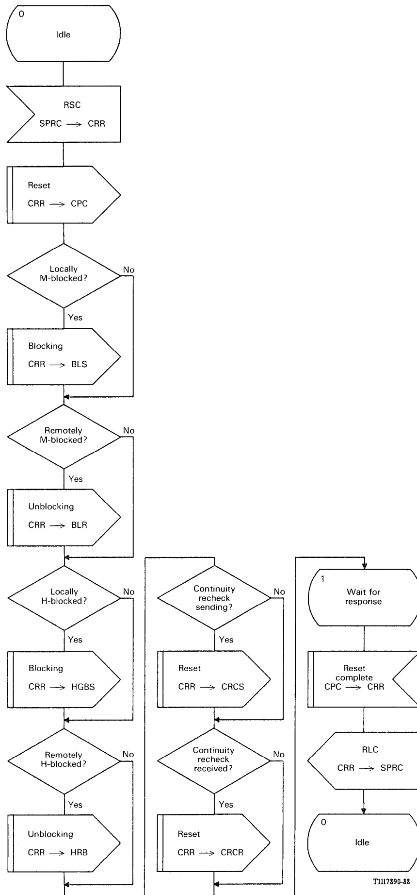
FIGURE B-34/Q.764 Circuit Reset Reception (CRR)
