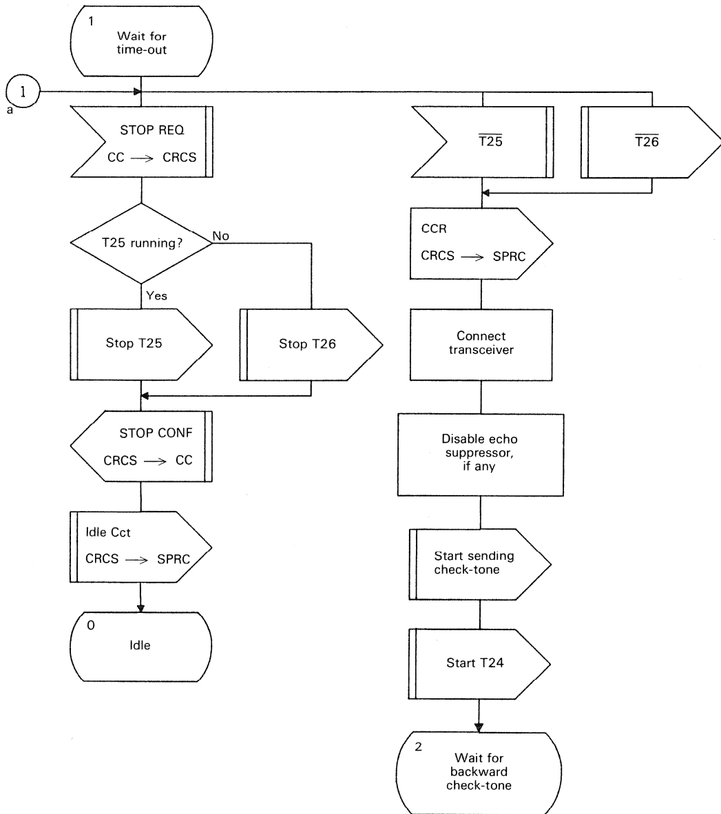
FIGURE B-37/Q.764 (Sheet 3 of 6)
