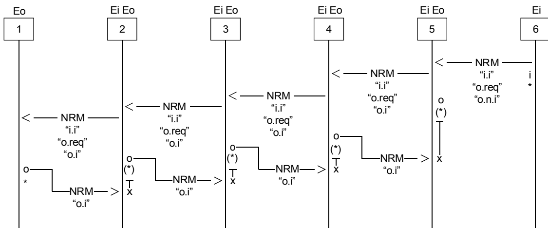
FIGURE C.9/Q.764
