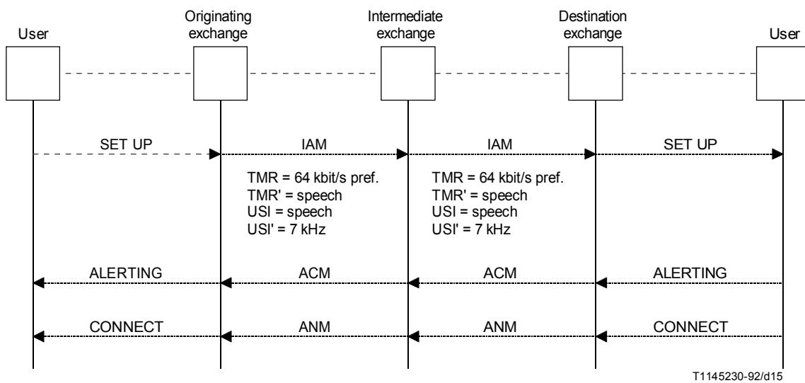
FIGURE D.1/Q.764
