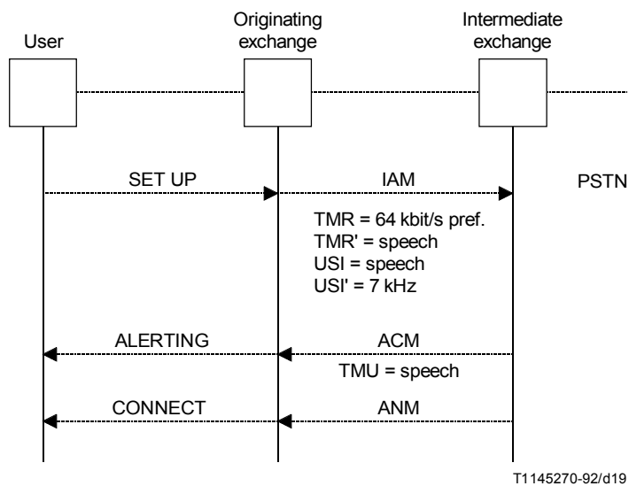
FIGURE D.5/Q.764 Fallback when interworking with PSTN
