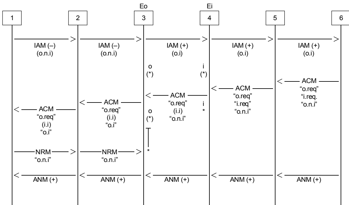
FIGURE C.3/Q.764
