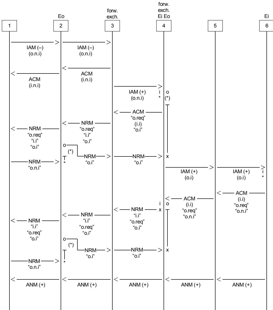
FIGURE C.2/Q.764
