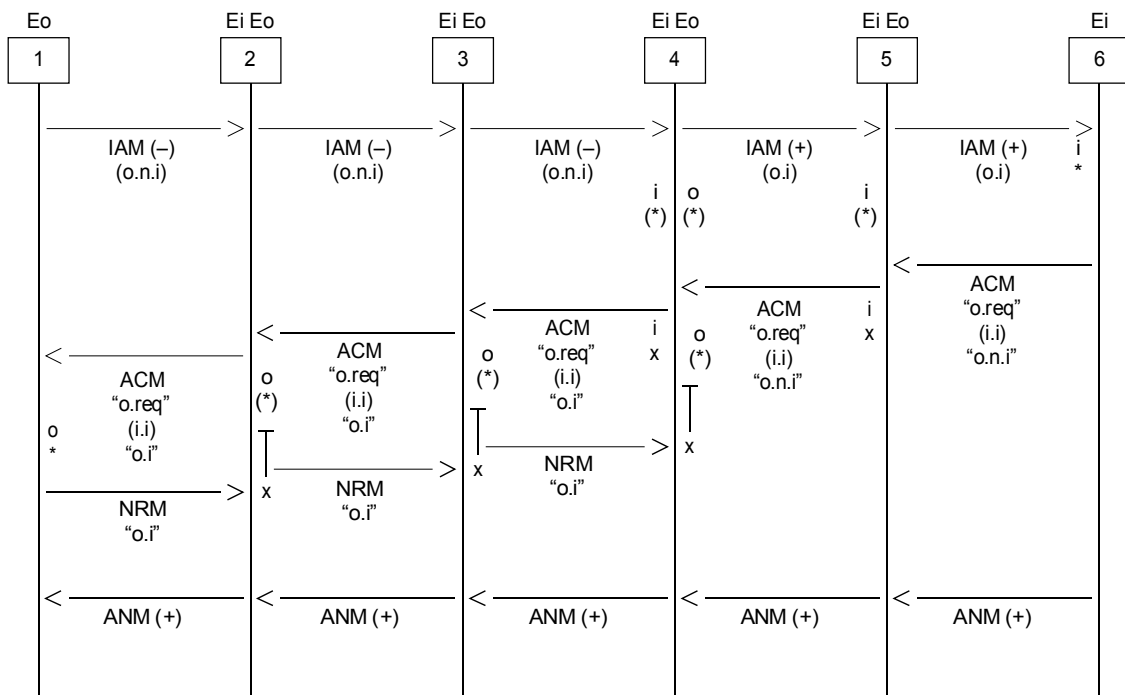
FIGURE C.1/Q.764
