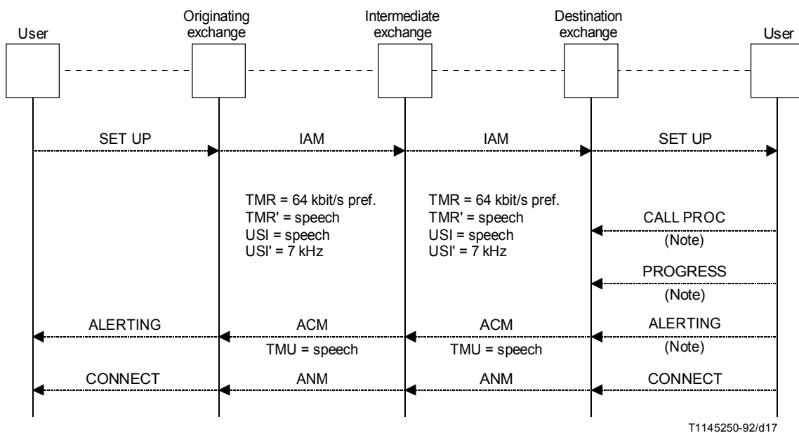
FIGURE D.3/Q.764 Fallback occurs to speech at the destination interface. Fallback indicated in alerting or any message before alerting
