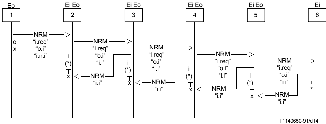
FIGURE C.10/Q.764
