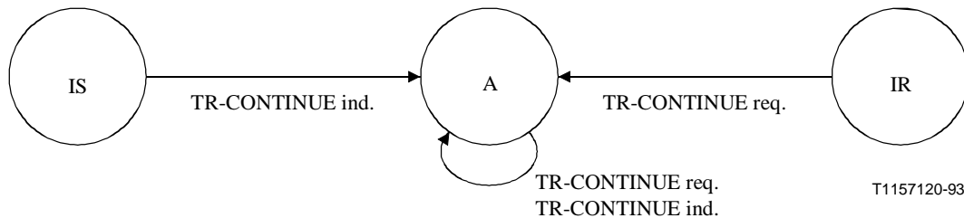
Figure 7/Q.771 – State transitions for transaction continuation
